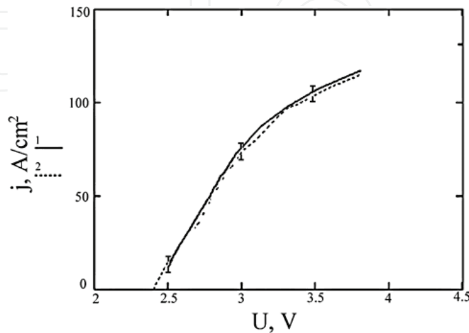
Figure 15. I-V LED: simulation (1) and experiment (2).
