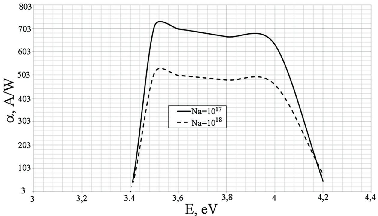
Figure 24. Phototransistor sensitivity vs. quanta energy E at P = 10^{-3} \text{ W/cm}^2 and U = 9 \text{ V} .
