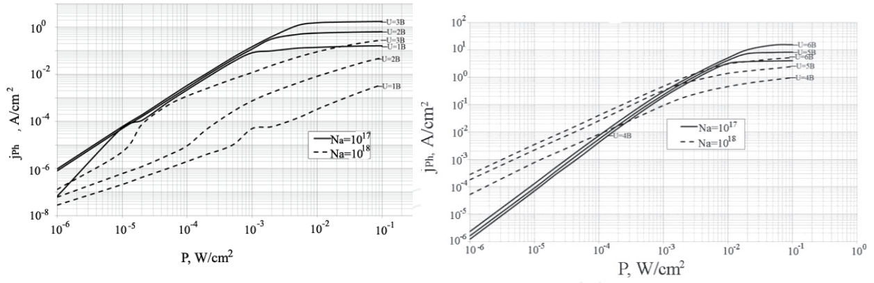
Figure 20. Photocurrent density J_{ph} vs. irradiation power P at U = 1-6 V.
