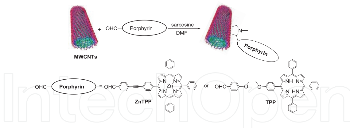
Scheme 5. Preparation of MWCNT-ZnTPP and MWCNT-TPP hybrid materials through a 1,3-dipolar cycloaddition reaction [43].
