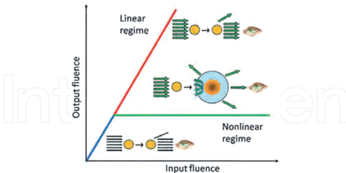
Figure 2. Trend of the light intensity (output fluence) transmitted by an ideal optical limiter versus the incoming light intensity (input fluence) [9].
