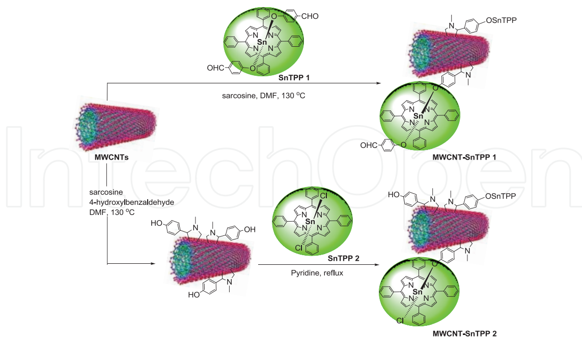
Scheme 6. Preparation of MWCNT-SnTPP 1 and MWCNT-SnTPP 2 [44].
