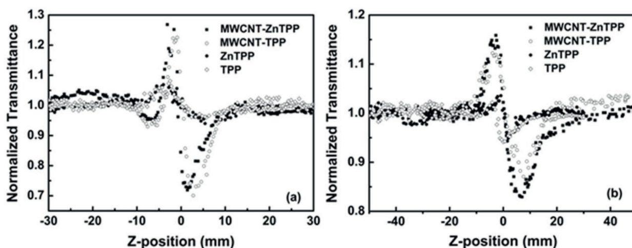
Figure 12. Normalized closed-aperture Z-scan curves of TPP, ZnTPP, MWCNT-TPP, and MWCNT-ZnTPP in N,N -dimethylformamide (DMF) with (a) 4 ns and (b) 21 ps pulse durations [43].
