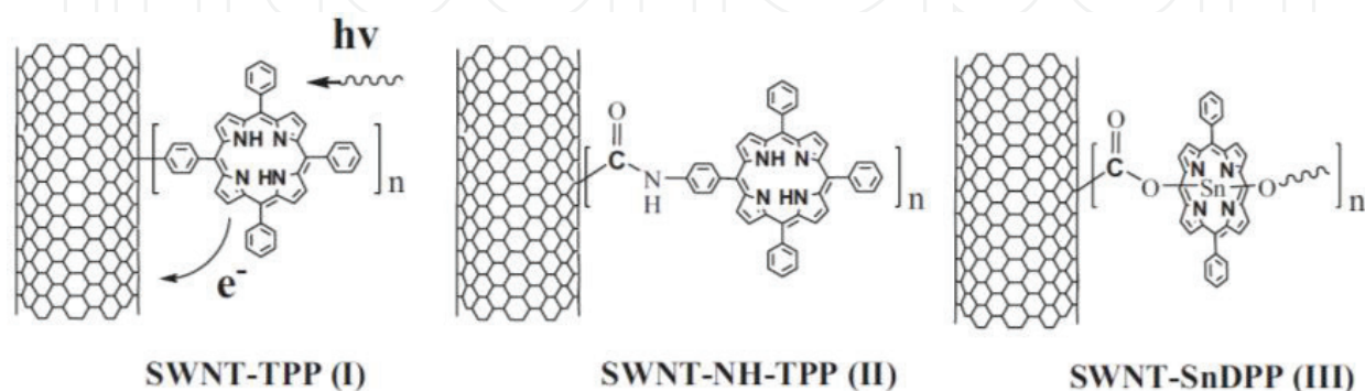
Figure 9. Structures of porphyrins covalently functionalized SWCNTs I, II, and III [40].
