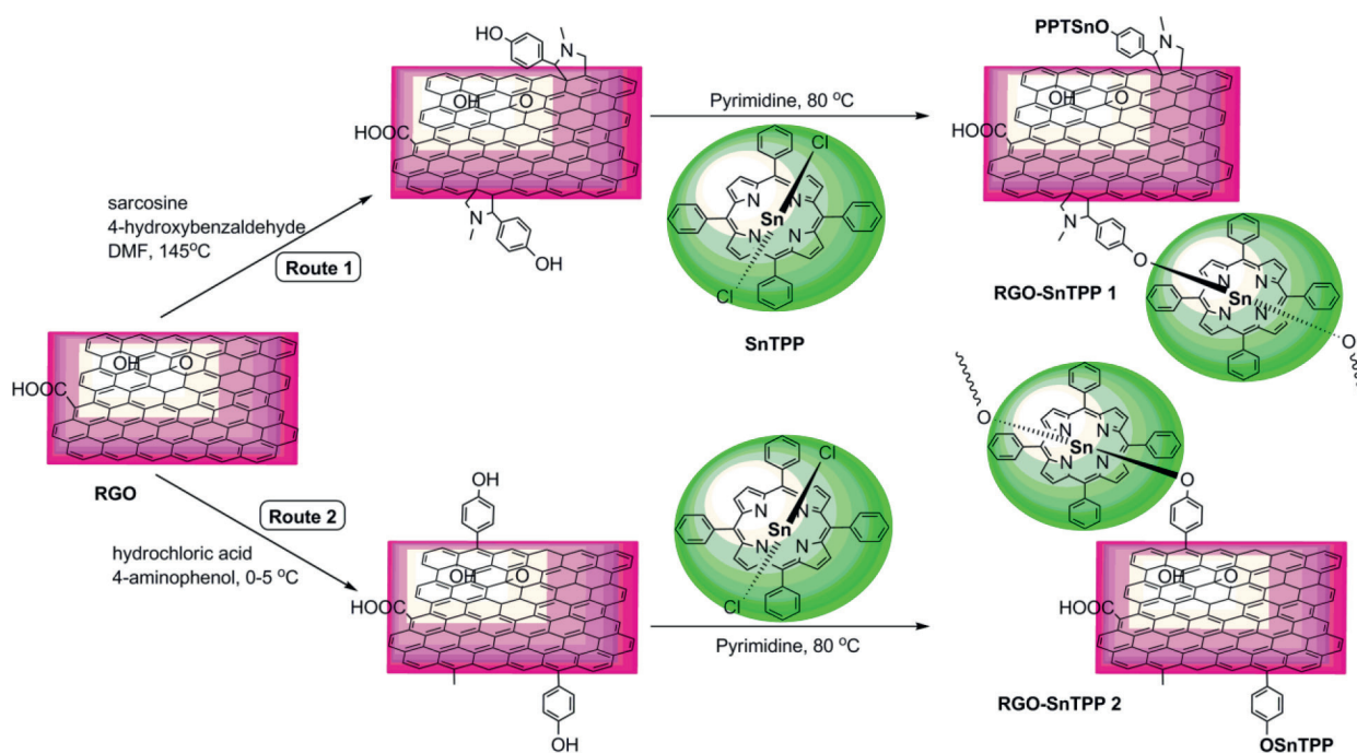
Scheme 2. Syntheses of RGO-SnTPP 1 and RGO-SnTPP 2 [30].
