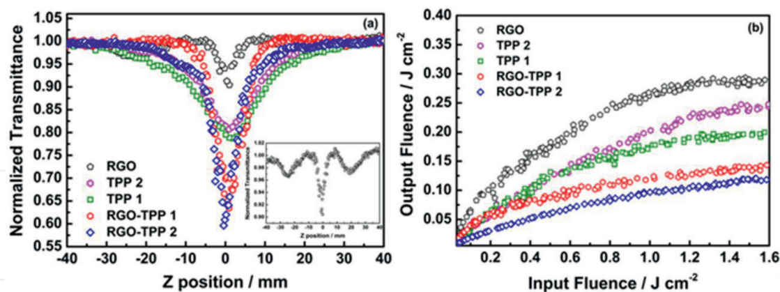
Figure 6. (a) Open-aperture Z-scan curves and (b) Optical limiting performances of RGO, TPP 2, TPP 1, RGO-TPP 1, and RGO-TPP 2 [26].
