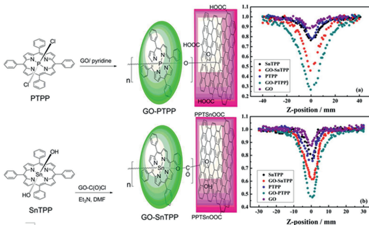
Figure 7. Synthetic routes of GO-PTPP and GO-SnTPP, and open-aperture Z-scan curves of GO, SnTPP, GO-SnTPP, PTPP, and GO-PTPP at 532 nm with (a) 4 ns and (b) 21 ps pulse duration [29].
