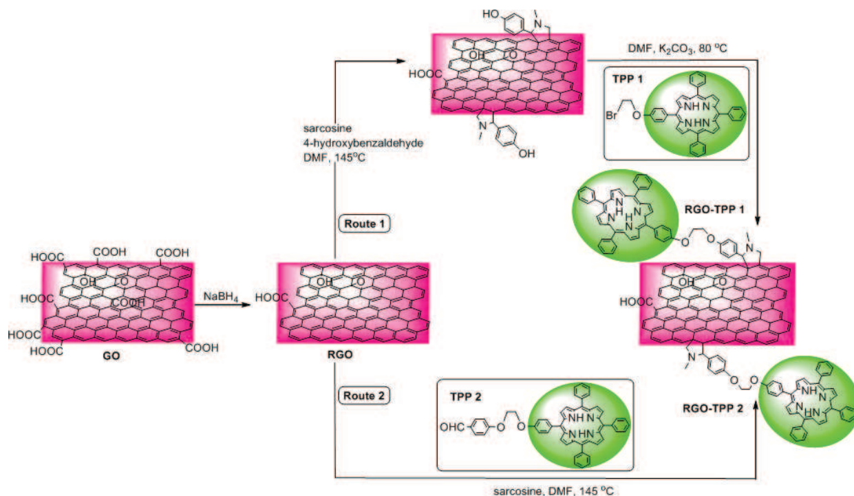
Scheme 1. Chemical routes to functionalize RGO with porphyrin molecules: preparation of RGO-TPP 1 (Route 1) and RGO-TPP 2 (Route 2) [26].
