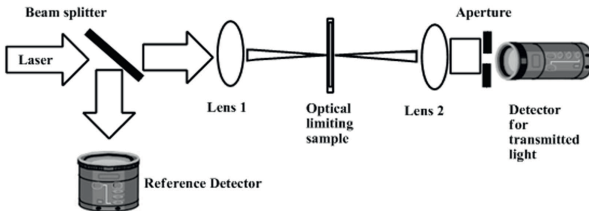
Figure 4. Experimental setup of the Z-scan technique with pulse trains, used to characterize the sample's nonlinear optical response [3].
