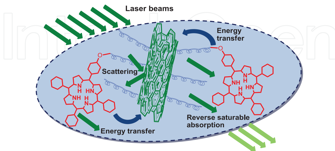
Figure 11. Possible mechanisms for the enhanced optical limiting effect of MWCNT-TPP [42].
