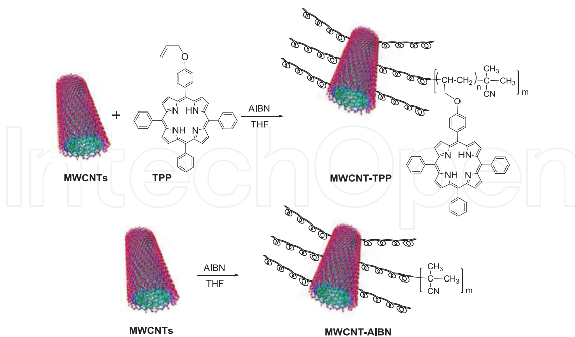
Scheme 4. Synthetic routes of MWCNT-TPP and MWCNT-AIBN [42].
