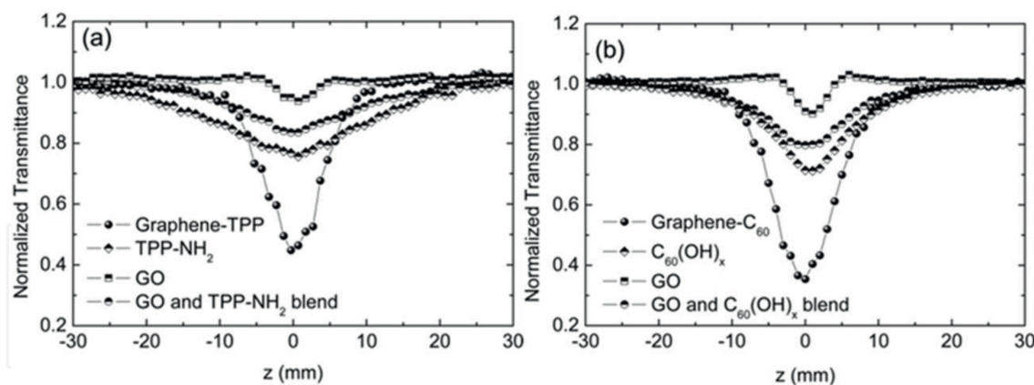
Figure 5. Open-aperture Z-scan curves of (a) Graphene-TPP, TPP-NH 2 , GO, and GO and TPP-NH 2 blend, and (b) Graphene-C 60 , C 60 (OH) x , GO, and GO and blend C 60 (OH) x [25].
