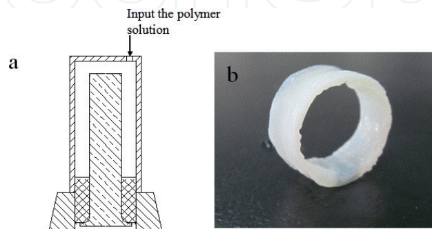
Figure 2. (a) A tubular mold; (b) overview of the tubular scaffold made from crosslinking of PLEGDMA, PEG diacrylate and NIPAAm.
