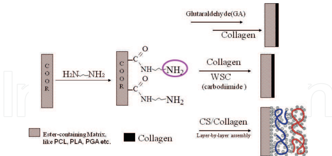
Scheme 1. Diagram of reactions between ester groups from synthesized polyesters and amino groups from diamine, aiming at introducing pendent amino groups onto substrate surface, through which many biomolecules containing amino or/and carboxylic groups can be bonded via crosslinking reagents or layer-by-layer assembly technology.
