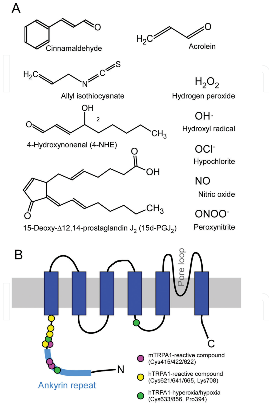
Figure 1. Chemical structure of TRPA1-activating reactive compounds (A) and reported target amino acid residues in TRPA1 (B).
