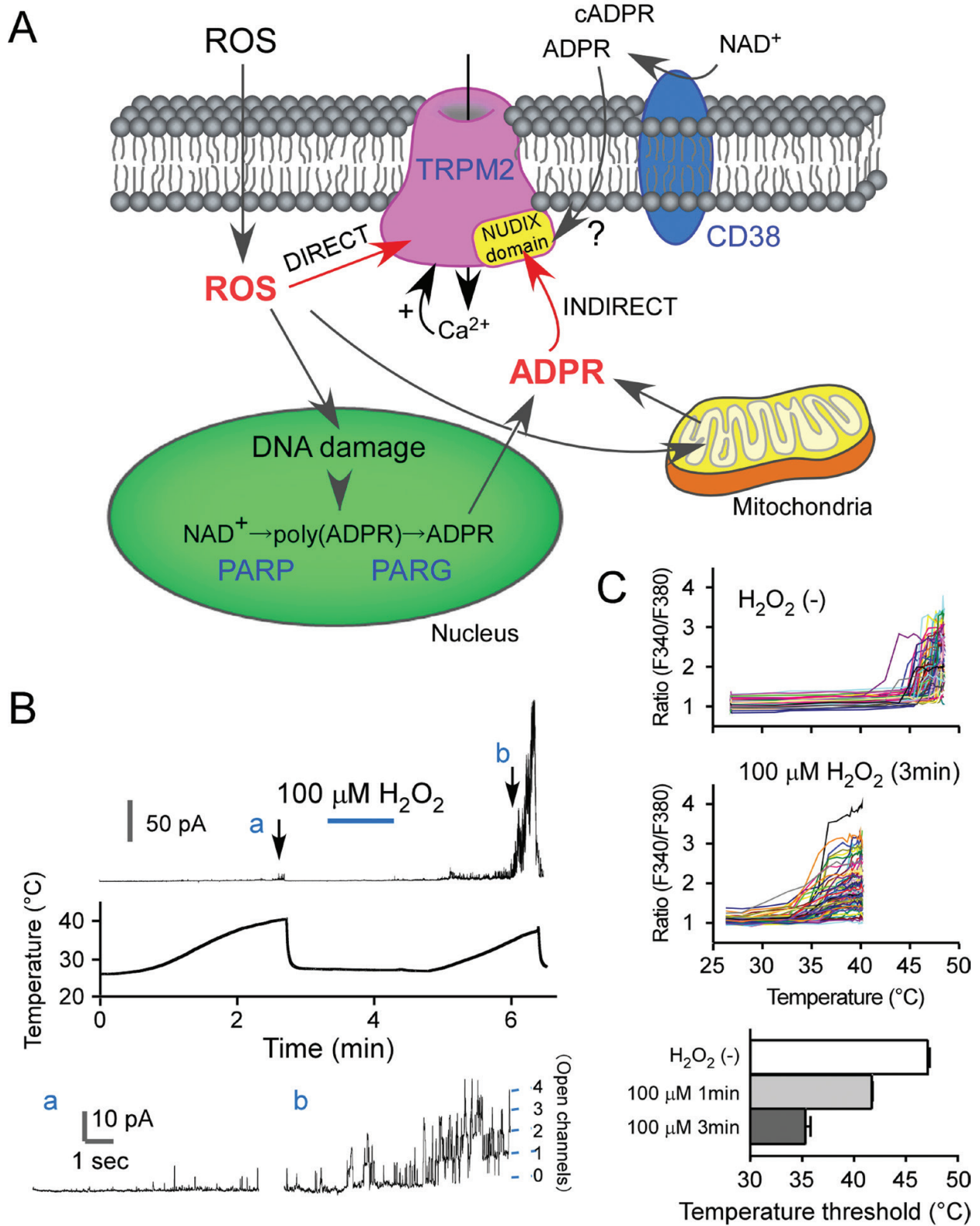
Figure 2. (A) Scheme showing the activation cascade of TRPM2 by reactive oxygen species (ROS). (B) H 2 O 2 -enhanced heat-evoked single channel opening observed in inside-out single channel recordings. (a,b) Magnified traces at the time points indicated in the upper column. (C) H 2 O 2 -treatment lowered the temperature threshold for TRPM2 activation. The temperature-fura2 ratio relationship is plotted for H 2 O 2 -untreated and H 2 O 2 -treated (100 μM, 3 min) cells. Average temperature thresholds for each group (Mean ± SEM) are shown.
