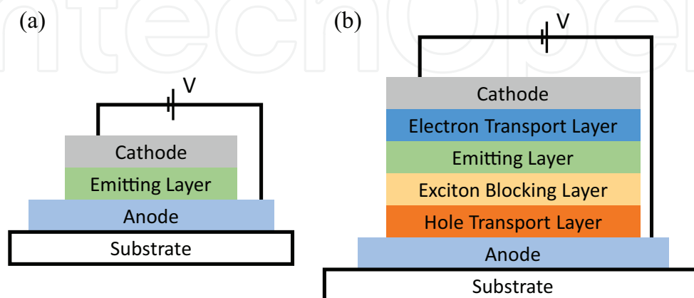
Figure 1. The structure of (a) basic and (b) typical organic light emitting diode.
