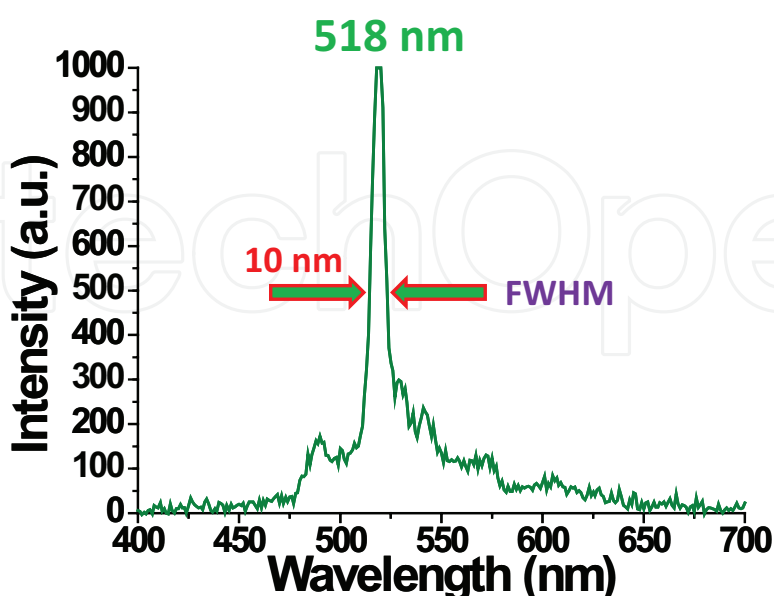
Figure 4. Emission spectrum of CdS colloidal sample.
