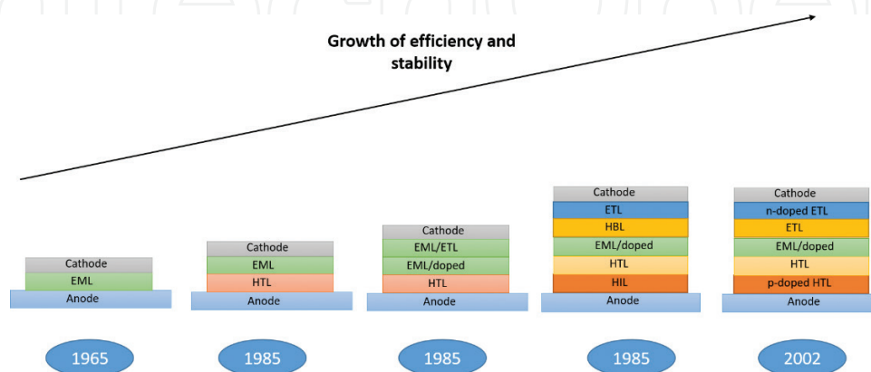
Figure 3. Evolution of OLED device structure.
