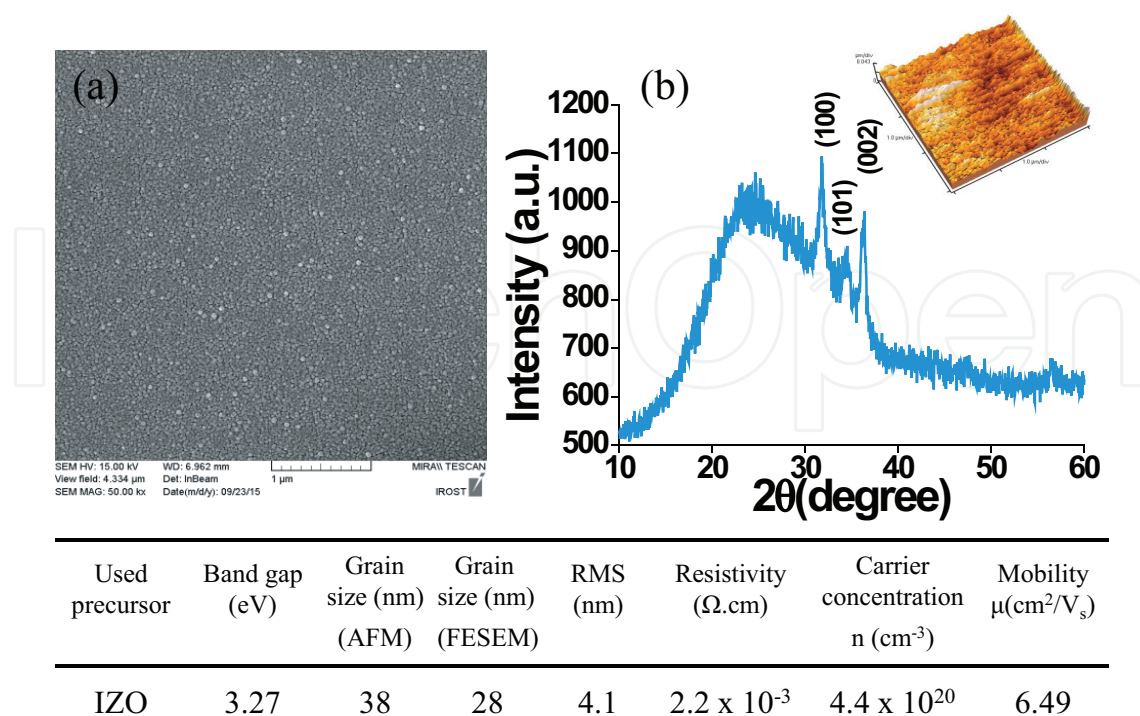
Figure 5. (a) A scanning electron microscopy (SEM) image and (b) the X-ray diffraction (XRD) pattern of QD.
