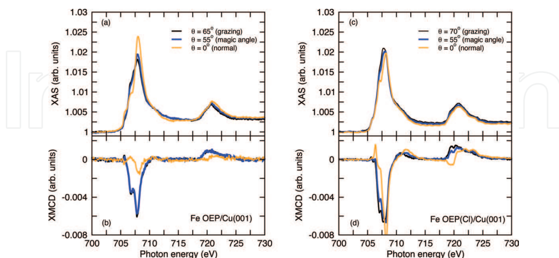
Figure 8. Measured Fe L_{2,3} edge XAS (a) and XMCD (b) for 0.4 ML Fe OEP on Cu(001). Panels (c) and (d) show the analogous results for Fe OEP (Cl)/Cu(001). The angle \theta denotes the angle between surface normal and photon beam. Taken from Ref. [13].
