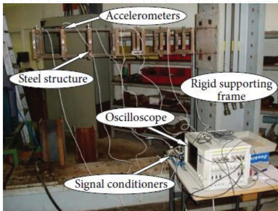
Figure 6. Test setup.
