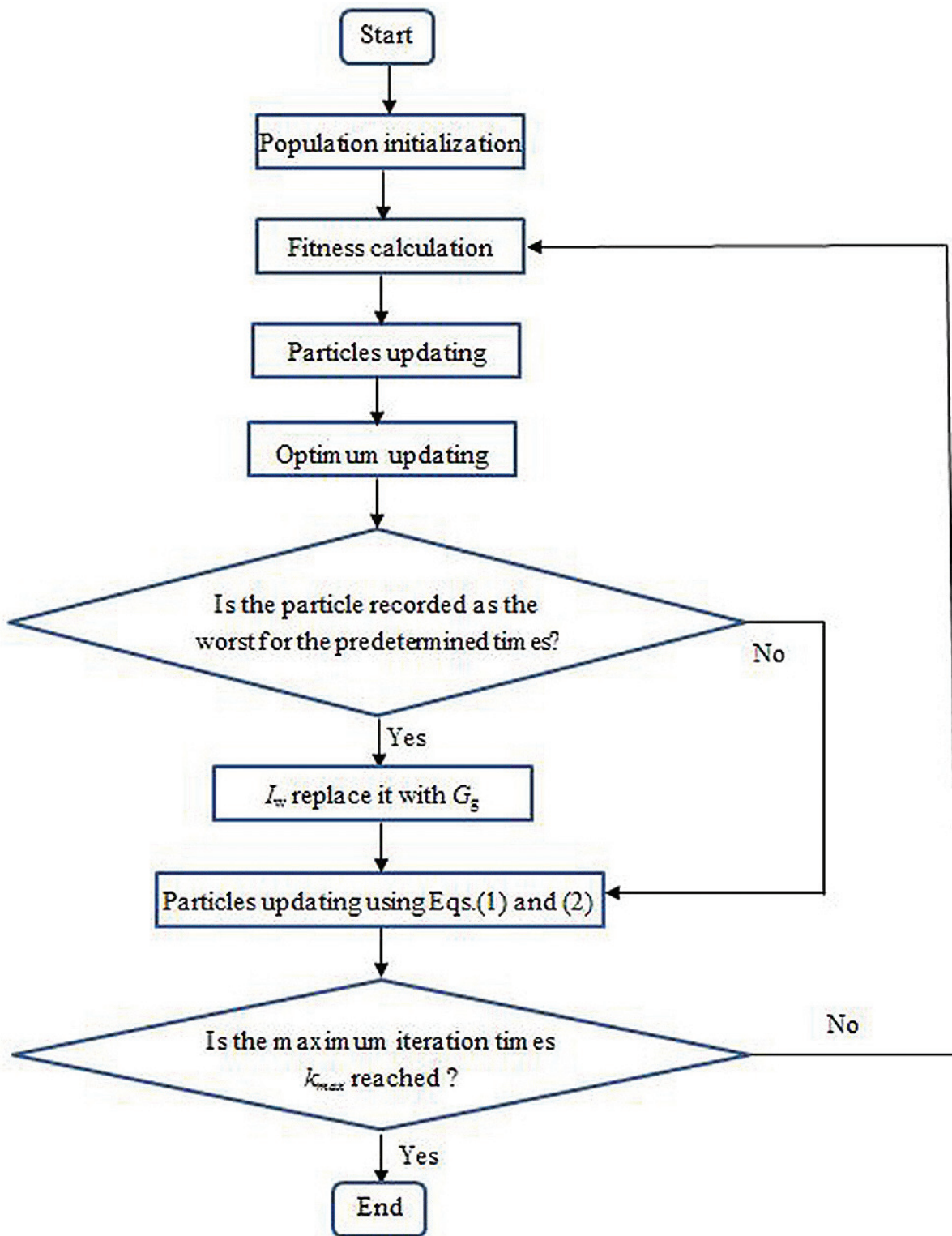
Figure 1. The flow chart of the IMPSCO algorithm.
