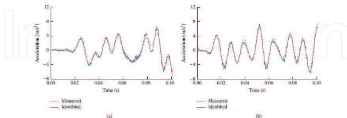
Figure 7. The comparison results of acceleration response. (a) The second floor; (b) the fifth floor.
