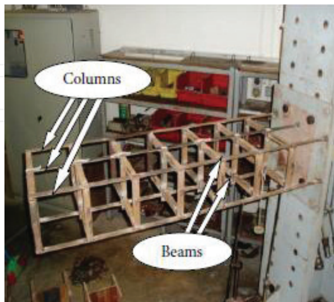
Figure 4. Seven-floor steel frame model.
