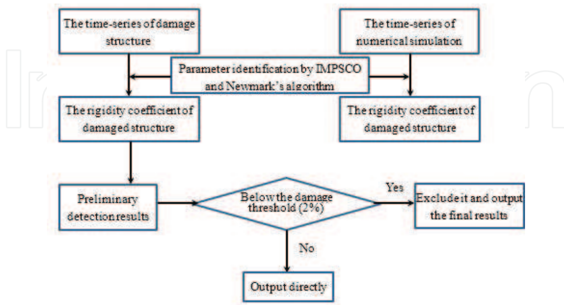
Figure 2. The schematic diagram of the damage detection strategy based on time-domain.
