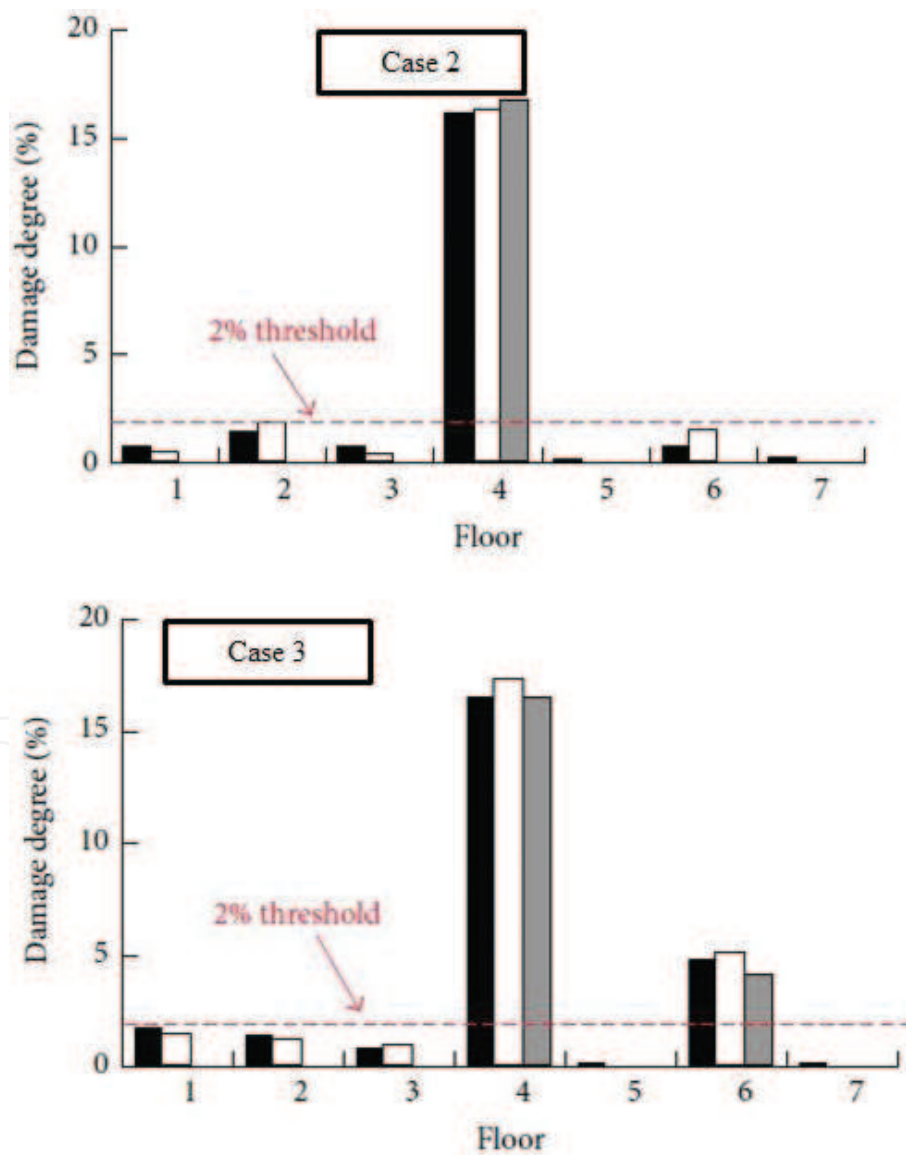
Figure 8. Identification results of all damage scenarios.
