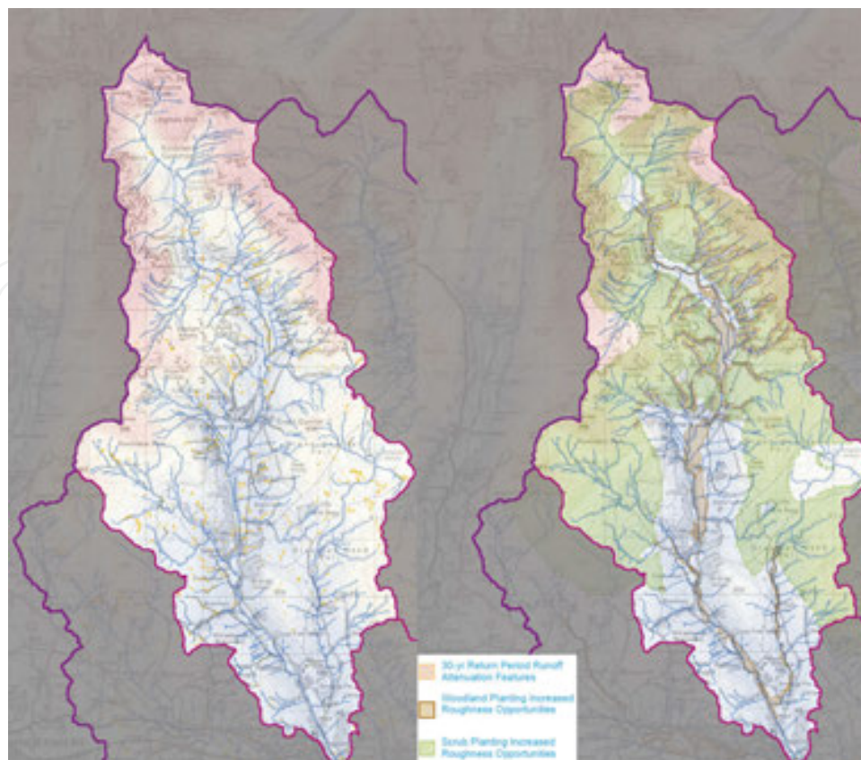
Figure 4. Runoff Attenuation Features (RAFs) and shrub and approximate woodland planting opportunities in the upper Kent (for illustration).
