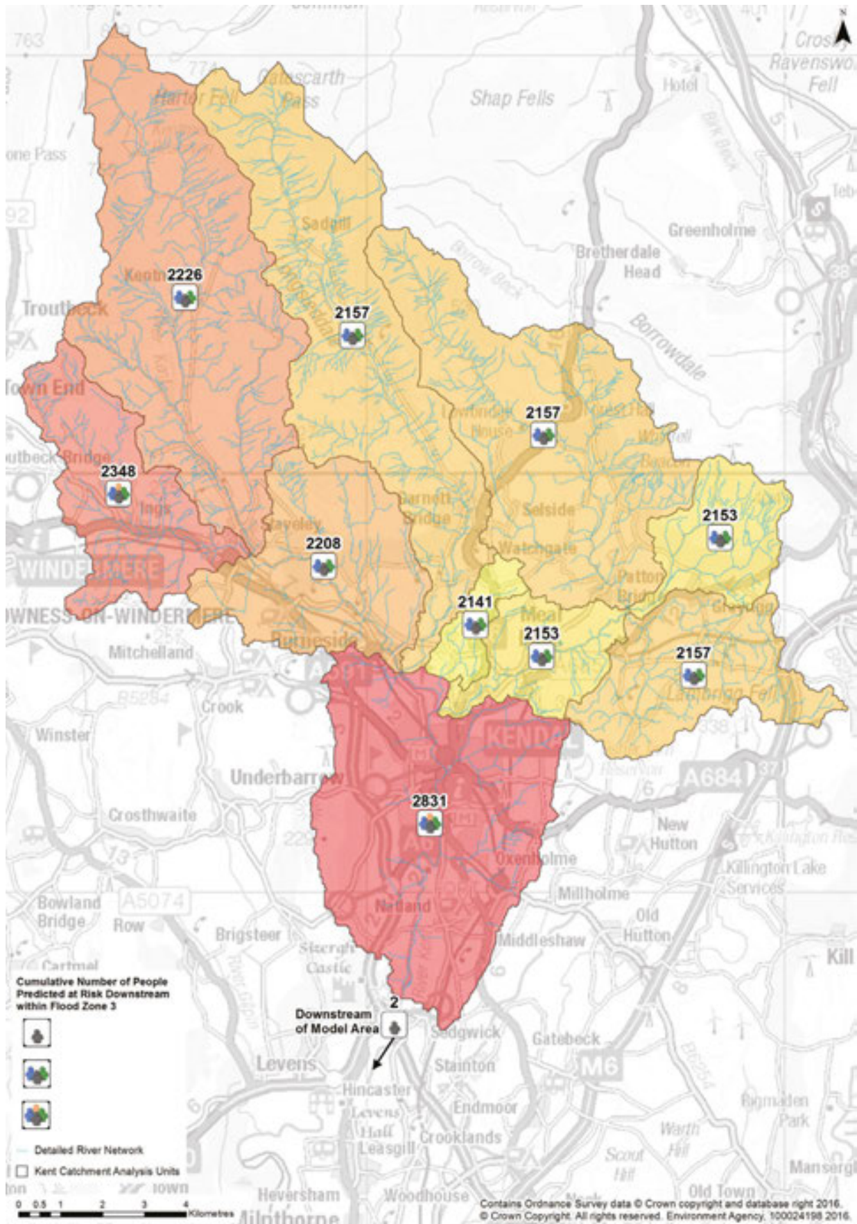
Figure 8. Downstream risk visualised for the Kent.
