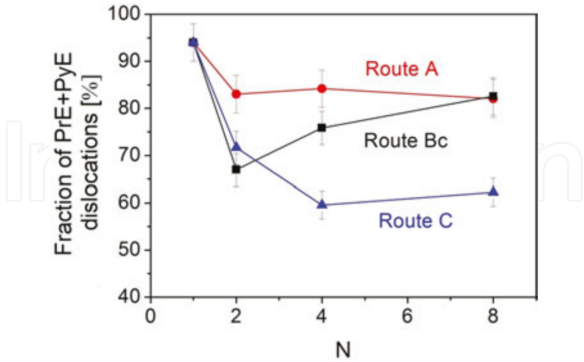
Figure 19. The dependence of the sum of relative fractions of prismatic (PrE) and pyramidal (PyE) <a>-type edge dislocations on the route of ECAP and the number of passes.
