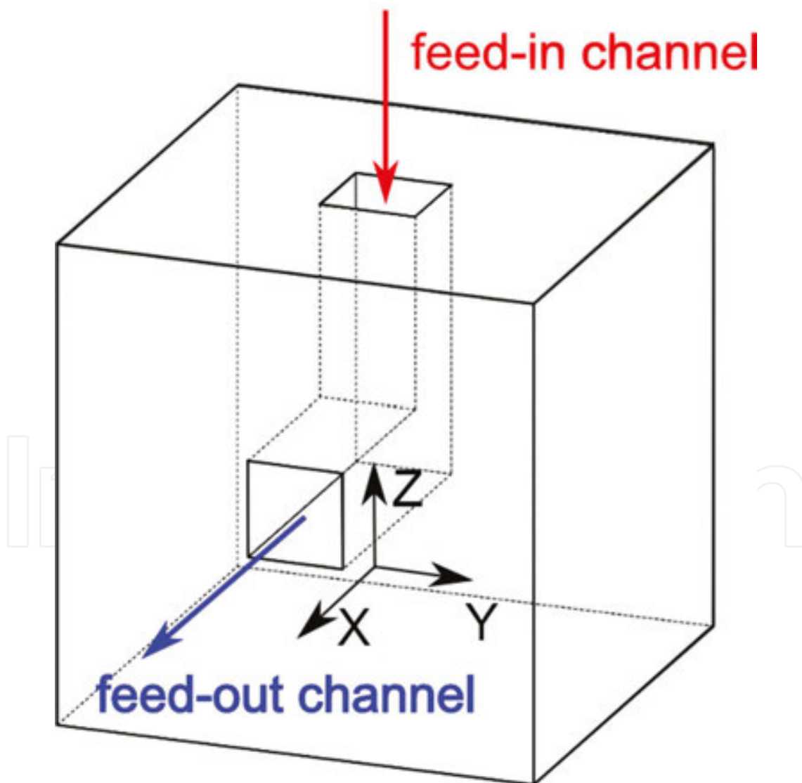
Figure 1. The scheme of the ECAP die including the coordinate system [2].
