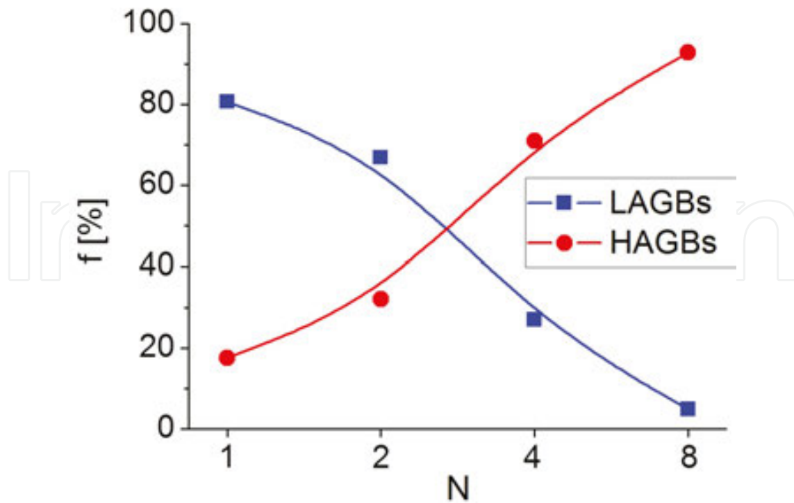
Figure 6. GB character evolution in ECAP Cu.
