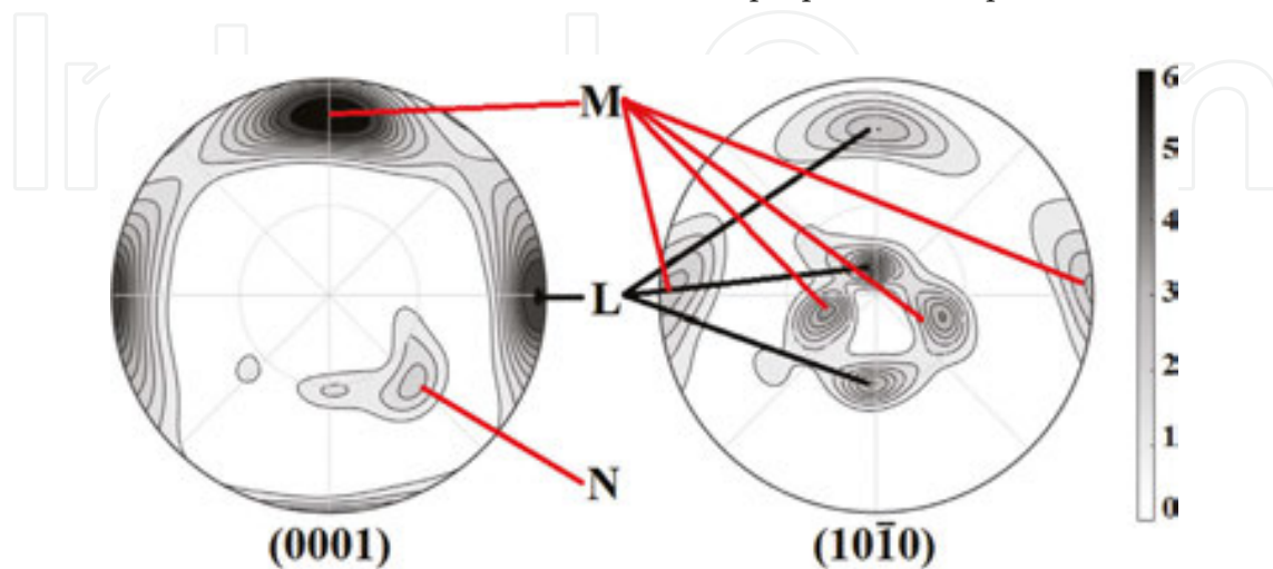
Figure 26. Depiction of the texture elements in the processed LAE442 alloy.
