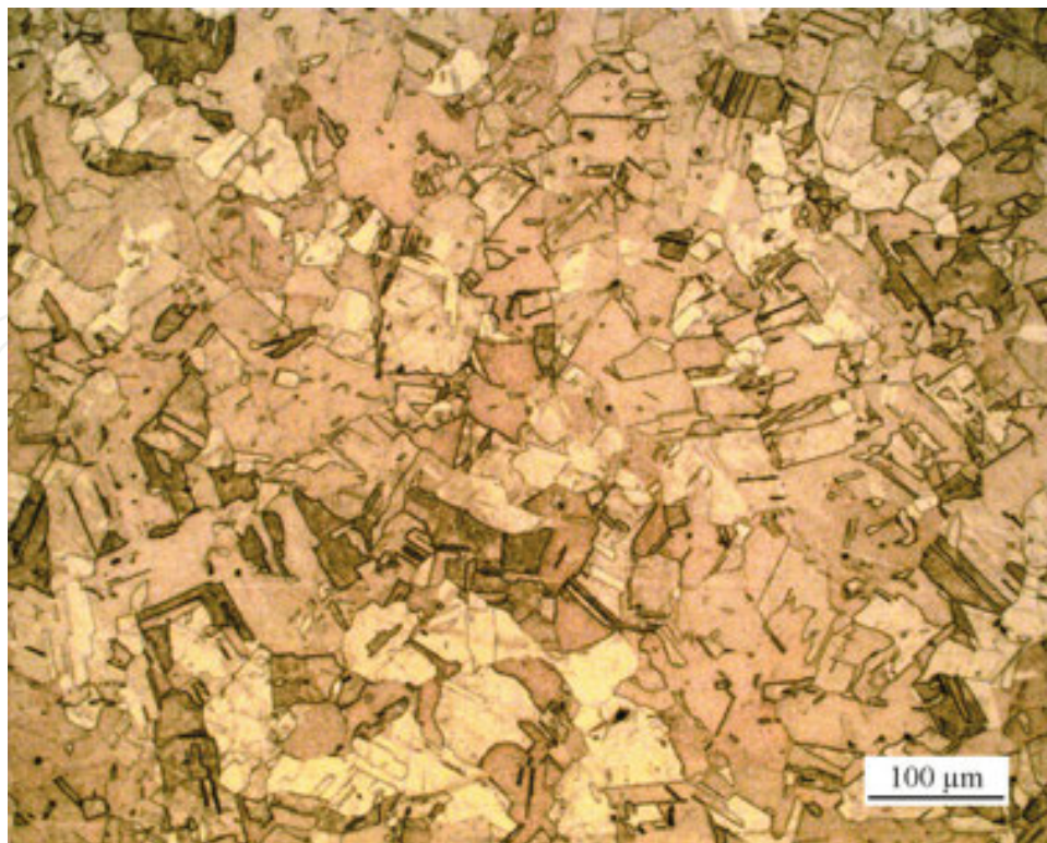
Figure 2. Microstructure of the non-deformed Cu.
