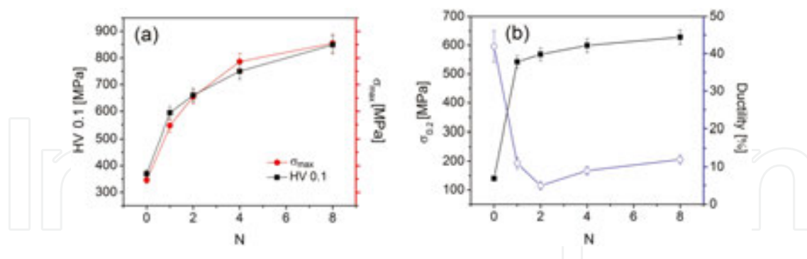
Figure 15. Development of (a) microhardness, tensile strength and (b) yield stress, ductility of IF steel with increasing numbers of ECAP passes.
