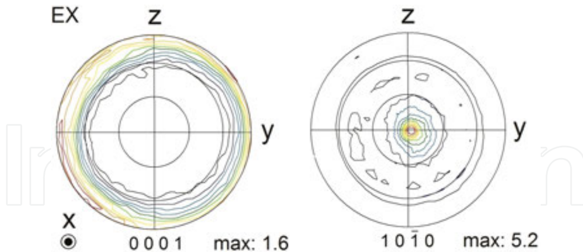
Figure 17. (0001) and (10 \bar{1}0 ) X-ray pole figure measured on cross-section.
