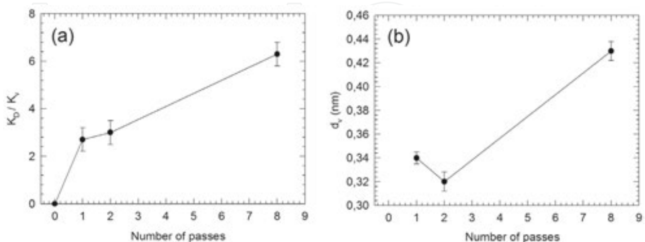
Figure 8. (a) The ratio K_D/K_v of positron trapping rate to dislocations and microvoids, (b) diameter of microvoids calculated from PAS results.
