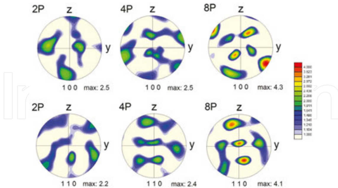
Figure 13. EBSD (100) and (110) pole figures for the IF steel samples processed by ECAP for different numbers of passes.
