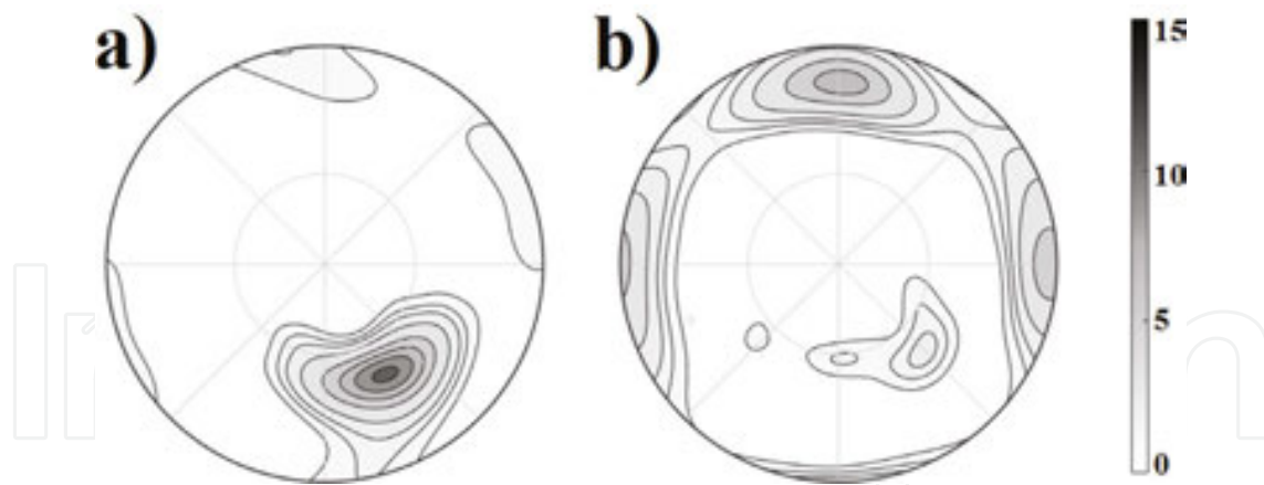
Figure 25. (0001) X-ray pole figure of (a) AE42 and (b) LAE442 after the final step of ECAP.
