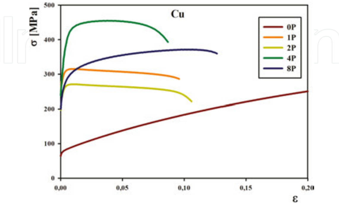
Figure 9. True stress vs. true strain curves of Cu specimens after different numbers of ECAP passes.
