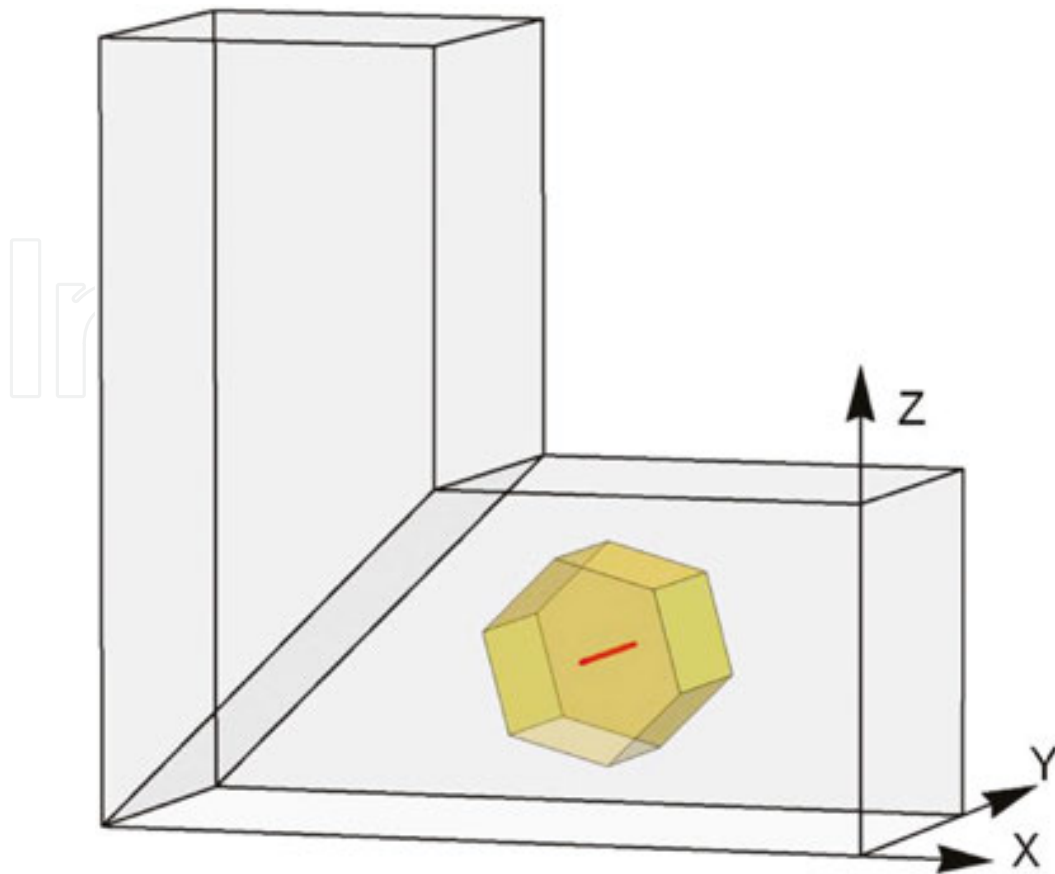
Figure 27. The formation mechanism of the texture component L.
