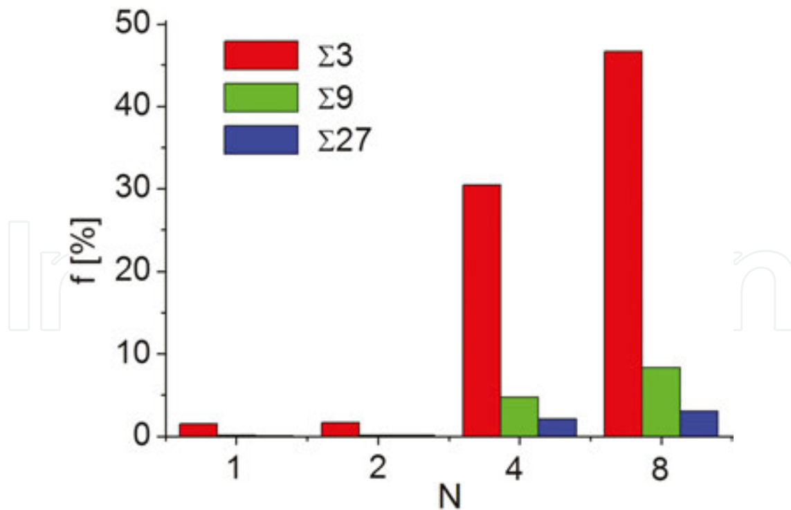
Figure 5. Special boundaries distribution.
