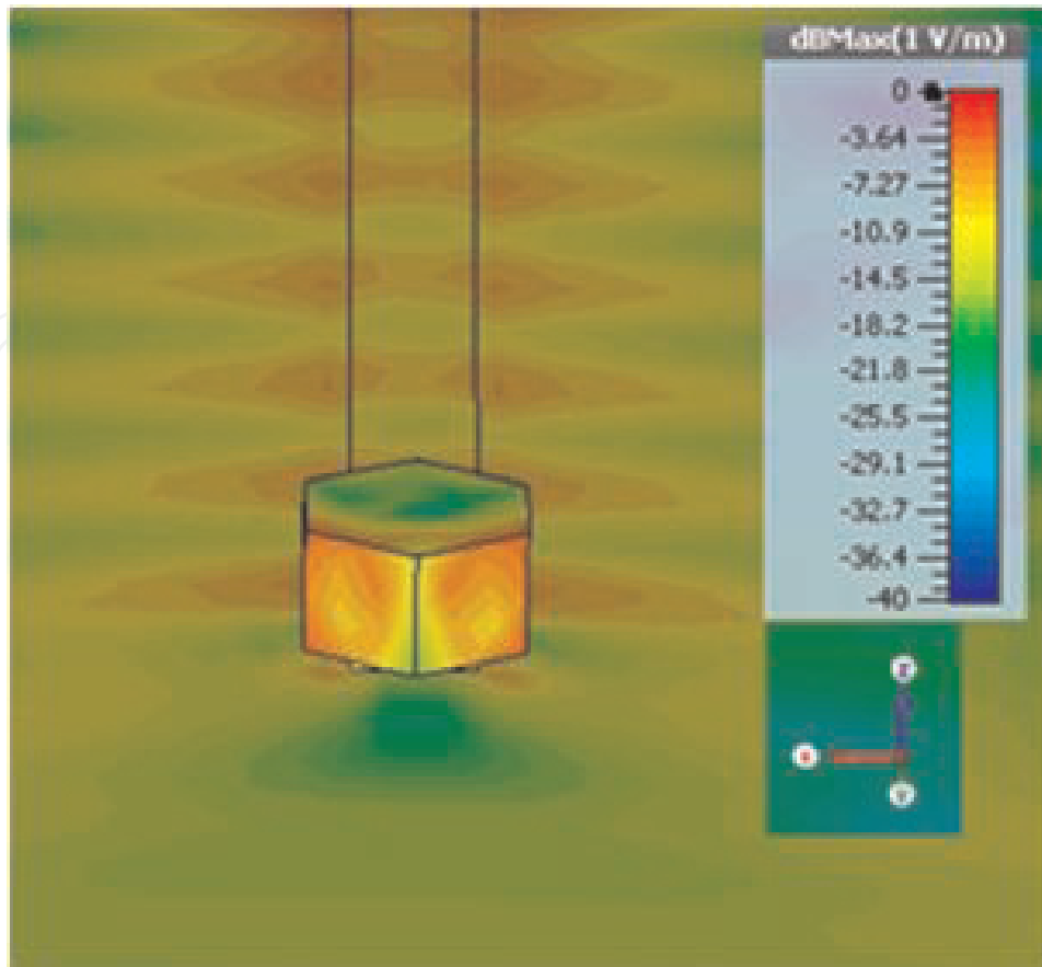
Figure 17. E-field distribution as shown via the magnitude at 193.5 THz with HE_{208} mode.
