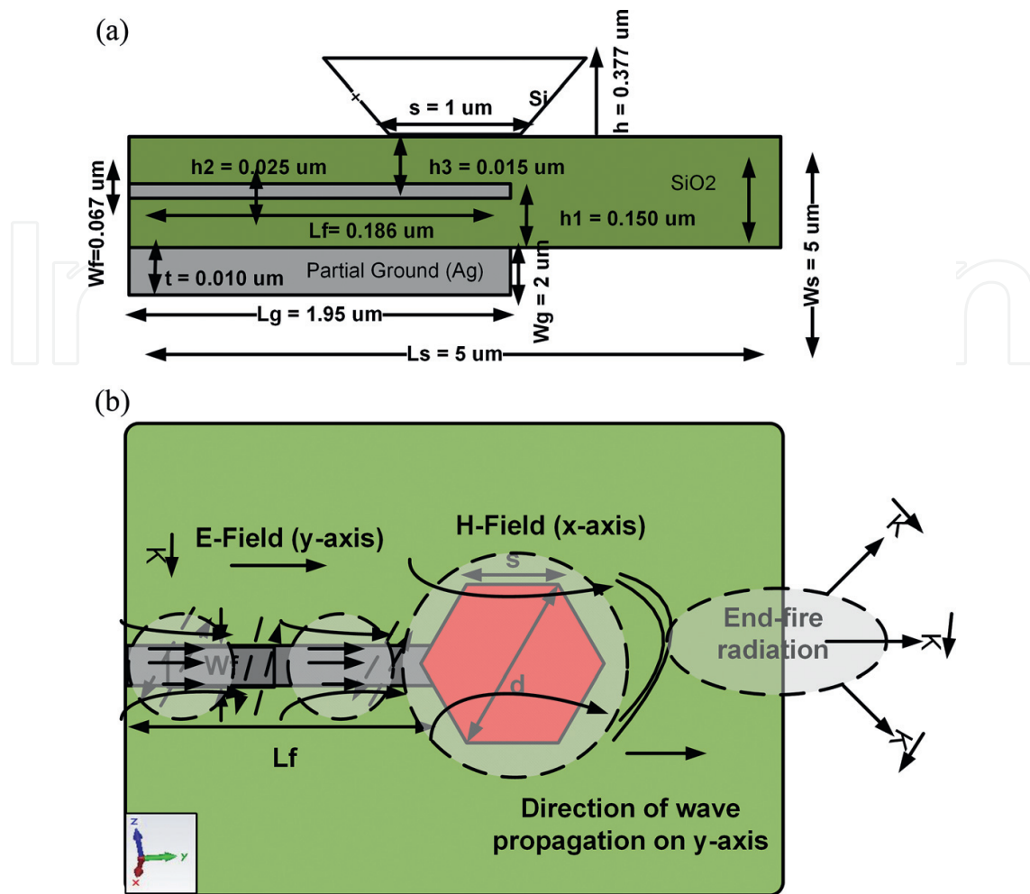
Figure 11. Geometry of hexagonal dielectric loaded nantenna (HDLN): (a) cross-sectional view; (b) front view with field vectors.
