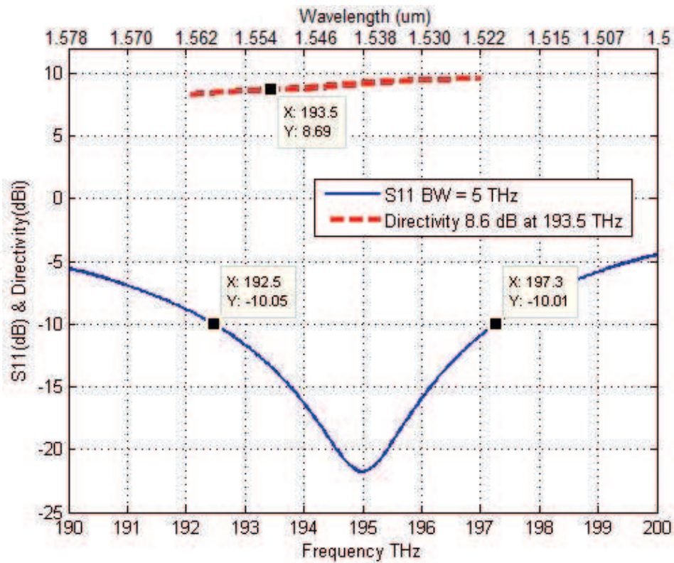
Figure 9. Simulated return loss and directivity of ETDNRNA.
