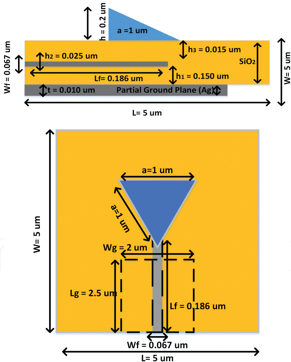
Figure 3. Antenna geometry of proposed nantenna design based on equilateral triangular DR (ETDRNA): (a) cross-sectional view; (b) front view.
