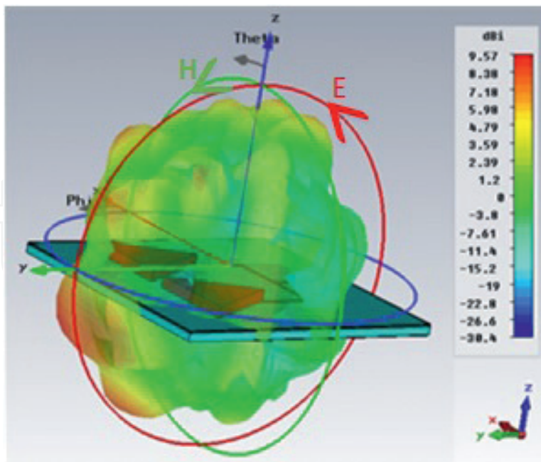
Figure 21. 3D radiation pattern at 193.5 THz.
