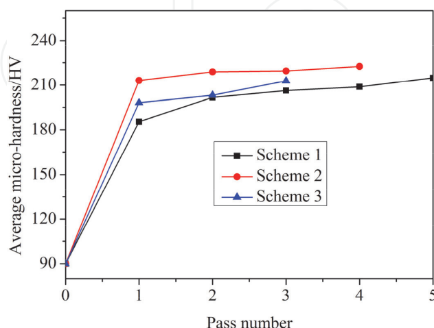
Figure 9. Average micro-hardness of Ni sheets before and after CGP.
