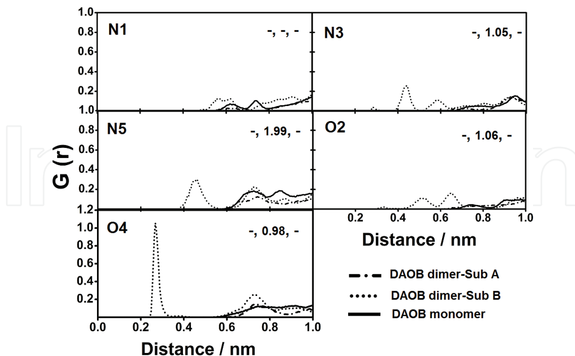
Figure 11. Radial distribution function of water molecules near the heteroatoms of Iso in DAOB. Vertical axes, G(r) , denote the radial distribution functions. Red, blue, and black numbers showed the mean number of water molecules in Sub A and Sub B of DAOB dimer, and DAOB monomer is indicated in red, blue, and black, respectively. The data for the DAOB dimer are taken from [56] and for DAOB monomer from [55]. (Reproduced by permission of The Royal Society of Chemistry).
