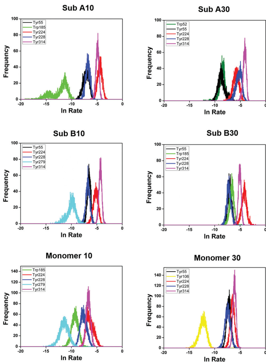
Figure 5. Distribution of logarithmic ET rate from aromatic amino acids to Iso*. Sub A10 and Sub B10 denote Sub A and Sub B at 10°C, and Sub A30 and Sub B30 denote Sub A and Sub B at 30°C in DAAD dimer, respectively. Inserts show amino acids with the top fastest ET rates. The distributions for DAAD monomers at 10°C (Monomer 10) and 30°C (Monomer 30) are also shown for comparison. The kinds of the amino acids are different among the six groups including monomer. (Reproduced from [53] with permission from the PCCP Owner Societies).
