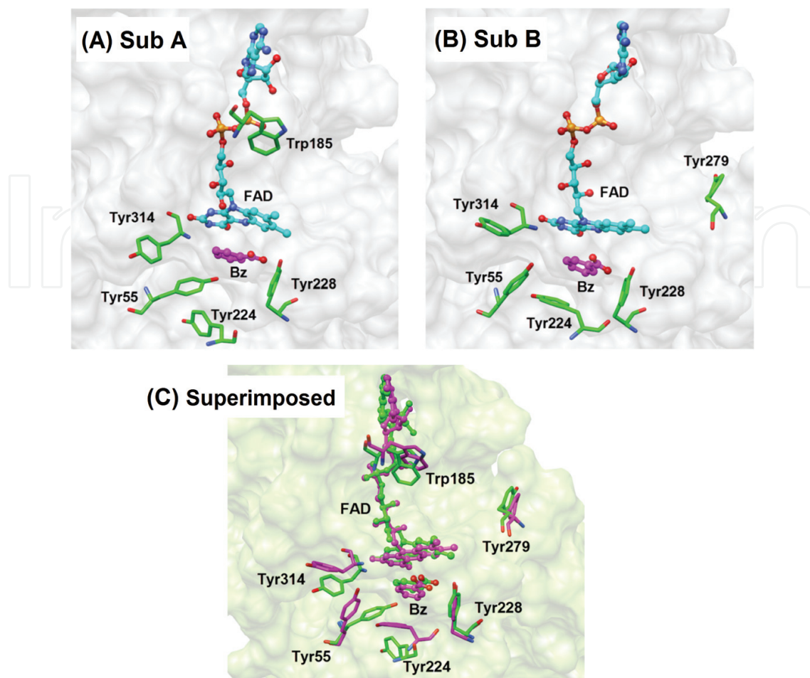
Figure 7. Structure of DAOB dimer at FAD binding site. (A) Sub A, (B) Sub B show subunits A and B in DAOB dimer. (C) Superimposed shows superimposition of Sub A and Sub B. The potential ET donors, Bz, Tyr224, Tyr228, Tyr314, Tyr55, Tyr279, and Trp185, are shown in addition to FAD. In bottom panel FAD and the aromatic amino acids are indicated in green for Sub A, and in magenta for Sub B. MDS calculation was performed at 20 °C. The data are taken from [56]. (Reproduced by permission of the Royal Society of Chemistry).
