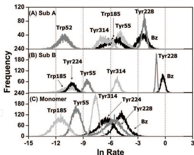
Figure 6. Comparison of the distribution of ln Rate between DAOB dimer and monomer. (A) Sub A and (B) Sub B in the dimer. It was identified that the observed fluorescence lifetime of the dimer, \tau_1^{obs} = 0.848 ps, is from Sub B and \tau_2^{obs} = 4.77 ps is from Sub A. Inserts denote six fastest ET donors both in Sub A and Sub B. The distribution in the monomer is also shown in (C) Monomer. The data are taken from [56]. (Reproduced by permission of The Royal Society of Chemistry).
