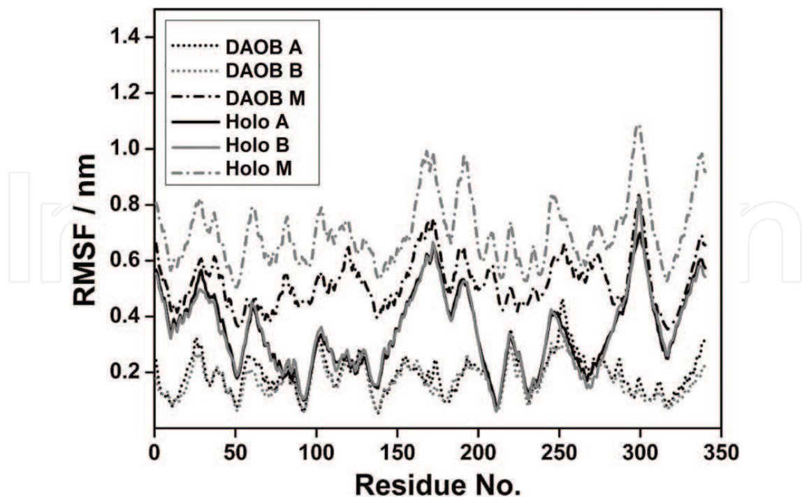
Figure 9. Comparison of root of mean square fluctuations among DAAO dimer, DAAO monomer, DAOB dimer, and DAOB monomer. Root of mean square fluctuations (RMSFs) were obtained by AMBER 10. Holo M, Holo A, and Holo B in the insert denote the DAAO monomer, Sub A, and Sub B of the DAAO dimer, respectively. DAOB M, DAOB A, and DAOB B denote the DAOB monomer, Sub A, and Sub B of the DAOB dimer, respectively. RMSFs of DAAO monomer were taken from [54], those for DAAO dimer from [53] and those of DAOB monomer from [55], and DAOB dimer from [56]. (Reproduced by permission of the Royal Society of Chemistry).
