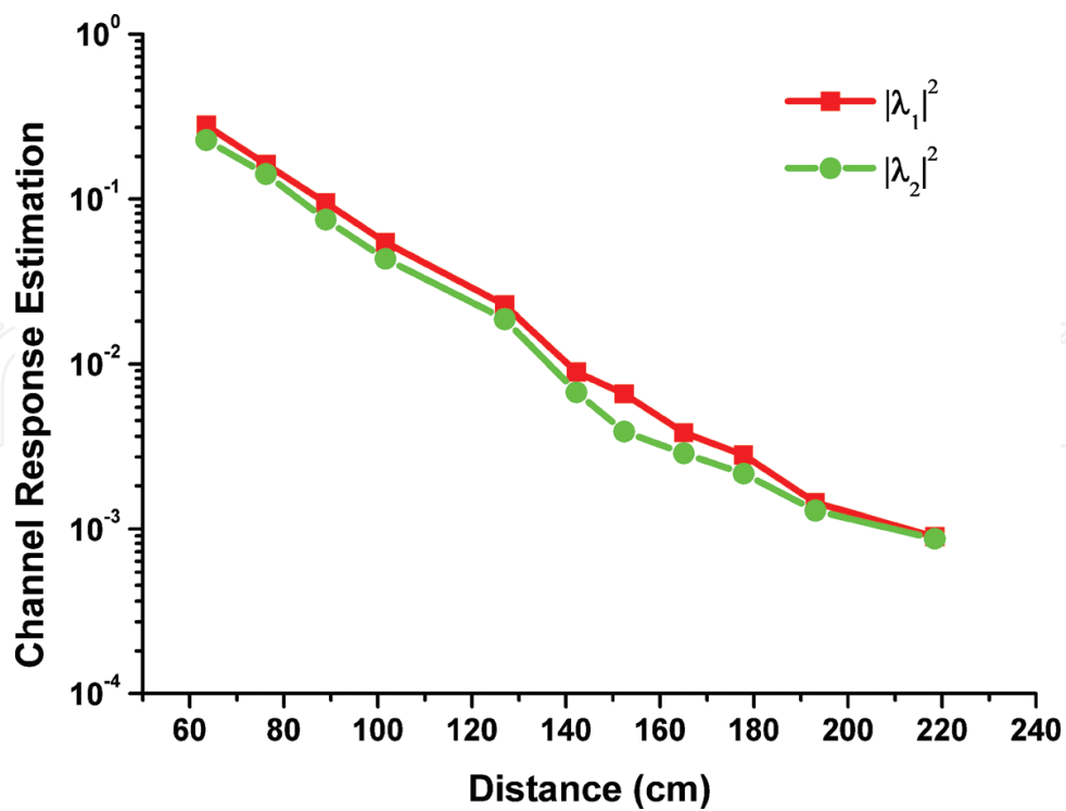
Figure 21. Channel estimation against link distance for 2 × 2 M-QAM MIMO VLC.
