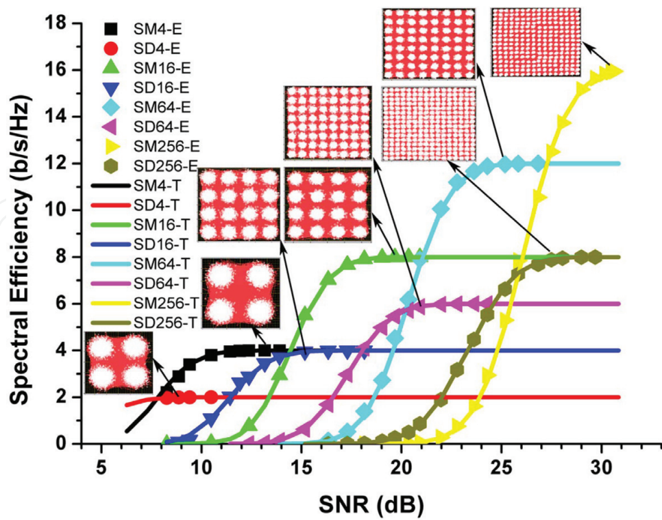
Figure 20. Spectral efficiency performance of M-QAM 2 × 2 MIMO VLC using spatial multiplexing and spatial diversity. Dots are experimental results and lines are theoretical results. Insets are the corresponding constellation diagrams.
