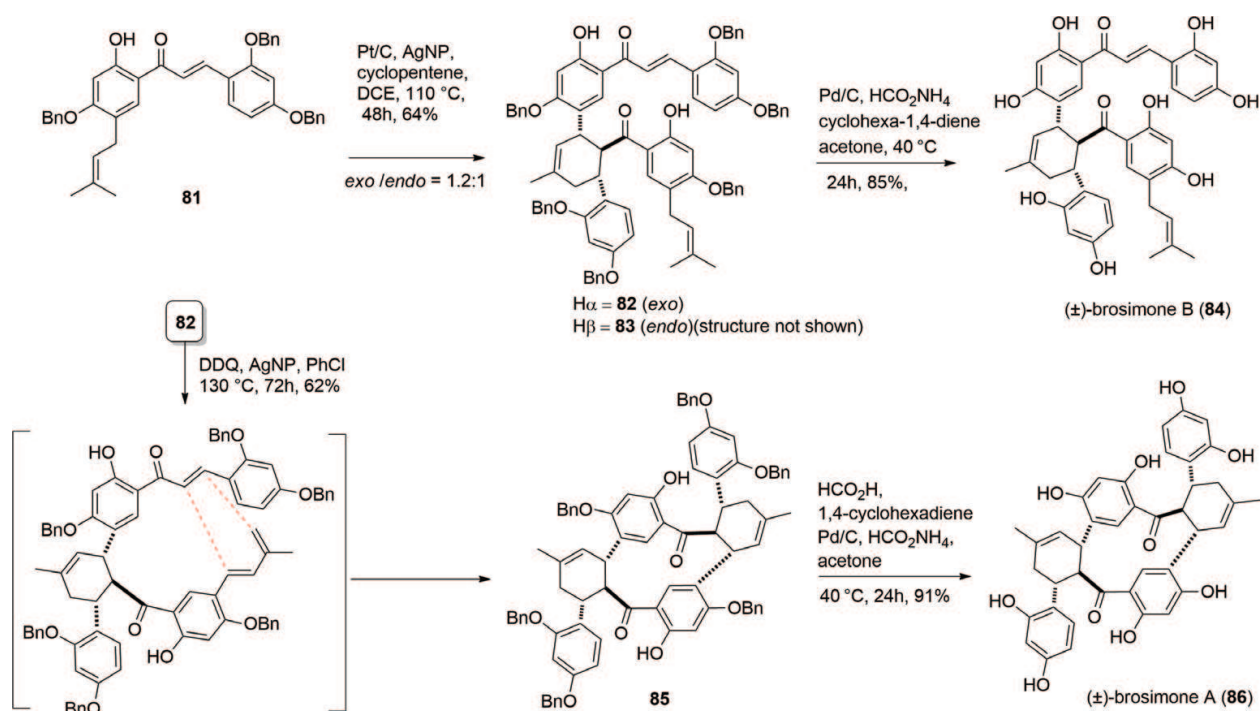
Scheme 11. Biomimetic synthesis of (±)-brosimone A and (±)-brosimone B [38].
