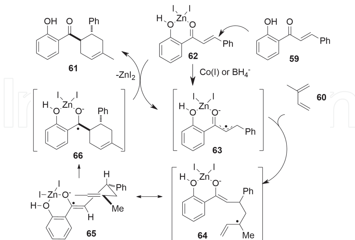
Scheme 4. Proposed mechanism for an electron transfer-initiated Diels-Alder cycloaddition reaction [33].
