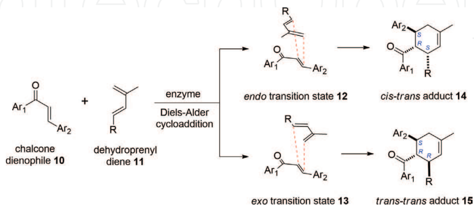
Scheme 1. Stereochemistry on the cyclohexene ring of flavonoid Diels-Alder natural products.
