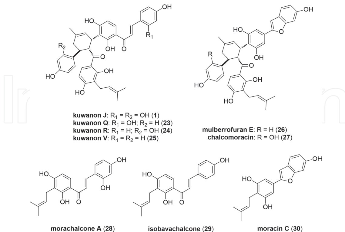
Figure 3. Metabolites isolated from the Morus alba cell cultures [15–18].
