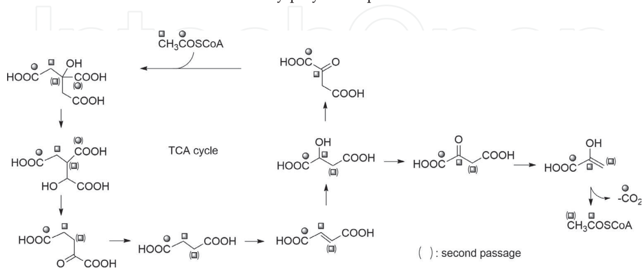
Figure 6. Formation of reorganized [1, 2- 13 C 2 ]acetate through the TCA cycle [19].
