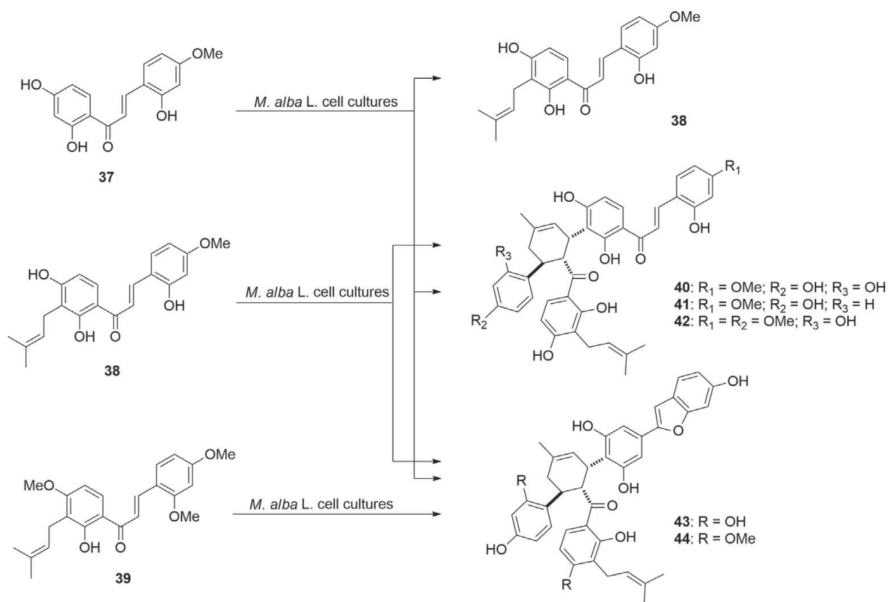
Figure 8. Feeding experiments of methoxychalcone derivatives to the M. alba cell cultures [22].
