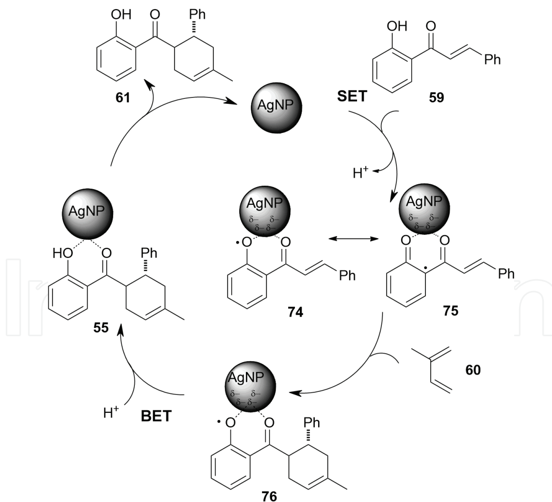
Scheme 8. Proposed mechanism for the silver nanoparticles-catalyzed Diels-Alder reaction [36].
