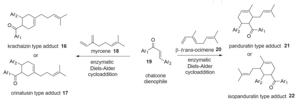
Figure 2. Plausible biosynthesis of flavonoid Diels-Alder natural products that derived from a monoterpene.
