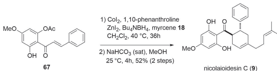
Scheme 5. Biomimetic synthesis of ( \pm )-nicolaioidesin C ( 9 ) [33].
