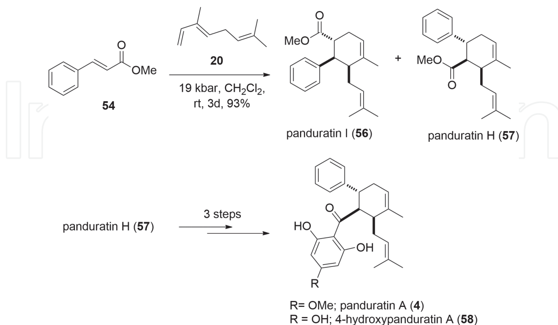
Scheme 3. Biomimetic synthesis of ( \pm )-panduratin A and ( \pm )-4-hydroxypanduratin A by using high pressure conditions [31].
