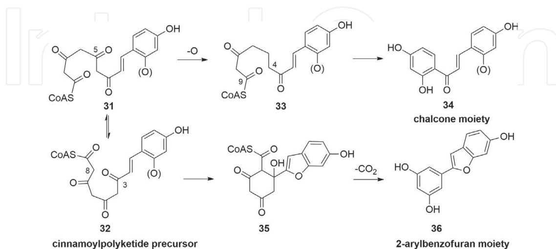
Figure 5. Hypothesized conversion of the chalcone and 2-arylbenzofuran moieties from cinnamoylpolyketide precursor [19].
