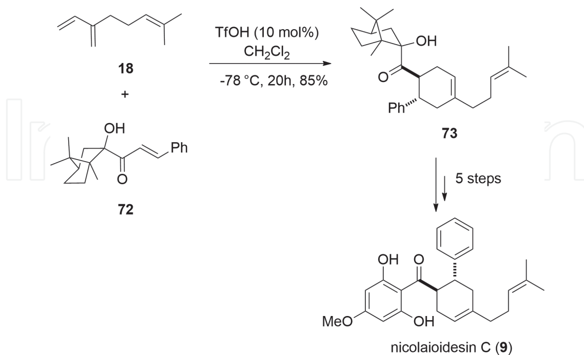
Scheme 7. Asymmetric biomimetic synthesis of (-)-nicolaioidesin C ( 9 ) [35].
