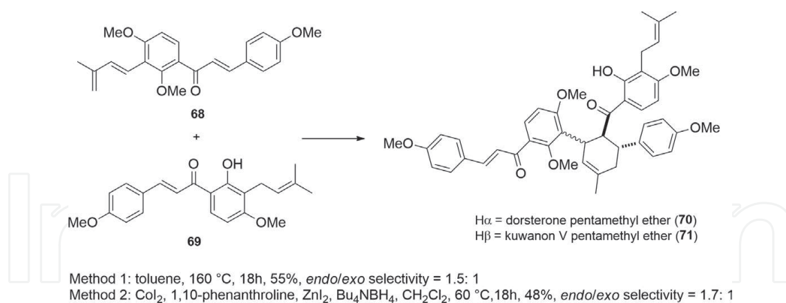
Scheme 6. Biomimetic synthesis of (±)-dorsterone and (±)-kuwanon V pentamethyl ethers [27].
