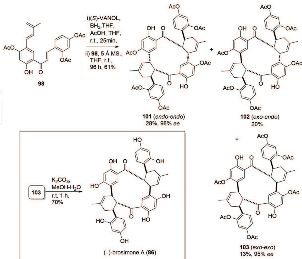
Scheme 15. Enantioselective synthesis of (-)-brosimone A [39].
