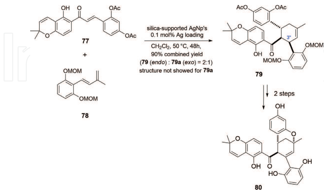
Scheme 10. Biomimetic synthesis of ( \pm )-sorocenol B [37].
