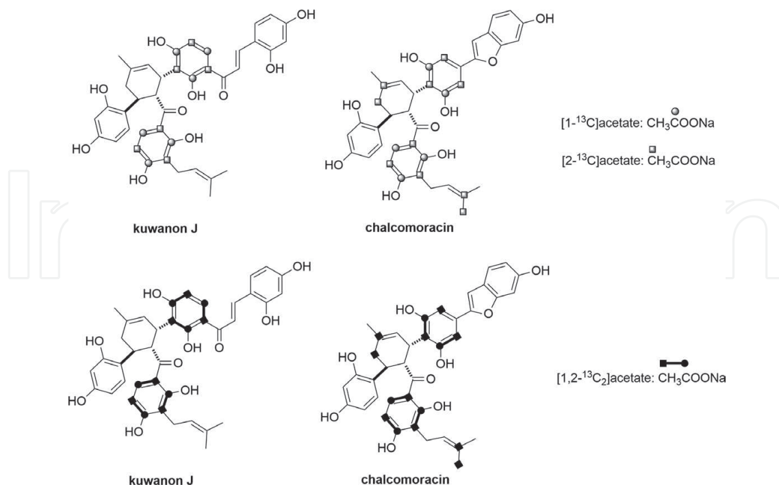
Figure 4. ^{13}\text{C} -labeling patterns of Kuwanon J and chalcomoracin from [1-^{13}\text{C}] -, [2-^{13}\text{C}] -, or [1, 2-^{13}\text{C}_2] acetate [19].
