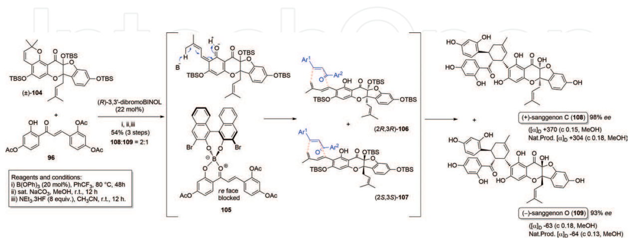
Scheme 16. Asymmetric synthesis of sanggenons C ( 108 ) and O ( 109 ) [41].
