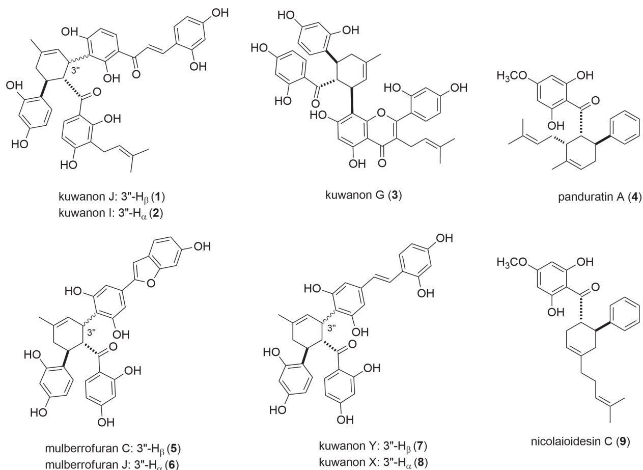
Figure 1. Examples of flavonoid Diels-Alder natural products.
