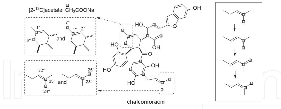
Figure 7. Two independent ^{13}\text{C} -labeling patterns at the isoprenyl units of chalomoracin and the transfer of the ^{13}\text{C} -labeling from cis -methyl carbon to trans -methyl carbon through the diene formation [8, 19].
