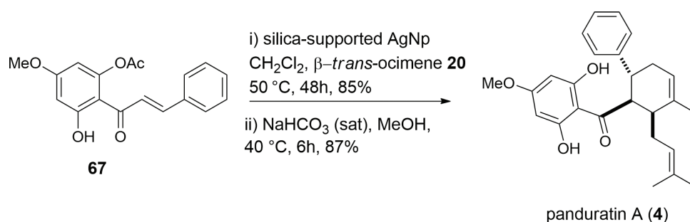
Scheme 9. Synthesis of ( \pm )-panduratin A ( 4 ) [36].
