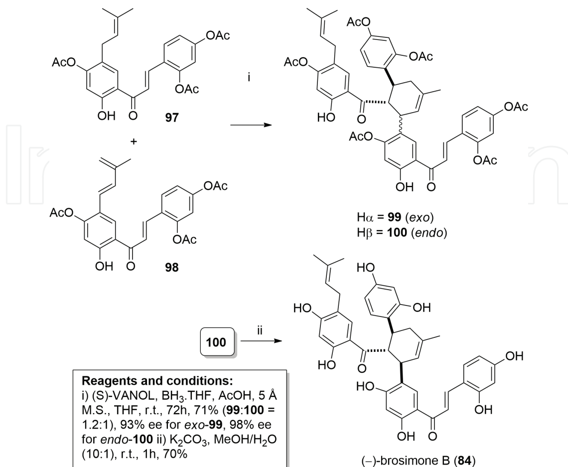
Scheme 14. Enantioselective synthesis of (-)-brosimone B [39].
