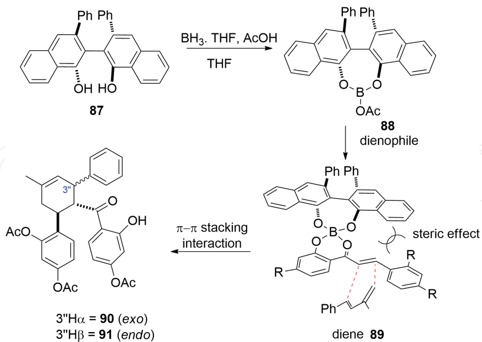
Scheme 12. Proposed mechanism for the chiral ligand-Lewis acid complex mediated enantioselective Diels-Alder reaction [39, 40].
