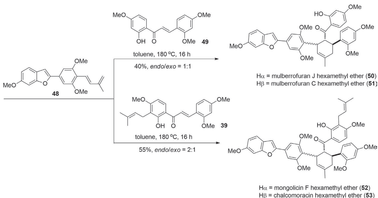
Scheme 2. Synthesis of (±)-mulberrofuran J ( 50 ), (±)-mulberrofuran C ( 51 ), (±)-mongolicin F ( 52 ), and (±)-chalconoracine ( 53 ) hexamethyl ethers by thermal Diels-Alder reaction [24].
