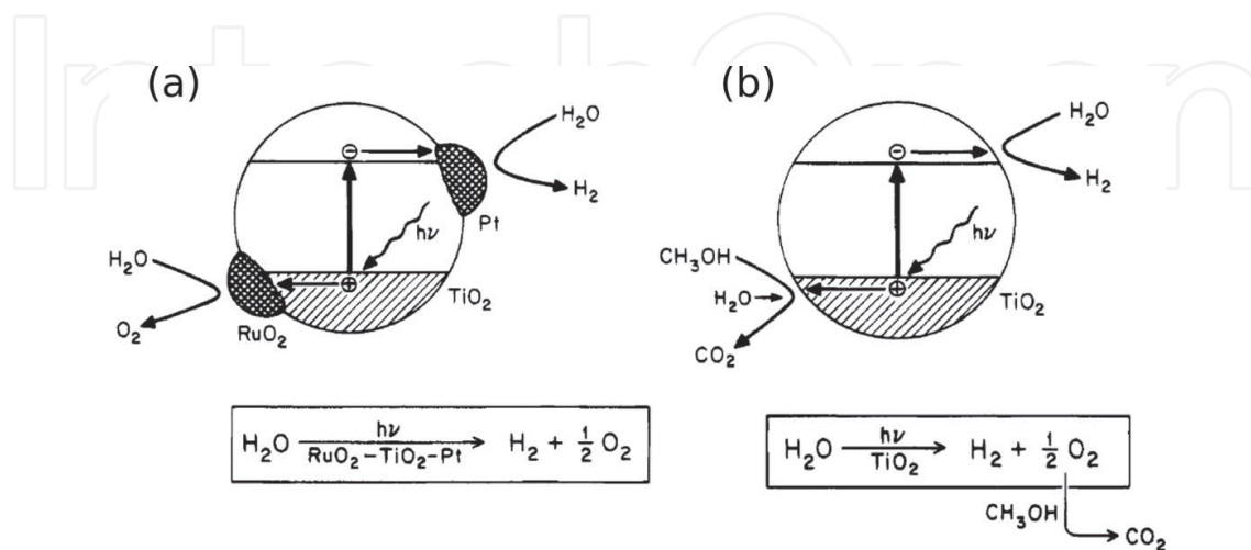
Figure 3. (a) Photosplitting of water on a composite catalyst. (b) Photosplitting of water: sacrificial donor effect. Reprinted with the permission from Ref. [85]. Copyright (1995) American Chemical Society.
