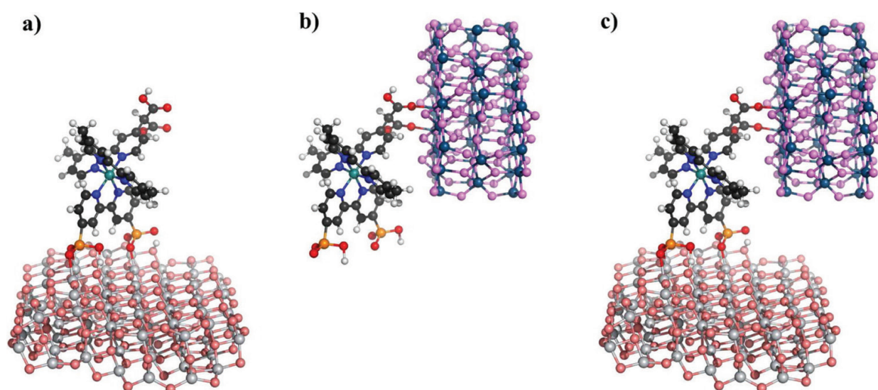
Figure 4. Optimized molecular structure of Ru-dye in its partially deprotonated form, grafted to the (\text{TiO}_2)_{82} cluster (a), to the (\text{IrO}_2)_{56}, 2\text{H}_2\text{O} nanoparticle (b), and tethered across the \text{TiO}_2 and \text{IrO}_2 systems, (c). Reprinted with the permission from Ref. [96] Copyright (2015) American Chemical Society
