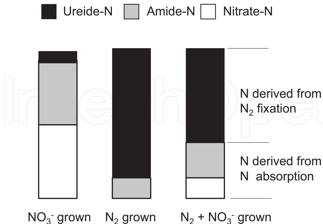
Figure 13. Concept of the simple ureide method for estimating N derived from nitrogen fixation and soil + fertilizer N.
