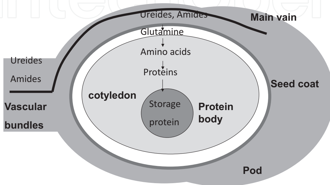
Figure 21. Model of the flow of ureides and amino acids in soybean pod to a seed.
