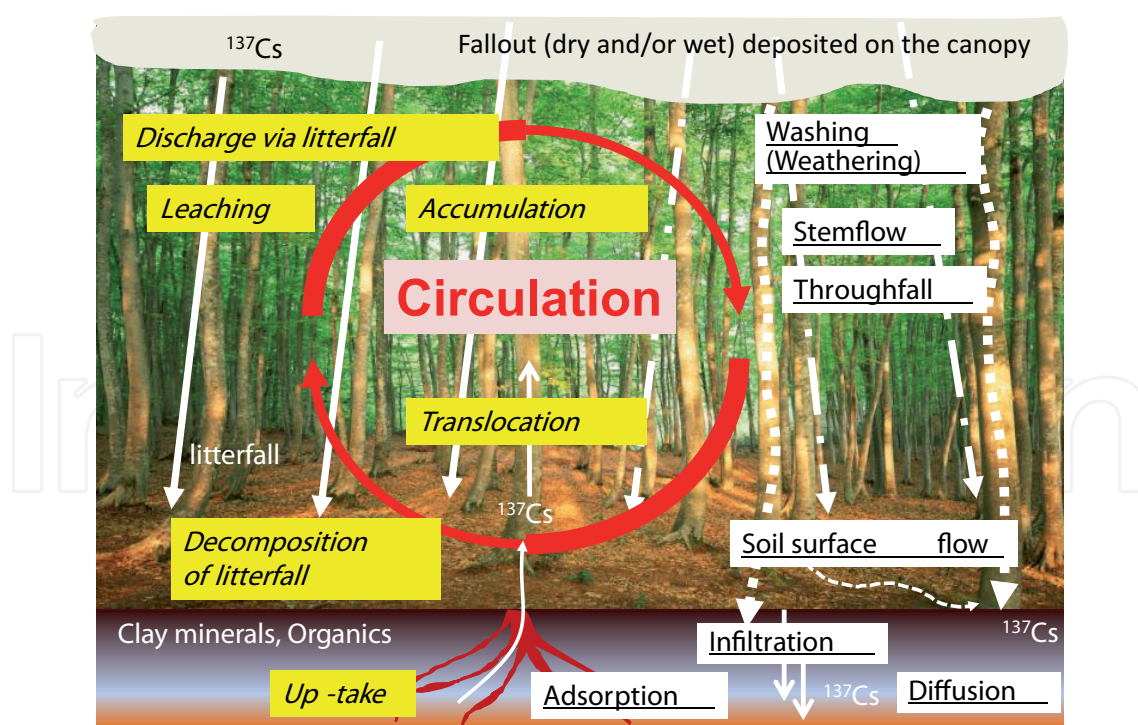
Figure 1. A possible circulation and translocation of radiocesium in forest vegetation is described with related natural forces. The terms written in italics ( Accumulation , Leaching , Translocation , Discharge , Decomposition , and Uptake ) and those with an underline ( others ) are showing forces related to biological activities and meteorological/geological activities, respectively.
