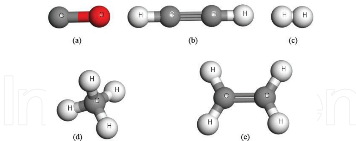
Figure 4. Optimized supercell structures for (a) CO, (b) C 2 H 2 , (c) H 2 , (d) CH 4 , and (e) C 2 H 4 .
