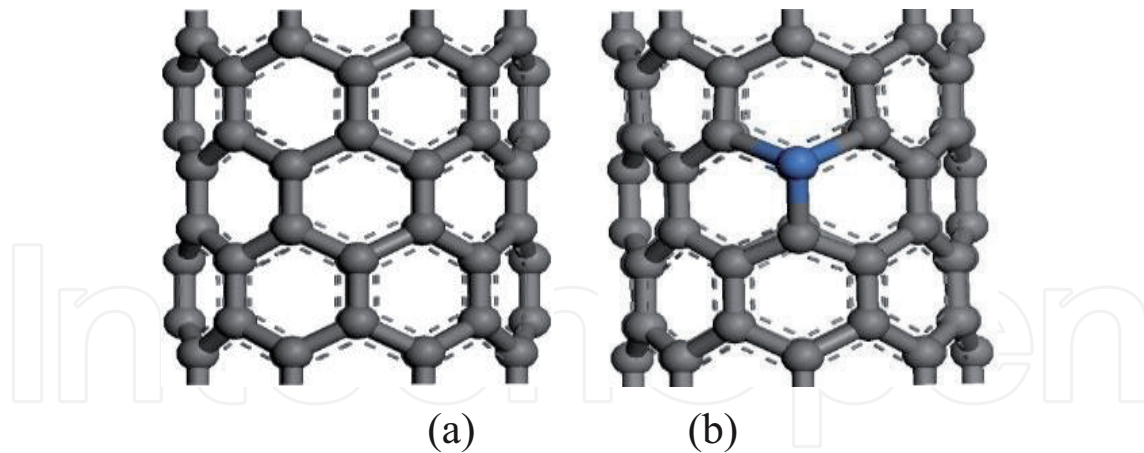
Figure 7. Geometrical structures of CNTs and Ni-CNTs. (a) CNTs, (b) Ni-CNTs.
