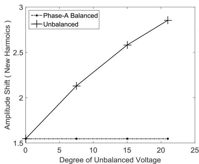
Figure 17. Characteristic of new harmonic on phase-A.
