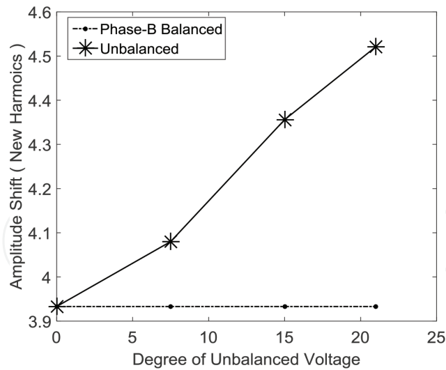
Figure 18. Characteristic of new harmonic on phase-B.
