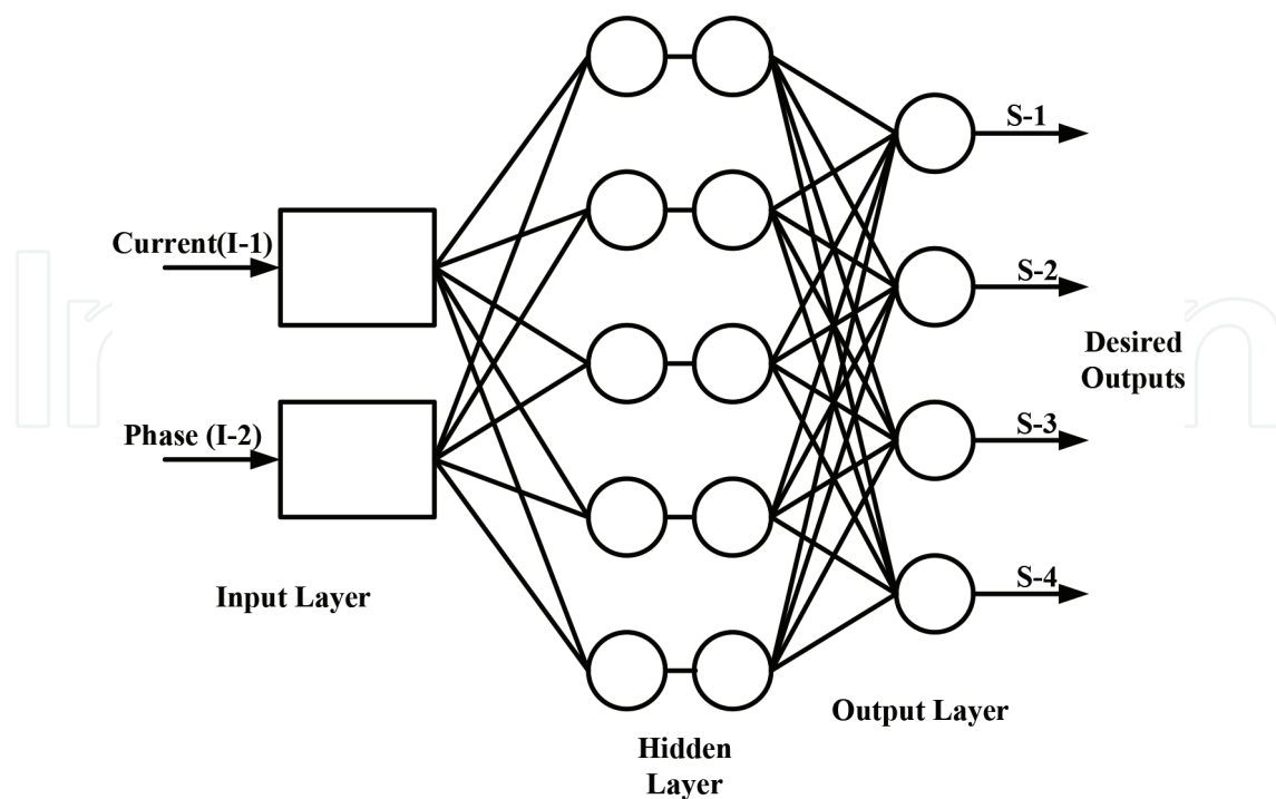
Figure 15. ANN architecture.
