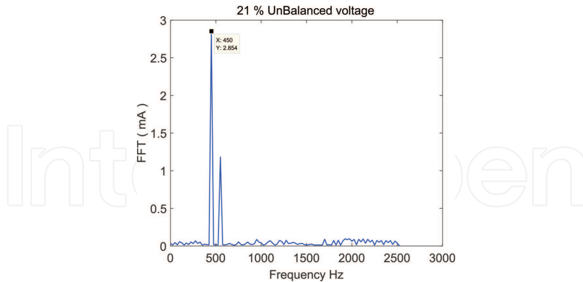
Figure 14. 21% Unbalanced voltage.
