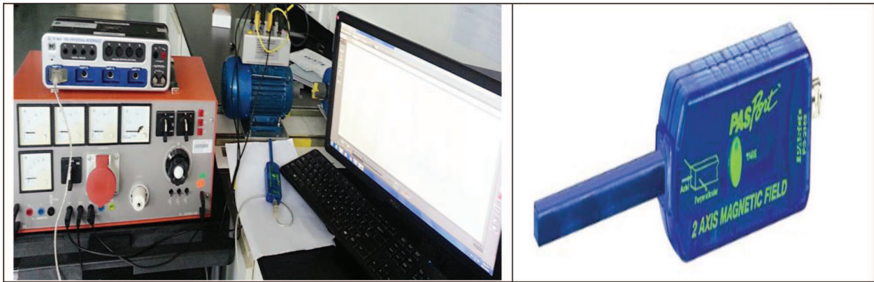
Figure 5. Test rig for measuring MMF.
