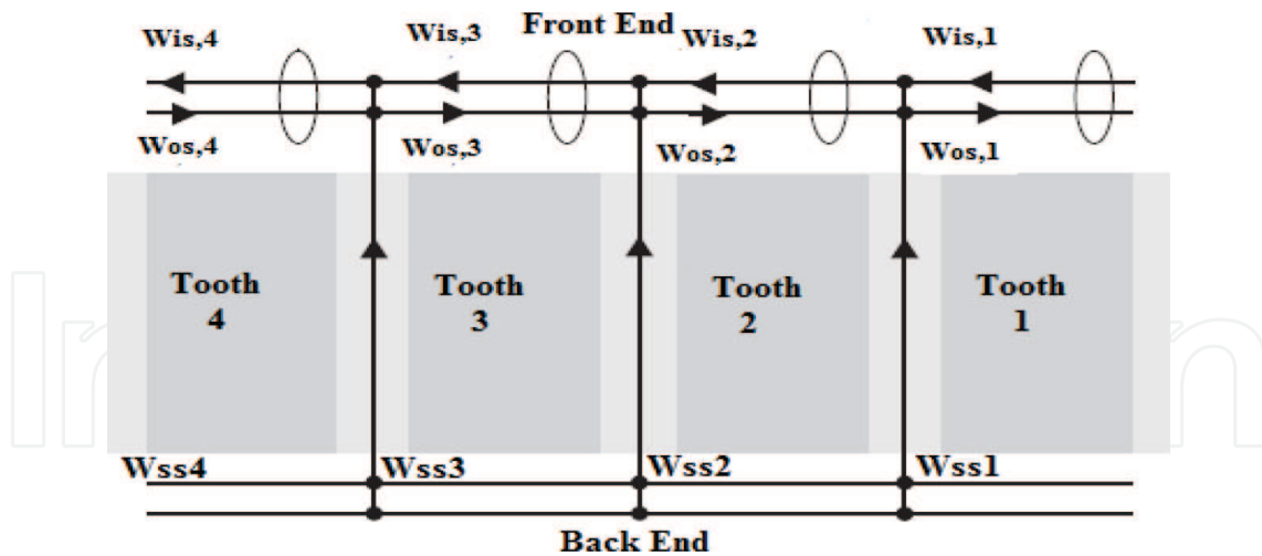
Figure 3. A version center view of stator through a developed diagram.
