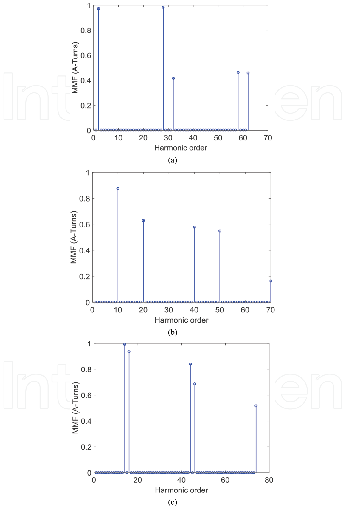
Figure 8. Harmonic order of MMF ( p = 2 , R = 30 , \mu = 1, 5 , and 7 ).
