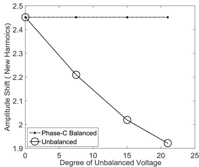
Figure 19. Characteristic of new harmonic on phase-C.
