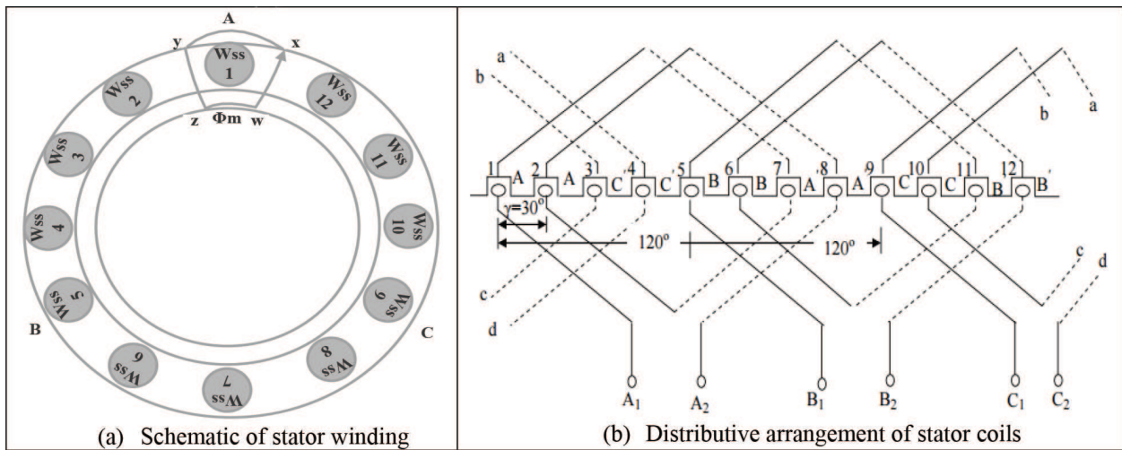
Figure 1. Stator winding arrangement in the slots.
