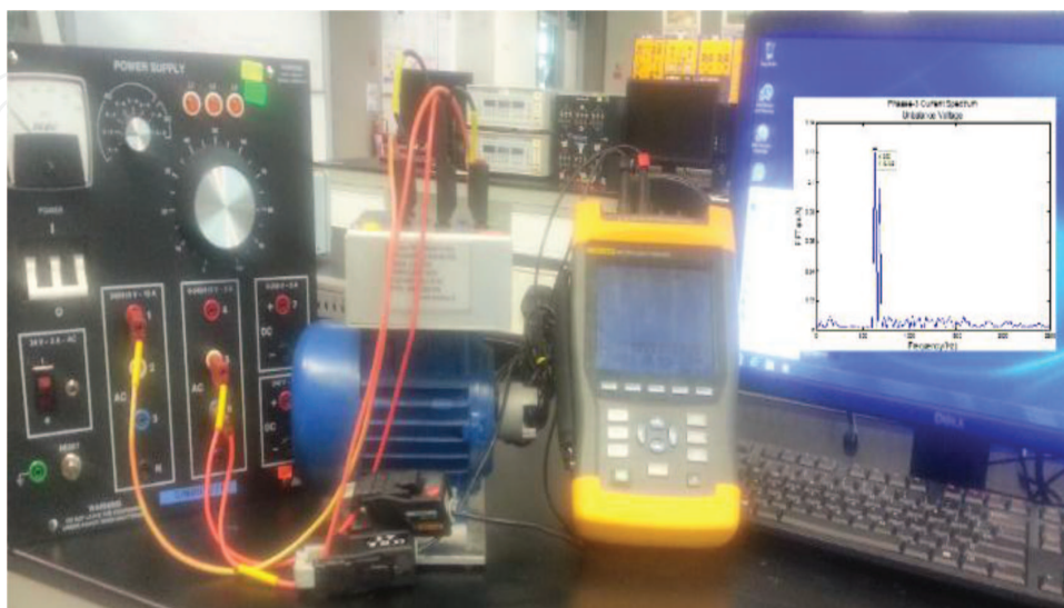
Figure 10. Experimental setup.
