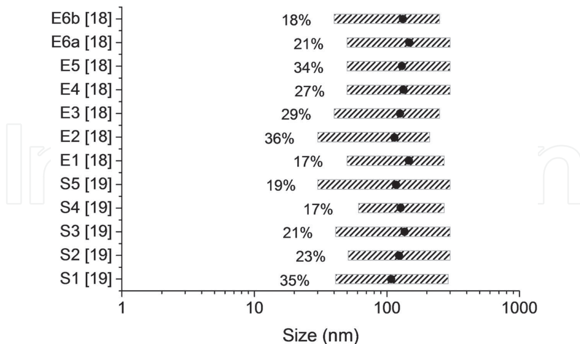
Figure 2. Size distribution (dashed rectangles), mean size (black dots) and percentage of nanoparticles in number (%) of food-grade TiO 2 particles characterized by (E) Dufey et al. [18] and (S) Yang et al. [19]. The mean sizes of the distribution vary between 106 and 145 nm.
