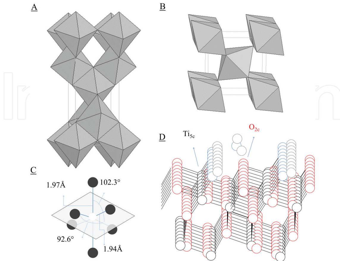
Figure 1. Bulk structures of (A) anatase, (B) rutile with (C) bond lengths and angles of the octahedrally coordinated Ti atoms in anatase, arranged from Diebold [17] and (D) arrangement of atoms on the (101) surface of anatase after adsorption and dissociation of water with Ti (grey filled balls), O from \text{TiO}_2 structure (empty balls), O from water (big hatched balls) and H from water (small hatched balls).
