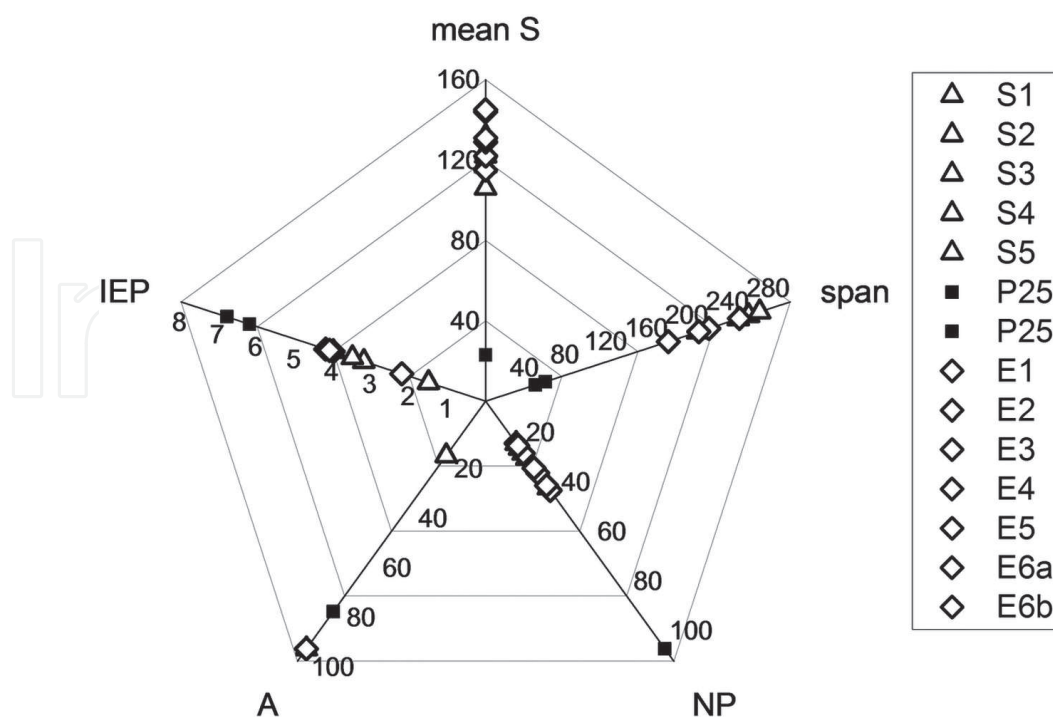
Figure 3. Physical and chemical parameters describing E171 and P25 forms of \text{TiO}_2 , namely the content in NPs, isoelectric point (IEP), the mean size of the distribution deduced by transmission electron microscopy (mean S) and the span of the particle size distribution (span). Data come from references [8, 19].
