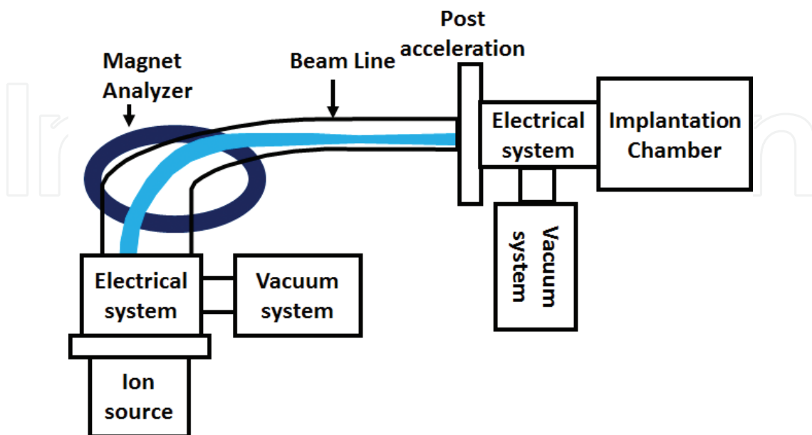
Figure 1. Ion implanter.
