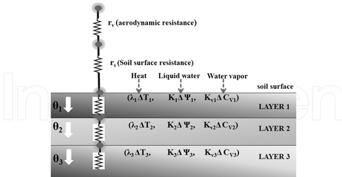
Figure 2. Scheme of the computational grid with the driving force terms (temperature, soil water potential, and soil vapor concentration), the soil conductivities and the resistances involved at the soil-atmosphere interface (adapted from Bittelli et al. [26]). The black dot is the mass balance for heat flow and water flux at a given node.
