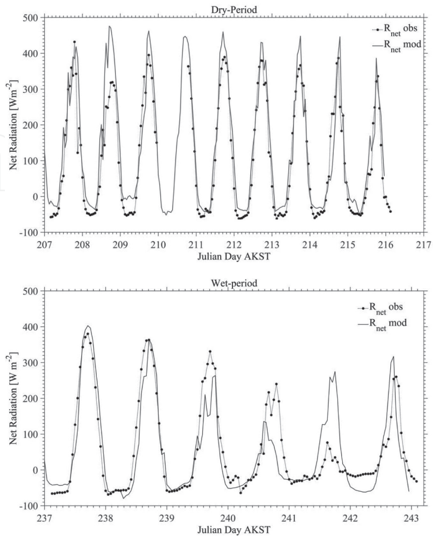
Figure 4. Simulated and measured hourly data of net radiation during the dry and wet period as a function of time. (Top panel) Dry period from 26 July to 3 August 2013 (Julian day 207–216) (bottom panel) wet period from 25 to 30 August 2013 (Julian day 237–242).
