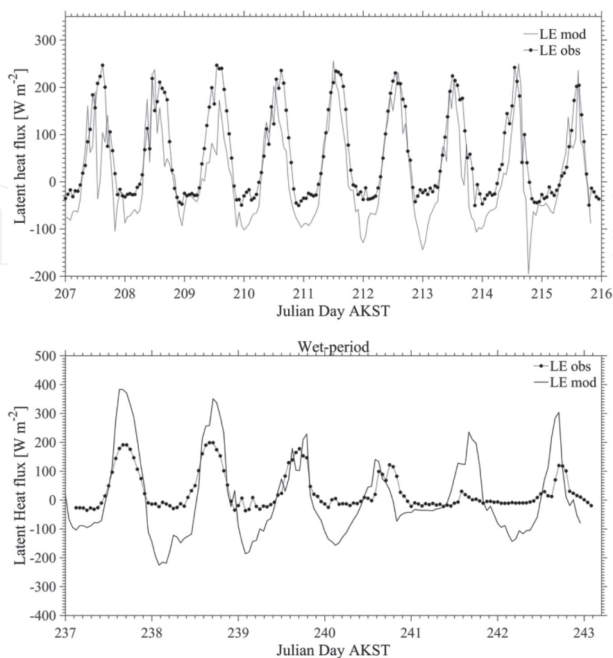
Figure 7. Evapotranspiration time series observed and modeled. (Top panel) Dry period from 26 July to 3 August 2013 (Julian day 207–216) (bottom panel) wet period from 25 to 30 August 2013 (Julian day 237–242).
