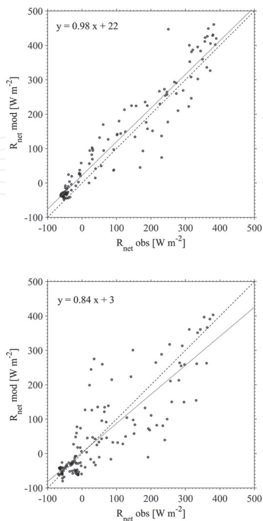
Figure 5. Comparison between the hourly observation of net radiation ( R_{\text{net, obs}} ) and the simulation of net radiation ( R_{\text{net, mod}} ) during the dry and wet period. (Top panel) Dry period from 31 July to 3 August 2013 (Julian day 210–215) and during the wet period (bottom panel) from 25 to 30 August 2013 (Julian day 237–242).
