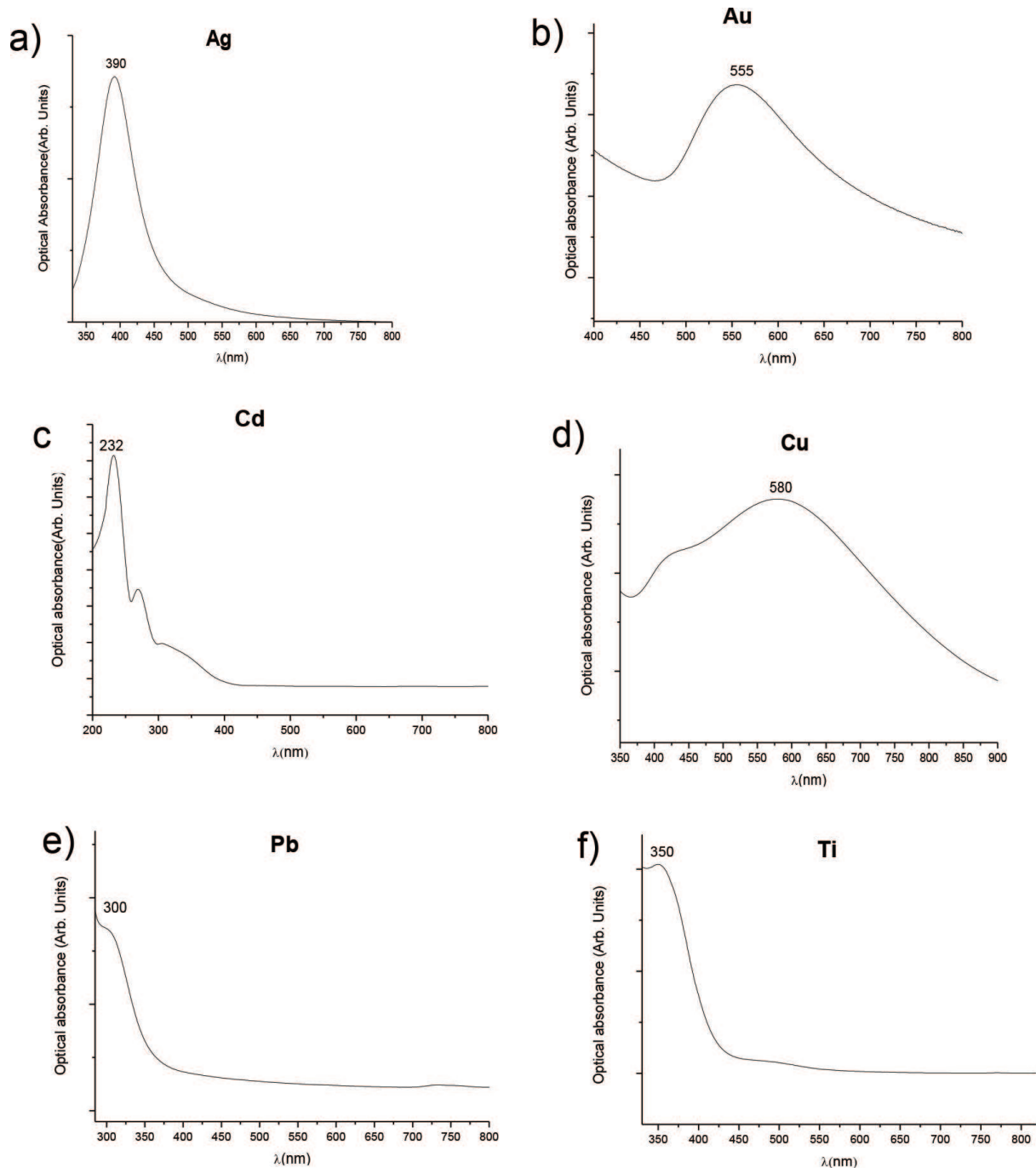
Figure 4. Optical absorbance of metallic nanoparticles synthesized by O. ficus-indica extract.
