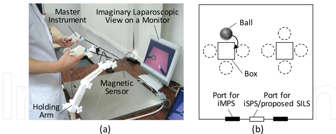
Figure 4. Object-moving task: (a) experimental set-up during the task in iMPS and (b) task detail; black port for iMPS and white port for iSPS and proposed SILS.
