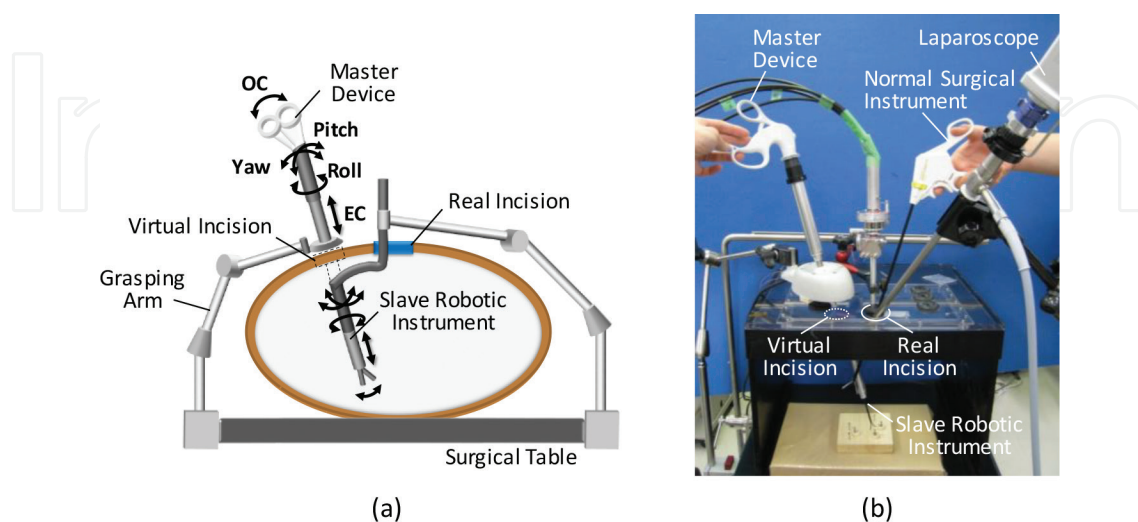
Figure 6. Local-operated master-slave robot system: (a) concept of proposed system and (b) surgical instrumental set-up for single-incision laparoscopic cholecystectomy.
