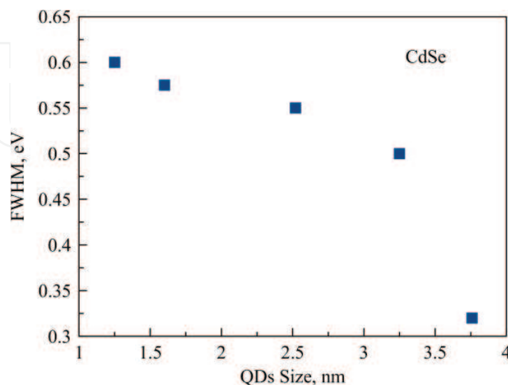
Figure 8. Dependence of the PL FWHM magnitudes for glasses doped with CdSe QDs with different sizes.
