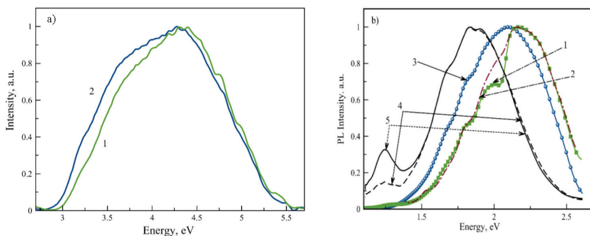
Figure 15. PL excitation spectrum of the glass doped with MCs ( \text{PbS} ) n ( \lambda_{\text{lum}} = 540 \text{ nm} ) (a) Luminescence spectra of the glasses doped with MCs ( \text{PbS} ) n : as-prepared (1) and after heat treatment at T_{\text{HT}} = 410^\circ\text{C} within 10 min (2), 20 min (3), 30 min (4) and 40 min (5) ( \lambda_{\text{exc}} = 250 \text{ nm} ) (b).
