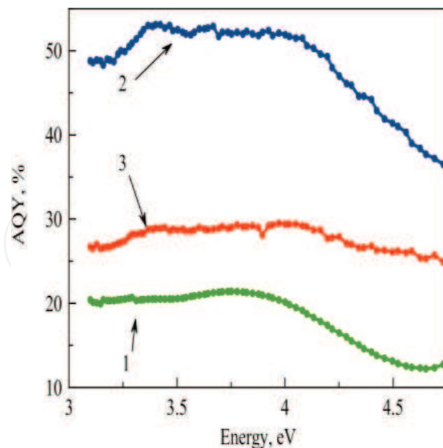
Figure 6. Dependence of the PL AQY for FP glasses doped with CdSe QDs with sizes 2.0 nm (1), 3.0 nm (2) and 4.0 nm (3) on the excitation energy.
