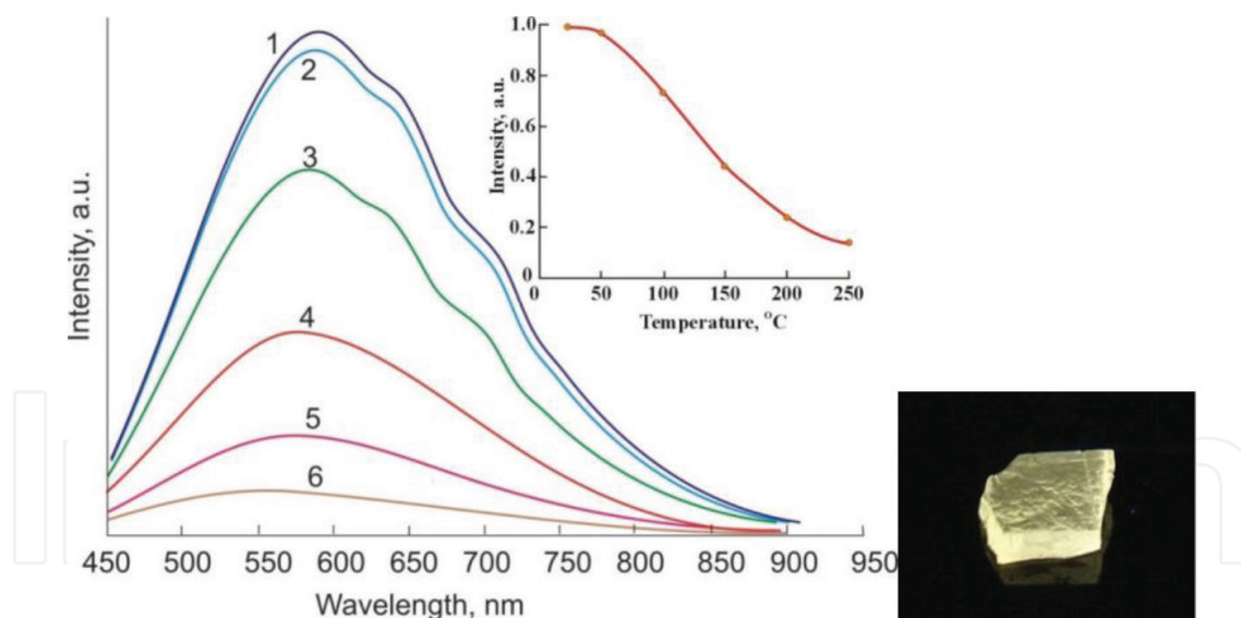
Figure 18. The influence of the temperature of the FP glasses doped with (\text{PbSe})_n MCs on the luminescence intensity... The luminescence spectra were measured at temperature of (1) 22°C, (2) 50°C, (3) 100°C, (4) 150°C, (5) 200°C and (6) 250°C. Excitation wavelength was of 405 nm. Inset: Luminescence intensity in maximum via the temperature of the sample and photo of the luminescence of the FP glass doped with (\text{PbSe})_n MCs.
