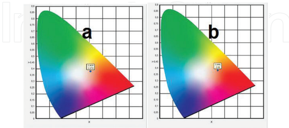
Figure 12. CIE chromaticity coordinates of the FP(CdSe) glass heat treated at T = 405^\circ\text{C} during 30 min (a) and 60 min (b).
