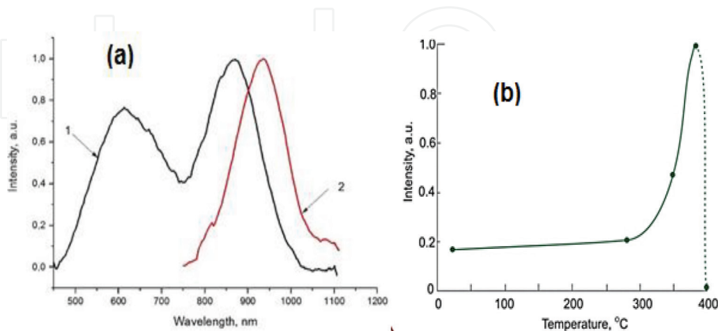
Figure 17. (a) Luminescence spectra of FP glass doped with MCs (\text{PbS})_n after heat treatment at 400^\circ\text{C} within 90 min (1) and 97 min (2), E_{\text{ex}} = 3.06 eV and (b) Luminescence intensity in maximum as a function of thermal treatment temperature.
