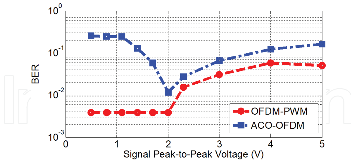
Figure 13. Experimental BER against the peak-to-peak amplitude for 16-QAM OFDM-PWM and ACO-OFDM under the same conditions.
