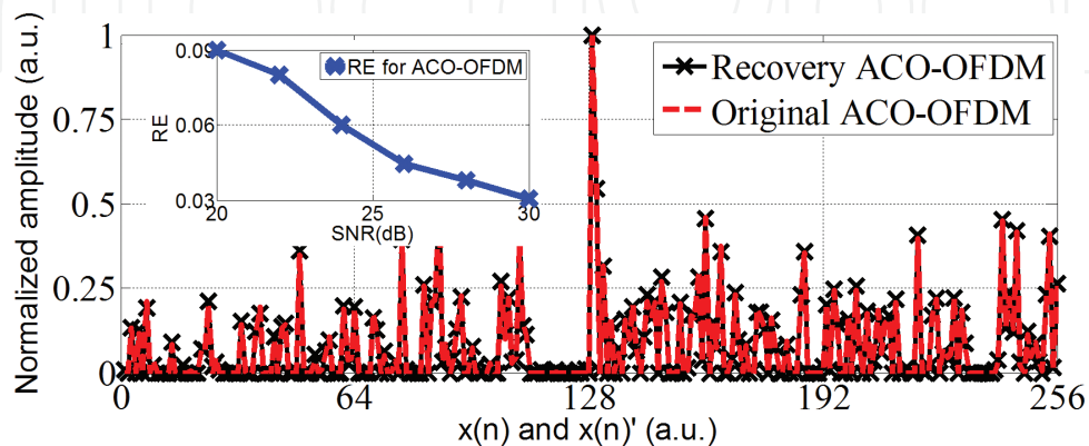
Figure 3. RE analysis for ACO-OFDM (with N = 256 ) for SNR of 30 dB. The inset shows the RE for 20 < \text{SNR} < 30 dB.
