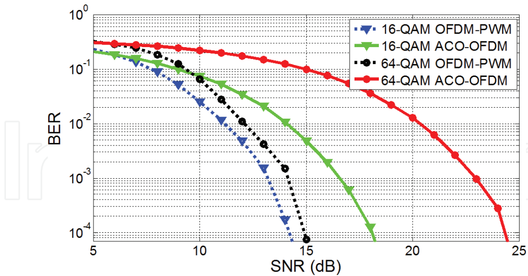
Figure 9. BER performance against the electrical SNR for OFDM-PWM and ACO-OFDM and with 16- and 64-QAM.
