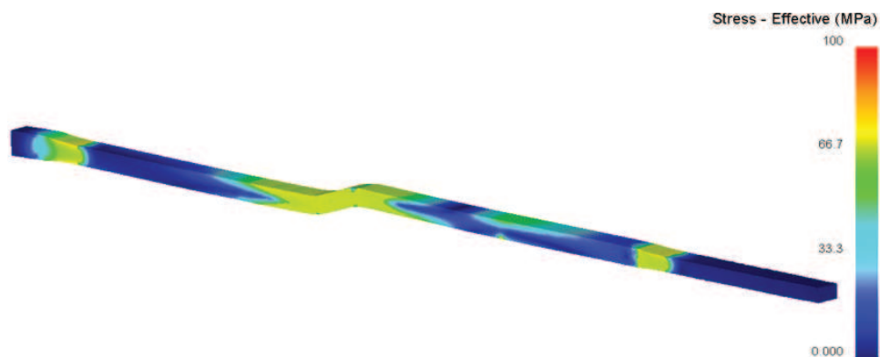
Figure 8. Stress state of the workpiece.
