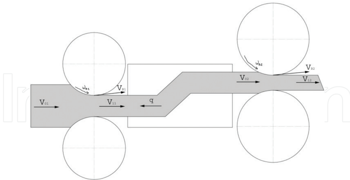
Figure 5. Kinematic diagram of the process "rolling-pressing" with two pairs of rolls.
