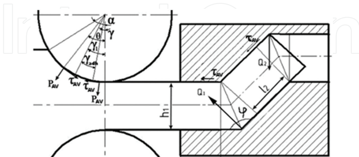
Figure 2. The scheme of forces during deformation.
