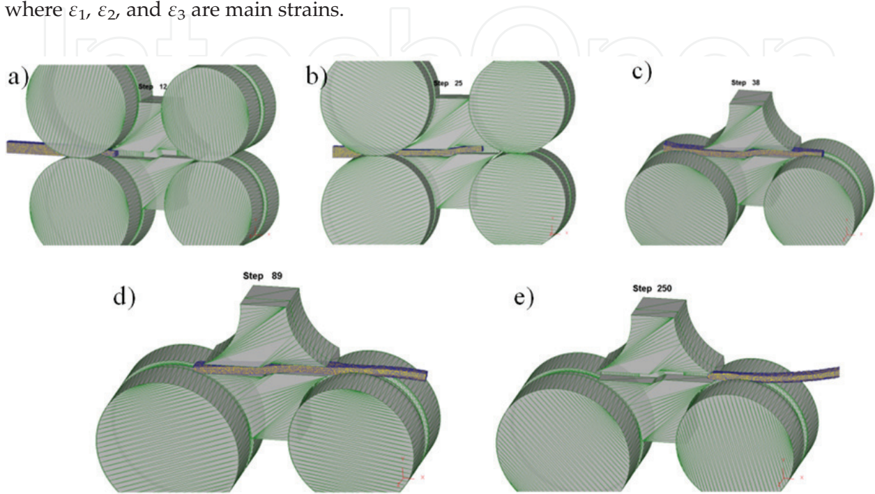
Figure 6. Stage of successful model with calibrated rolls: (a) the workpiece is in the 1 st pair of rolls, (b) the workpiece is in the 1 st pair of rolls and in the matrix, (c) the workpiece is in the both pairs of rolls and in the matrix, (d) the workpiece is in the matrix and in the 2 nd pair of rolls, (e) the workpiece is in the 2 nd pair of rolls.
