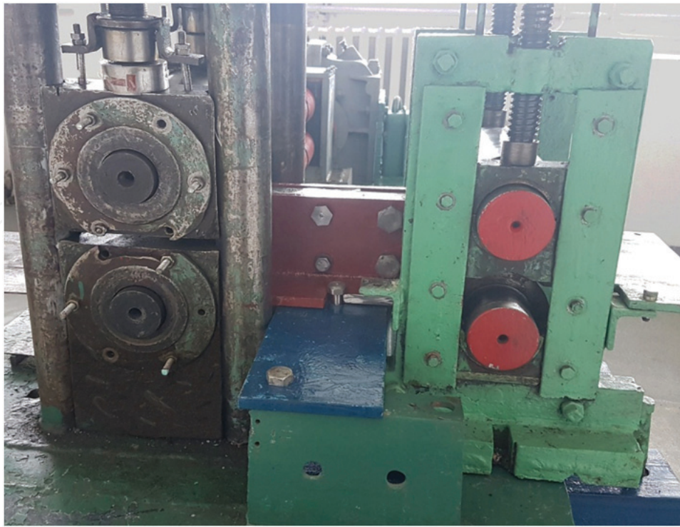
Figure 11. Experimental stand for realization of combined process "rolling-pressing."
