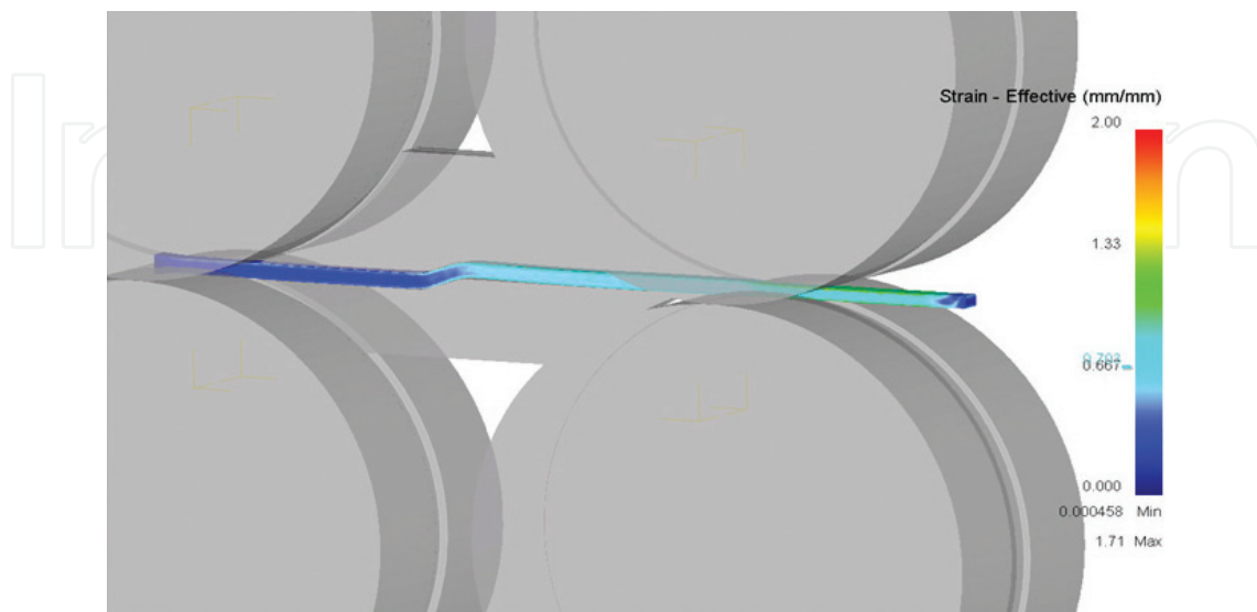
Figure 7. Strain state of the workpiece.
