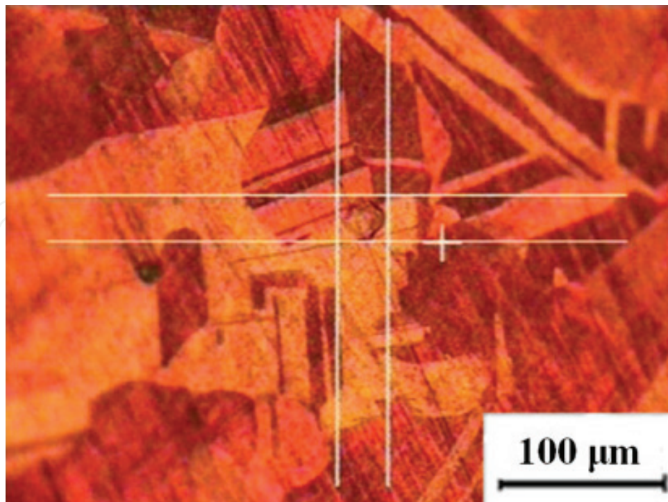
Figure 15. Determination of microhardness of copper.
