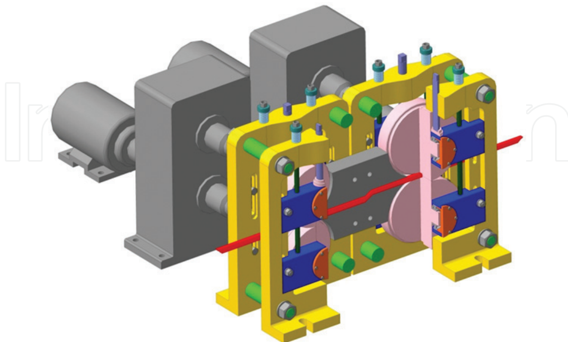
Figure 4. Combined process “rolling-pressing” with two pairs of rolls.
