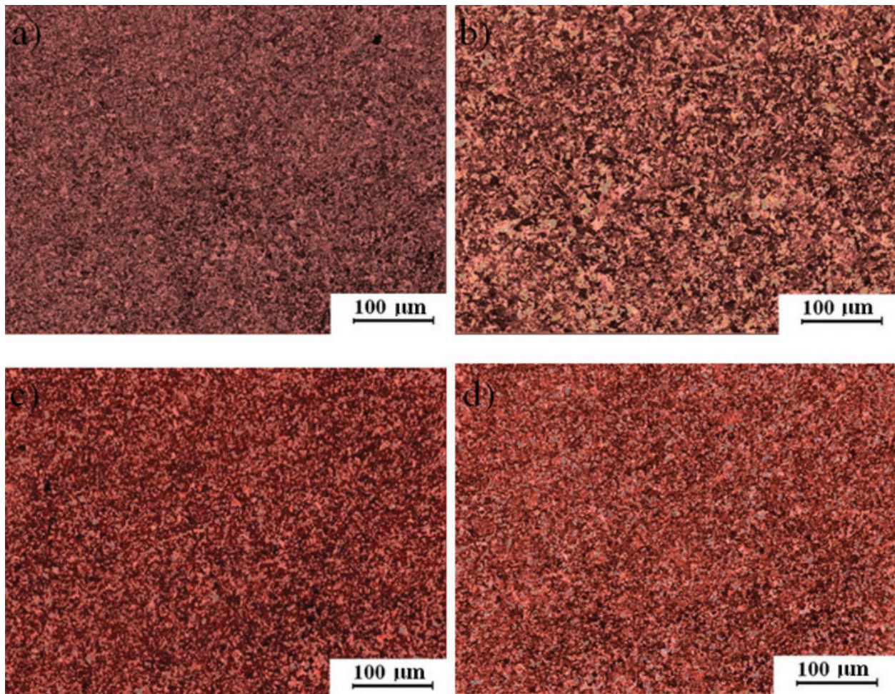
Figure 13. Optical photographs of the microstructure of the copper after three passes of "rolling-pressing" process: (a) initial microstructure, (b) annealing, (c) quenching, and (d) normalizing.
