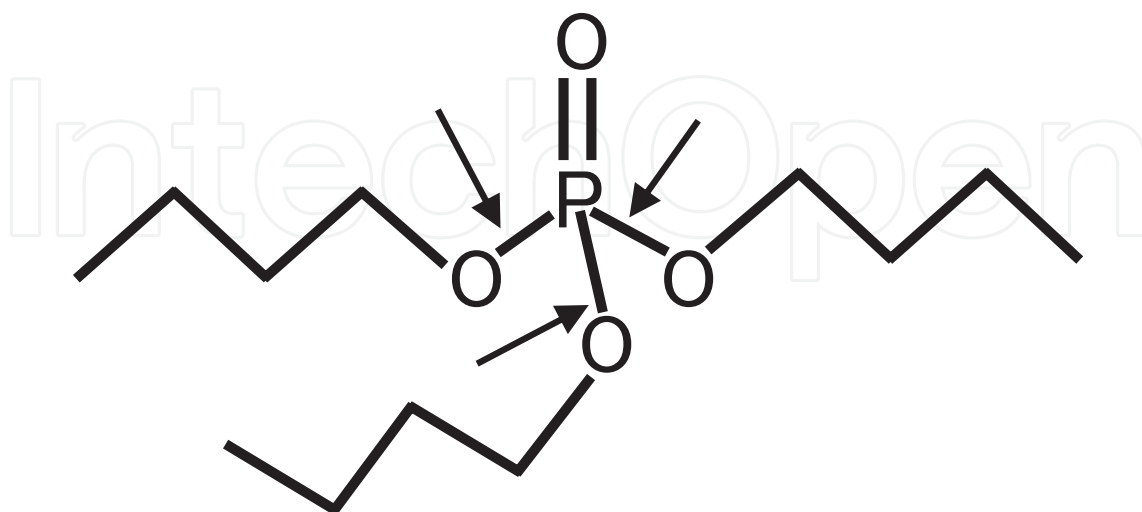
Figure 5. The structure of tributyl phosphate (TBP). Note that, unlike with glycerol 2-phosphate (G2P), three phosphoester bonds (arrowed) require cleavage to yield free inorganic phosphate (Pi) via intermediate DBP. The products would be 1 mol of Pi and 3 mol of butanol. The enzymology is unknown.
