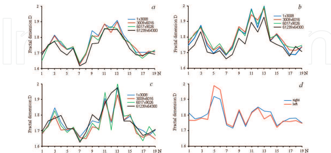
Figure 16. The fractal index D of EEG signals (19 sensors) when the right-handed subjects were random movements: (a) left hand, (b) right hand, (c) both hands, and (d) random movement foot (right, left).
