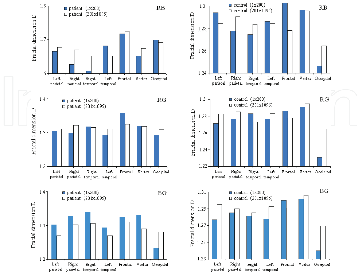
Figure 14. Histogram of the fractal dimension D before and after the red-blue stimulus (RB), red-green (RG), and the blue-green (BG) for the patient MEG signals from the PSE and a group of healthy subjects.
