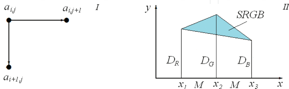
Figure 2. Presentation of experimental data: (I) diagram Hasse and (II) area of triangle in the property frame of references.
