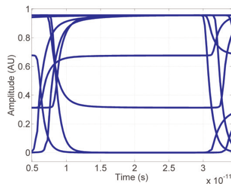
Figure 10. The eye diagram for 4-PAM modulation format and a bit rate of 50 Gb/s, the memory loop length L = 1 km. The signal is at the input of the all-optical memory loop.
