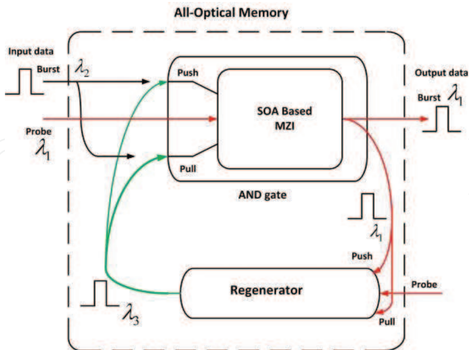
Figure 5. Schematic setup of the all-optical memory based on SOA MZI.
