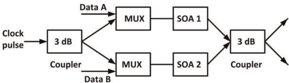
Figure 4. SOA-based MZI.
