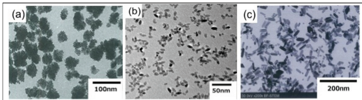
Figure 4. TEM images of nanoparticles of; (a) ZrO_2 (ZR-30AH, Nissan Chemical Industrial Co. Ltd.), (b) TiO_2 with surface deactivation (nanoUSE-TI, Nissan Chemical Industrial Co. Ltd.), and (c) TiO_2 (PST-18NR, JGC-CCIC Co. Ltd.) [11].
