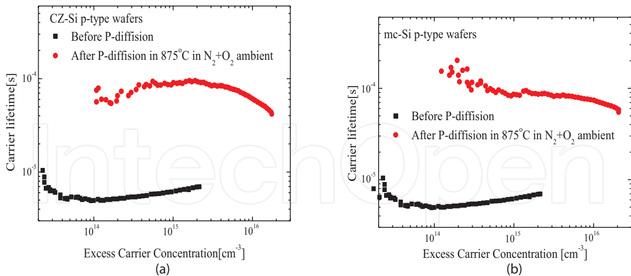
Figure 24. The carrier lifetime as a function of excess carrier concentration in (a) CZ-Si wafers and (b) mc-Si wafer before and after phosphorus diffusion [38].
