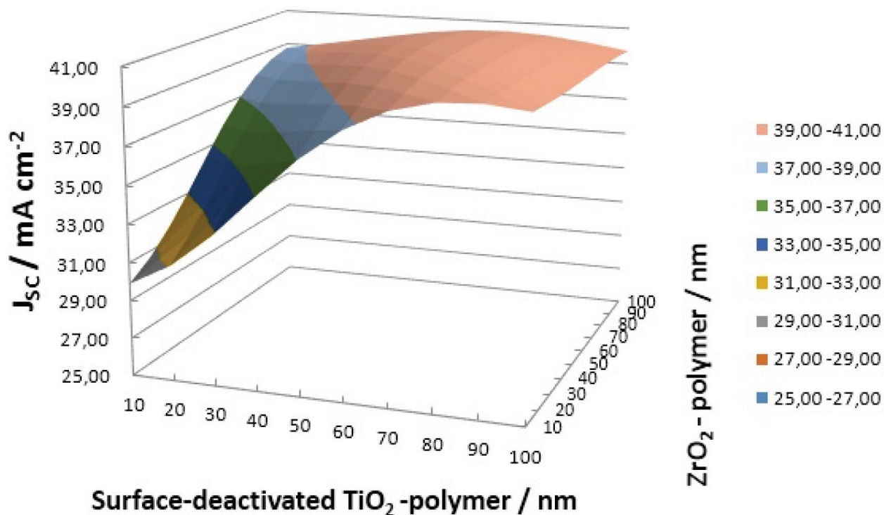
Figure 10. Estimated short-circuit current density with thickness variations of ZrO 2 -polymer and surface-deactivated TiO 2 -polymer films on flat-surface silicon solar cells [11].
