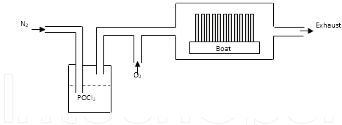
Figure 19. The schematic of \text{POCl}_3 diffusion system.
