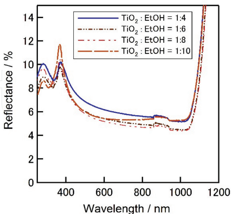
Figure 8. Reflectance spectra of textured silicon surface with surface-deactivated \text{TiO}_2 -polymer antireflection coating [11].
