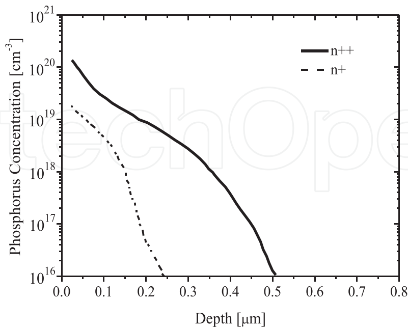
Figure 29. SIMS profiles of highly doped regions under the contacts and out-diffused lowly doped regions between the contacts diffused with the similar profile used for solar cell fabrication at 870^\circ\text{C} for 10 min.
