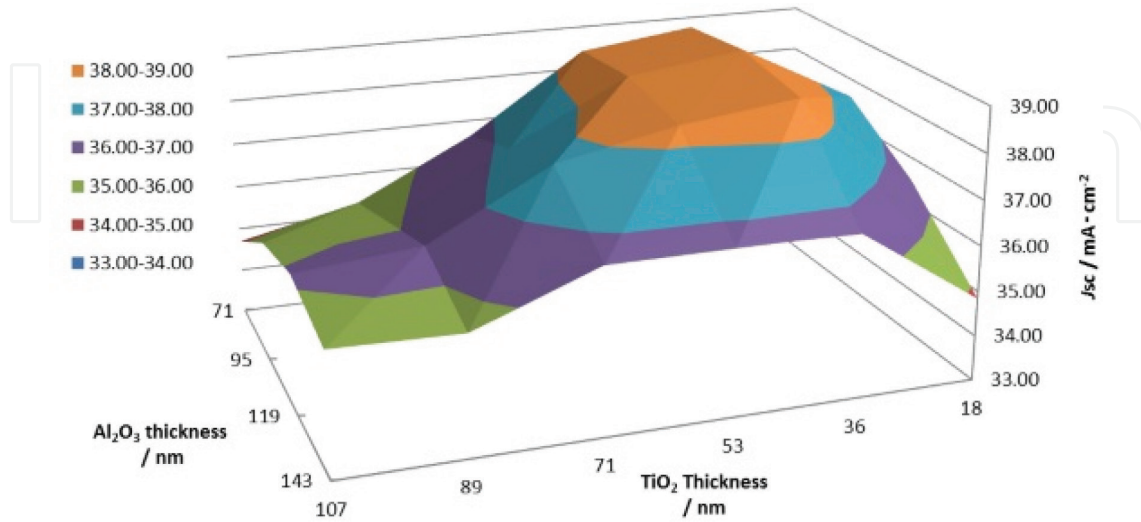
Figure 16. Estimated J_{sc} calculated by the experimental reflectivity data using (Al_2O_3/TiO_2/Si) layers with various thicknesses of Al_2O_3 and TiO_2 films [21].
