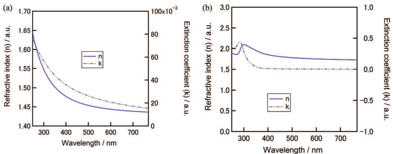
Figure 9. Fitting of ellipsometry measurements of (a) nano-colloid ZrO_2 (ZR30-AH)-polymer composite and (b) surface-deactivated TiO_2 -polymer composite [11].
