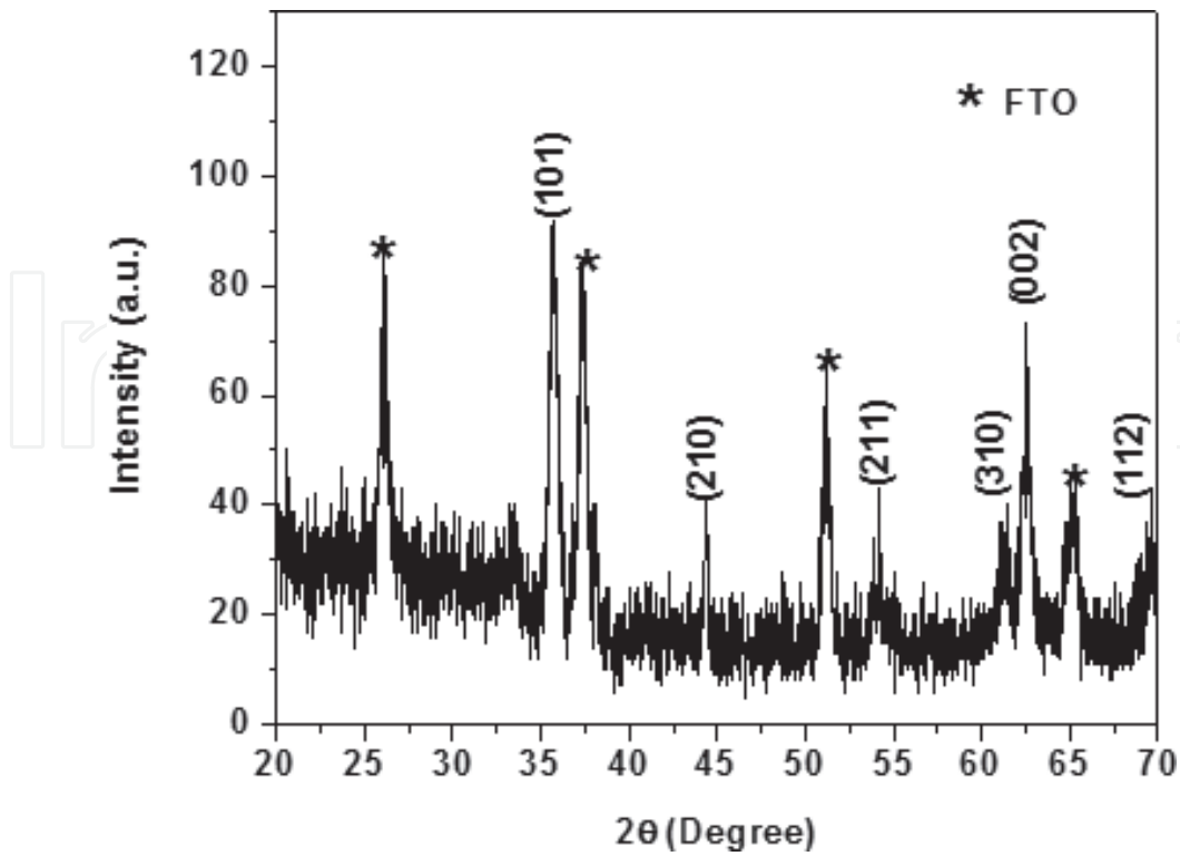
Figure 7. XRD pattern of the rutile-phased TNAs [25].
