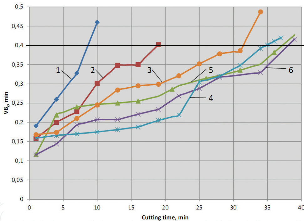
Figure 1. Dependence of wear VB on cutting time at dry turning of steel C45 at a_p = 1.0 mm; f = 0.2 mm/rev; v_c = 250 m \text{min}^{-1} . 1 – Uncoated; 2 – TiN; 3 – Cr-CrN-(TiCrAl)N; 4 – Zr-ZrN-(NbZrTiAl)N; 5 – Zr-ZrN-(ZrCrAl)N; 6 – Ti-TiN-(ZrNbTi).
