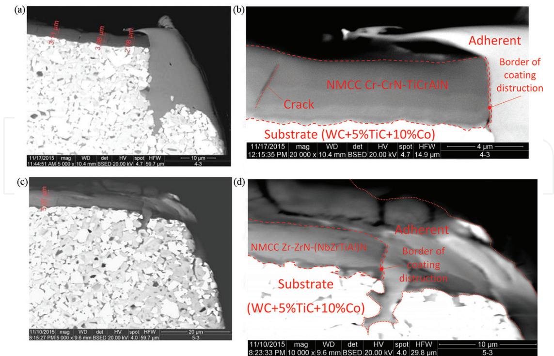
Figure 6. Examples of failure of coating and substrate because of breaking along the formed longitudinal crack. NMCC Cr-CrN-TiCrAlN (a, b); Zr-ZrN-(NbZrTiAl)N (c, d) [34].
