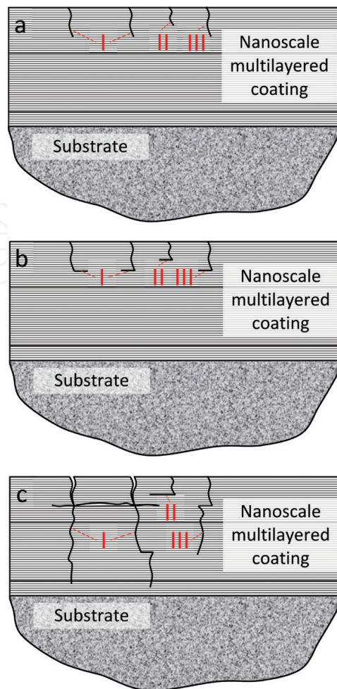
Figure 7. Stages of formation of a cross crack, transforming into a longitudinal crack (delamination) in multilayered nanostructured coating: (a) initiation of a crack, (b) transformation of a cross crack into a longitudinal crack (delamination); (c) creation of a through longitudinal crack between two cross cracks; (d) a tear-out or chipping of a coating segment between two cross cracks.
