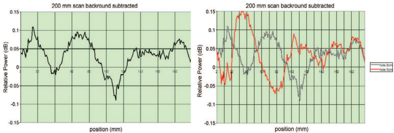
Figure 7. Relative power scan of a sample with a hole and when two holes were filled alternately ( f = 6 GHz). The second hole was drilled 3 cm away from the first one [15] (Reproduced with permission of ELSEVIER S.A. via Copyright Clearance Center).
