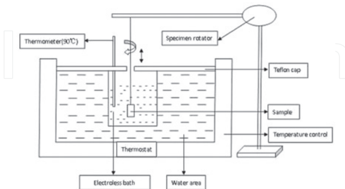
Figure 1. Basic illustration of the apparatus used in electroless coating experiments.
