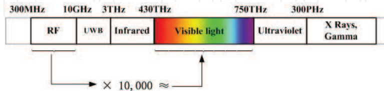
Figure 1. The electromagnetic spectrum.
