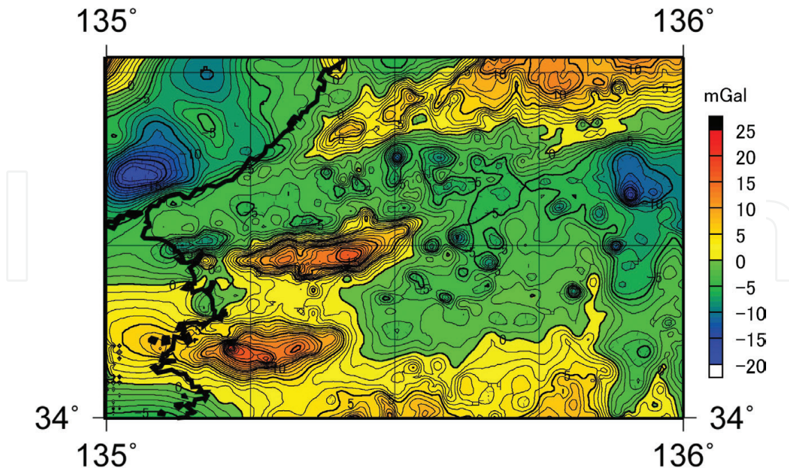
Figure 2. Residual Bouguer anomaly map of the study area and surroundings. The contour interval is 1 mGal. In the residual Bouguer anomaly map, the regional linear trend of the Bouguer anomalies, such as the effect of the subducting plate, is estimated and removed by the least-squares method from the Bouguer anomalies. The Bouguer anomaly used here is based on the gravity anomaly database (0.5 km \times 0.5 km mesh data) by Komazawa [19], and a Bouguer density of 2670 kg/m 3 is employed.
