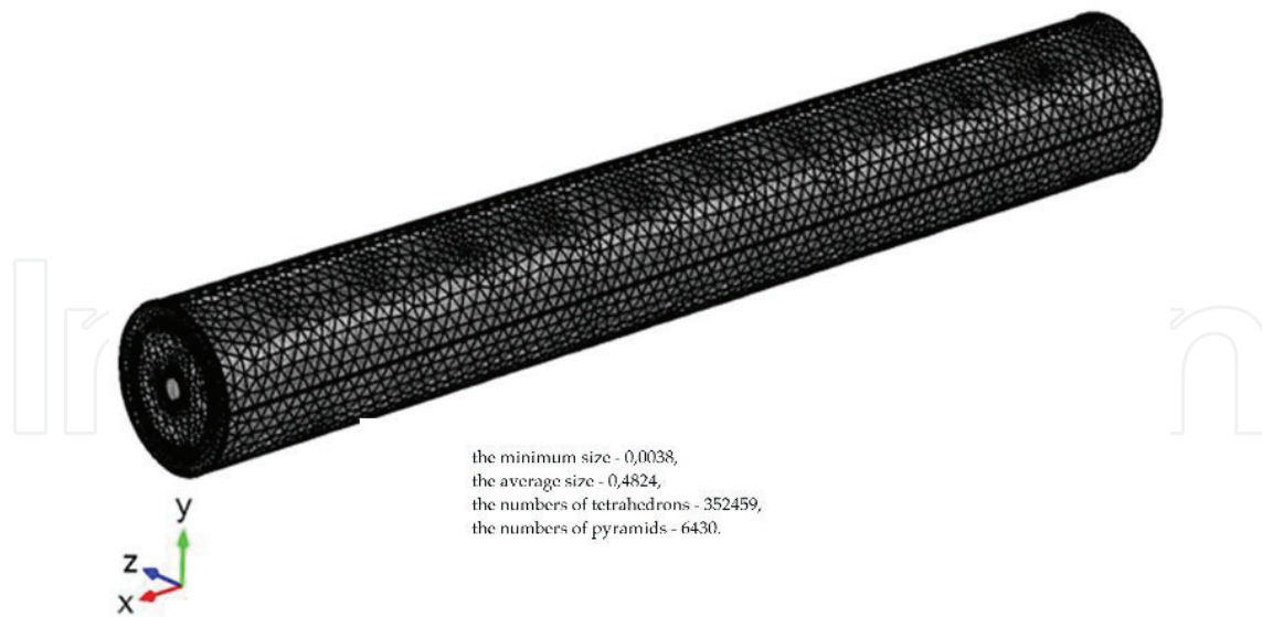
Figure 2. Calculation mesh.
