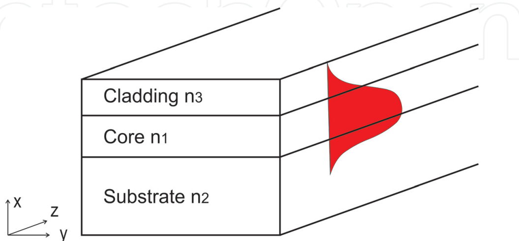
Figure 1. A three-layer configuration of a slab optical waveguide.
