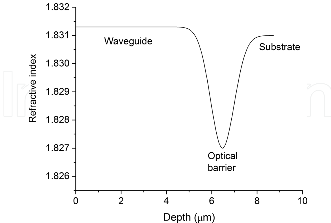
Figure 5. A refractive index profile of a Yb:YAG waveguide implanted with protons at an energy of 1 MeV and an incident angle of 46° [27].
