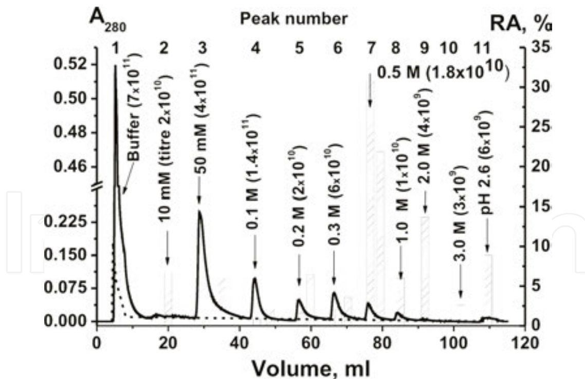
Figure 10. Affinity chromatography of phage particles on DNA-cellulose: (—) and (---), A 280 values correspond respectively to the material of phage particles containing or not cDNA of kappa light chains [111]. The bars show the RAs of 16 fractions of 11 peaks eluted with various concentrations of NaCl and acidic buffer (pH 2.6). The titres of the particles of different peaks are given in the parenthesis.
