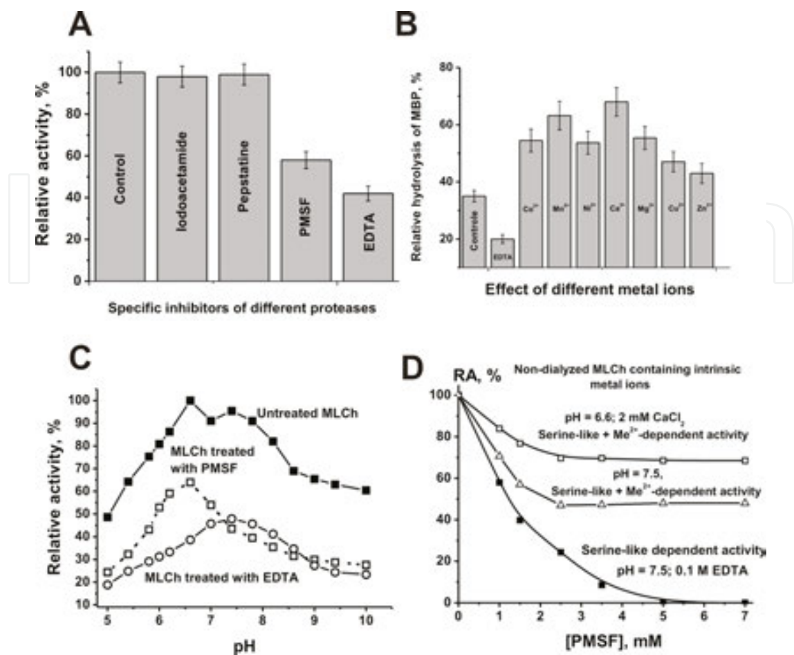
Figure 23. The RAs of the activity of NGTA2-Me-pro-Tr in the hydrolysis of MBP after its preincubation with specific inhibitors of different type proteases (A) [119]. MLCh (0.3 mg/ml) was preincubated alone (control), or the presence of iodoacetamide, PMSF, pepstatin, or EDTA; 1.0 \mu l of this mixture was added to 29 \mu l of MBP-containing standard reaction mixtures (A). The relative activity of NGTA2-Me-pro-Tr after preincubation with without different inhibitors (control) was taken for 100%. Effects of 10 mM EDTA and various Me 2+ ions (2 mM) on the RAs of MLCh are shown (B). Dependences of the relative proteolytic activity of NGTA2-Me-pro-Tr before and after its treatment with PMSF and EDTA upon pH of reaction mixtures are shown (C). Dependence of the MBP-hydrolyzing activity on concentration of CaCl 2 at pHs 6.0 and 8.5 (D).
