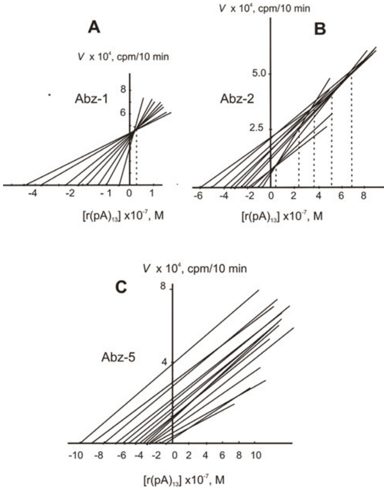
Figure 9. Initial rates of [5'\text{-}^{32}\text{P}](\text{pA})_{13} hydrolysis as a function of oligonucleotide concentration for three SLE IgGs [71]. The K_m and V_{max} values were determined using the Cornish-Bowden coordinates (A–C). The common intersection points give K_m and V_{max} values characterizing different abzymes; the absence of intersection points indicates that many different monoclonal abzymes with similar and different kinetic parameters catalyze the oligonucleotide hydrolysis.
