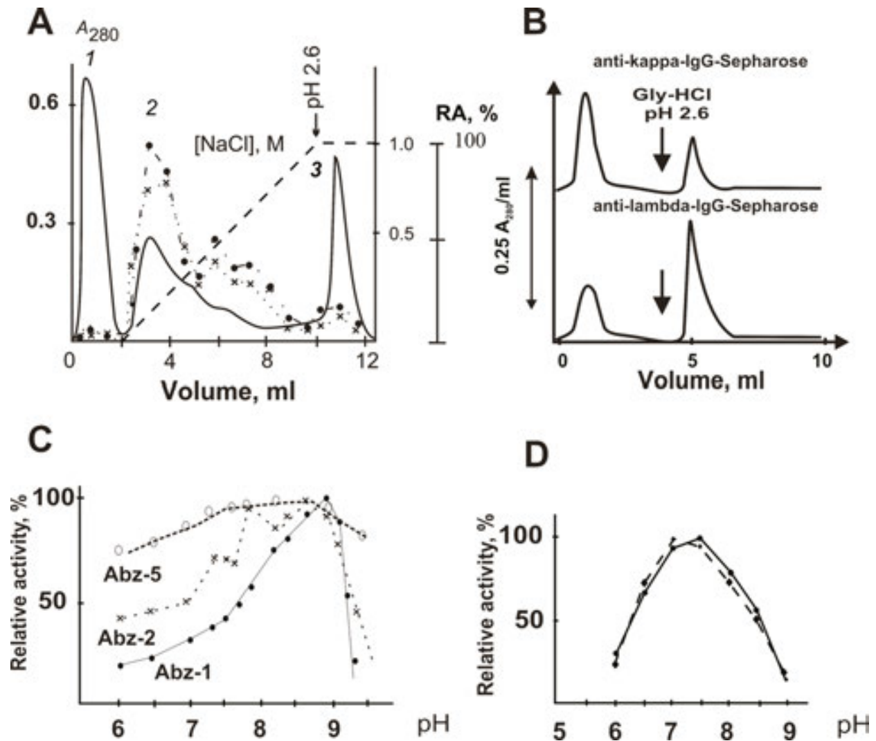
Figure 8. Separation of SLE IgMs having affinity to DNA by affinity chromatography on DNA-cellulose (A) [70]: (—) absorption at 280 nm, (•) and (x) RA of Abs in hydrolysis of respectively [5'-^{32}\text{P}](\text{pA})_{13} and [5'-^{32}\text{P}]\text{d}(\text{pA})_{13} , 1–5 \mu\text{l} of each fraction was added to 100 \mu\text{l} of reaction mixture and maximal RNase and DNase activity was taken for 100%. Separation of anti-DNA IgGs containing light chains of kappa and lambda type by affinity chromatography on Sepharoses bearing immobilized Abs against human kappa- and lambda-IgGs [71]: (—) absorption at 280 nm (B). pH dependencies of the relative RNase activity of three SLE IgGs (C) and human serum RNases (RNase 3 (•) and RNase 4 (•)) (D) in the hydrolysis of [5'-^{32}\text{P}](\text{pA})_{13} [71].
