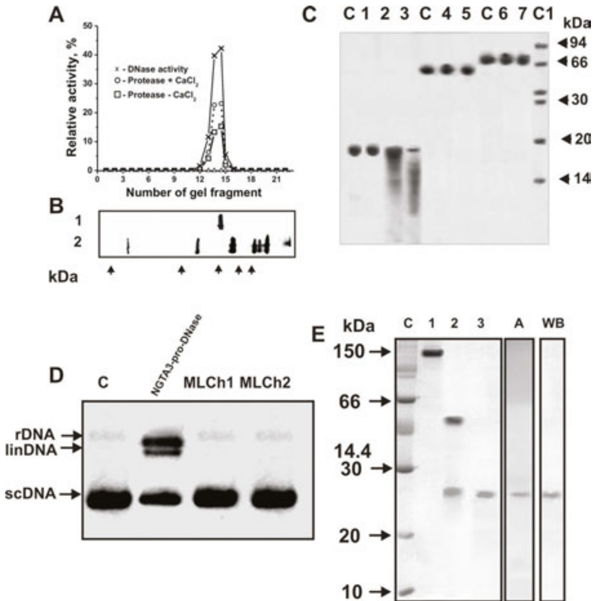
Figure 24. SDS-PAGE analysis of MBP- and DNA-hydrolyzing activities (A) and homogeneity of NGTA3-pro-DNase (7 \mu g) using a reducing 5–16% gradient gel followed by silver staining (B, lane 1); the arrows (B, lane 2) indicate the positions of protein markers. After SDS-PAGE the gel was incubated using conditions for renaturation of NGTA3-pro-DNase. The relative MBP- and DNA-hydrolyzing activity (%) was revealed using the extracts of 2- to 3-mm gel fragments (A). The activity of NGTA3-pro-DNase corresponding to a complete hydrolysis of 0.5 mg/ml MBP (or 18 nM scDNA) after 24 h of incubation of 25 \mu l reaction mixture containing 10 \mu l of the gel extracts was taken for 100%. SDS-PAGE analysis of hydrolysis of MBP by inact-MLChmix (lane 1) or NGTA3-pro-DNase (lanes 2 and 3, different time of incubation) (C). Hydrolysis of control proteins (0.5 mg/ml) by inact-MLChmix and NGTA3-pro-DNase was analyzed: human albumin (lanes 4 and 5) and lactoferrin from human milk (lanes 6 and 7) (C). The mixtures were incubated for 6 h with inact-MLChmix (lanes 4 and 6), or NGTA3-pro-DNase (lanes 5 and 7). All lanes C correspond to different proteins incubated alone without MLChs, while lane C1- to standard protein markers. DNase activity of NGTA3-pro-DNase and two control MLCh1 and MLCh2 (10 nM) was analyzed in the presence of 5 mM MgCl 2 (D); lane C corresponds to scDNA incubated alone. In situ assay of DNase activity of the NGTA3-pro-DNase (8 \mu g) after treatment with DTT (lane A) (E). DNase activity was revealed by ethidium bromide staining as a dark band on the fluorescent background. A part of the gel was stained with Coomassie R250 to show the position of the SLE IgGs before (lane 1) and after incubation with DTT (lane 2), as well as NGTA3-pro-DNase (lane 3) (E). MLCh was analyzed by Western blotting to a nitrocellulose membrane using mouse IgGs against light chains of human Abs conjugated with horseradish peroxidase (lane WB) (E).
