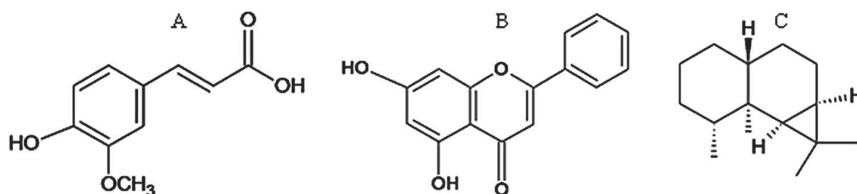
Figure 7. Chemical structures of some flavonoids found in Russula mushrooms. A = ferulic acid, B = chrysin, C = aristolane.
