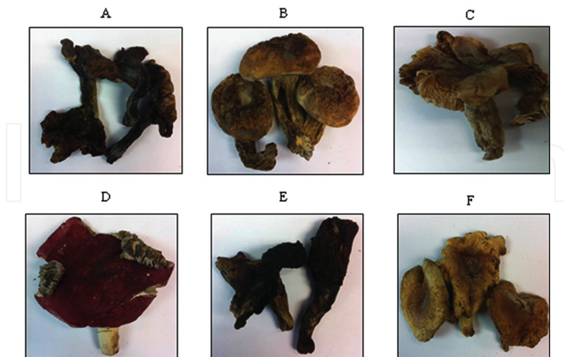
Figure 6. Physical characteristics of some Russula mushrooms found in Thailand; A = Russula crustosa Peck, B = Russula delicata Fries, C = Russula monspeliensis Sarnari, D = Russula velenovskyi Melzer & Zvára, E = Russula virescens (Schaeff) Fries, F = Russula alboareolata Hongo.
