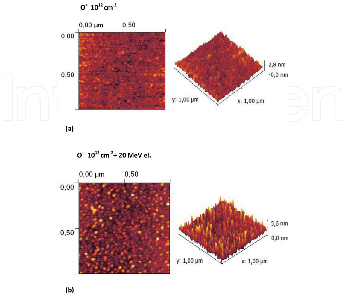
Figure 12. Si-SiO 2 sample implanted with O + ions (dose of 10 12 cm -2 ) before (a) and after (b) MeV electron irradiation.
