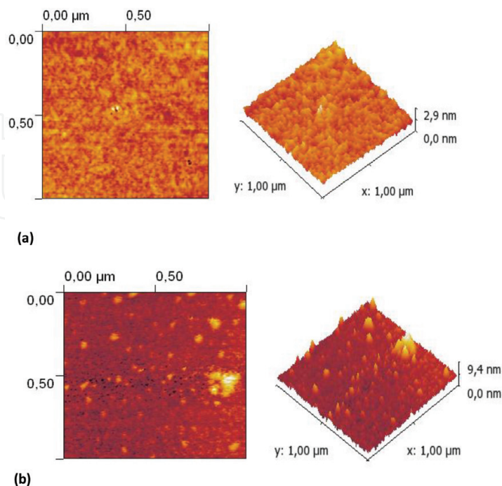
Figure 11. Surface morphology of Si-SiO 2 sample before (a) and after electron irradiation (b).
