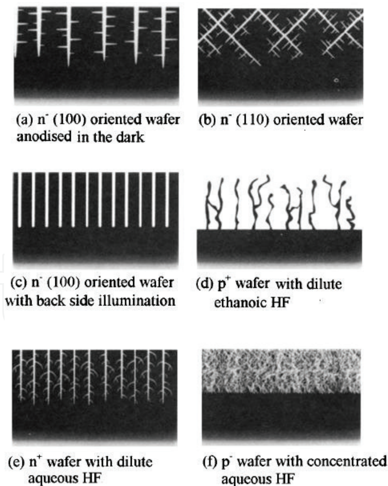
Figure 9. Illustration of pore formation based on dopant factor [22].
