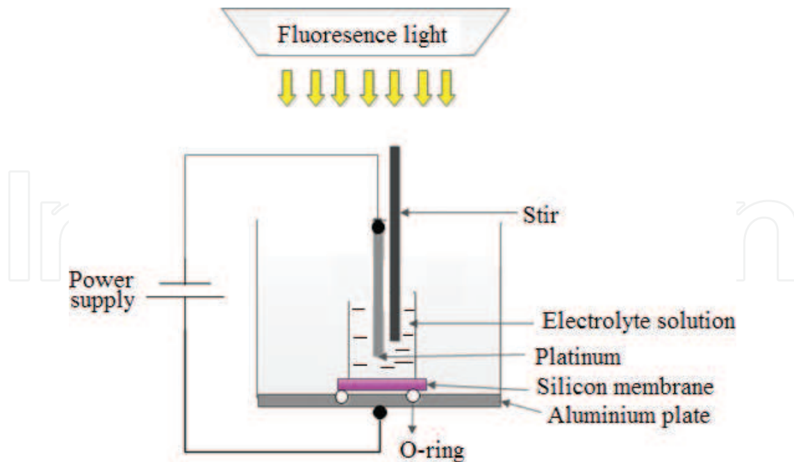
Figure 15. Electrochemical etching process.
