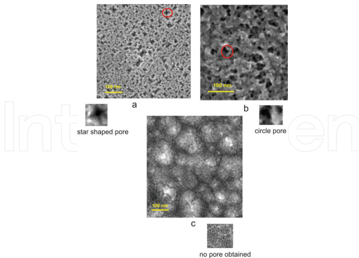
Figure 25. The pore structure for the mixture of HF + methanol as electrolyte solution: (a) undoped, (b) n-type (c) p-type.
