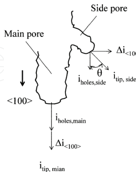
Figure 8. Forming a hole caused by the formation of a new model of current eruption which dissolves holes in different orientations [39].
