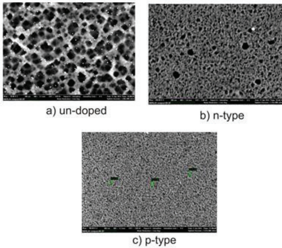
Figure 23. Shape of porous on different doping.
