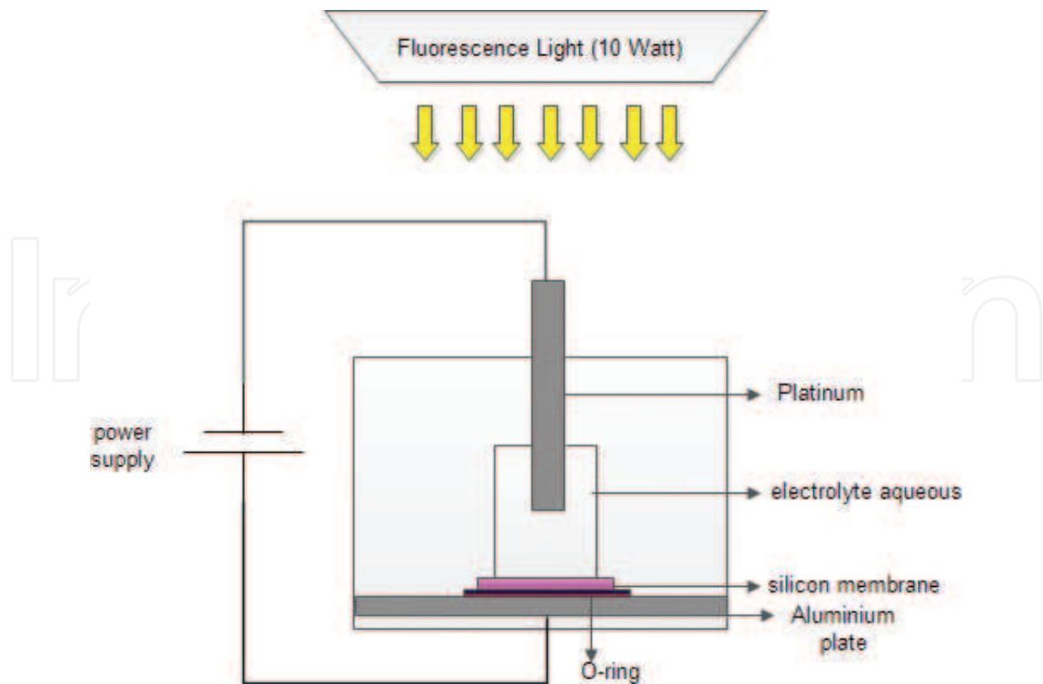
Figure 2. Cross section of a conventional single-tank cell [27].
