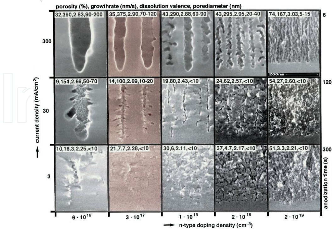
Figure 22. Scanning electron micrographs of porous silicon for n-type doped <100> silicon [19].
