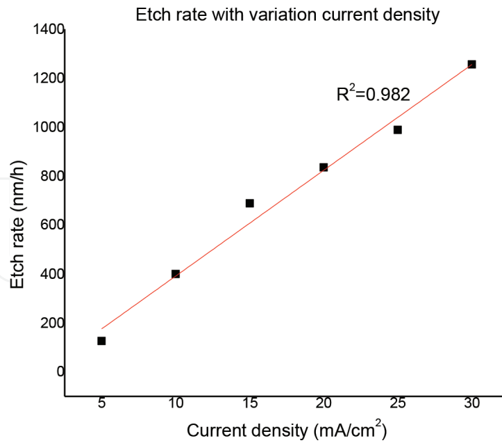
Figure 19. Correlation between the porous layer etching rate and current density in ethanoic HF solution.
