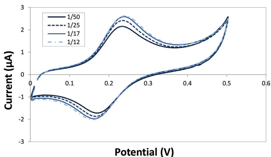
Figure 4. Cyclic voltammograms of diluted pomace extracts.
