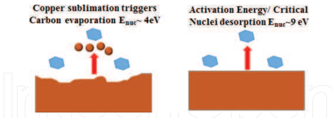
Figure 4. Activation energy differ for low and atmospheric pressure CVD. At low pressure, evaporation of Cu is significant which limits nucleation of graphene ( E_{nuc} \sim 4\text{ eV} ). Cu evaporation is less at atmospheric pressure CVD, where nucleation activation energy is higher ( E_{nuc} \sim 9\text{ eV} ). [Reprinted with permission from Ref. [45].
