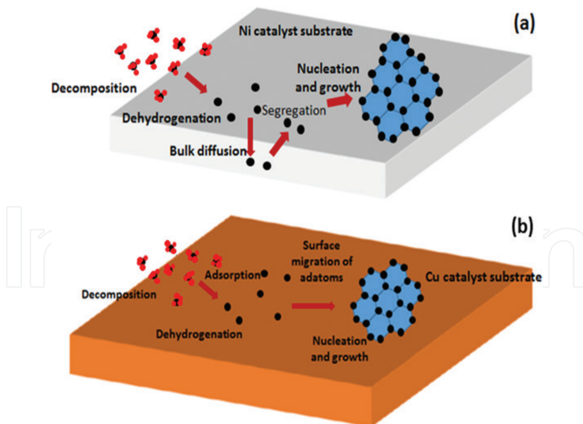
Figure 5. (a) Graphene growth process on highly carbon soluble metal substrate (e. g., Ni). Decomposition, dehydrogenation, bulk diffusion, and segregation process determined the graphene nucleation and growth. (b) Graphene growth process on a low carbon soluble metal substrate (e.g., Cu). Decomposition, dehydrogenation, and surface adsorption/desorption process determined the graphene nucleation and growth.
