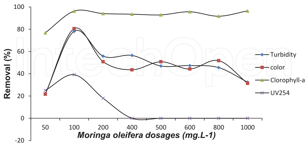
Figure 1. Color, turbidity, compounds with absorption in UV_{254\text{nm}} and chlorophyll-a removal in relation to the dosage of Moringa oleifera powder seeds for Anabaena flos-aquae .
