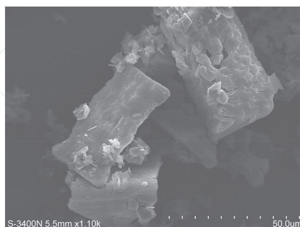
Figure 1. The SEM figure of magnesium ammonium phosphate crystal.
