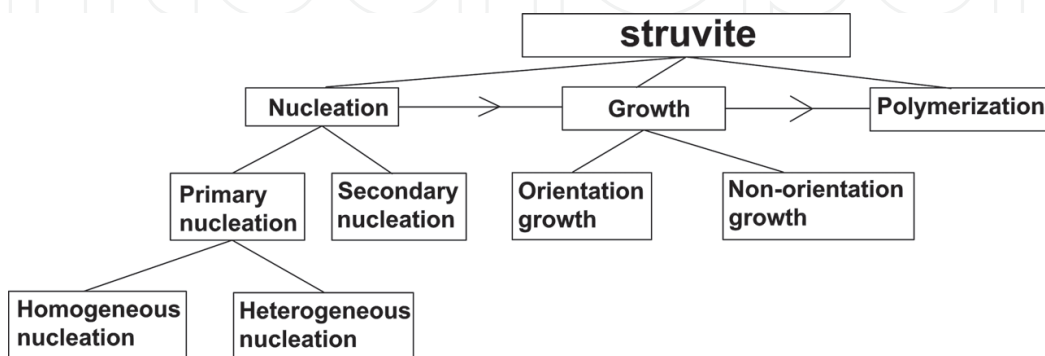
Figure 2. The crystal nucleation, growth and aggregation mechanism of magnesium ammonium phosphate.
