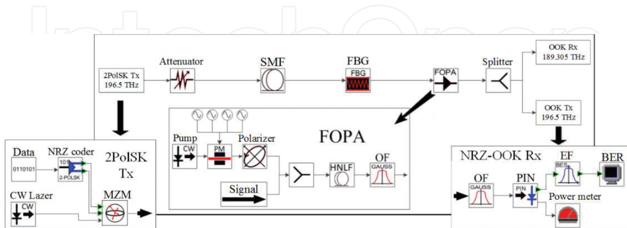
Figure 15. Simulation model of the single-channel transmission system, where a single-pump FOPA with linearly polarized pumping radiation is used for 2PolSK to NRZ-OOK modulation format conversion.
