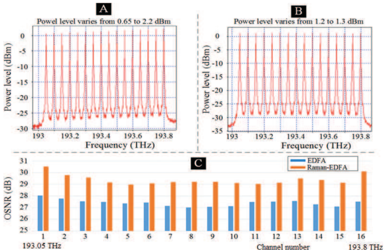
Figure 6. Signal spectra at the output of the EDFA (A) and at the output of the hybrid Raman-EDFA amplifier (B) and OSNR comparison among all 16 channels in the system with the EDFA in-line amplifier and the hybrid Raman-EDFA amplifier (C).
