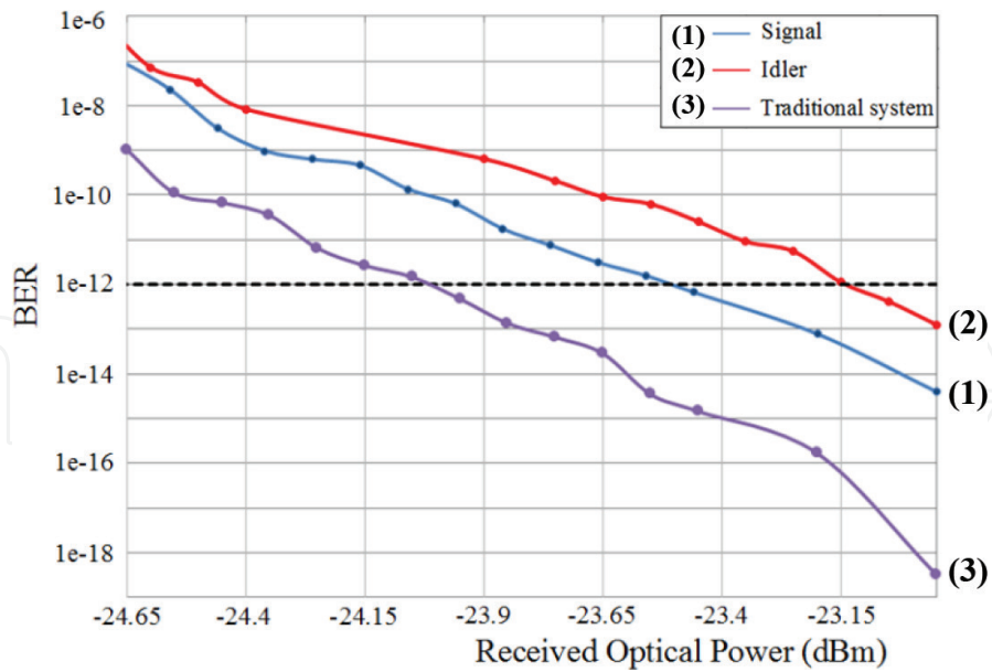
Figure 20. BER value dependence on the detected signal power in the standard eight-channel transmission system (3) and in the fifth channel on the second branch of the multichannel system with modulation format conversion at the initial signal frequency (1) and idler frequency (2).
