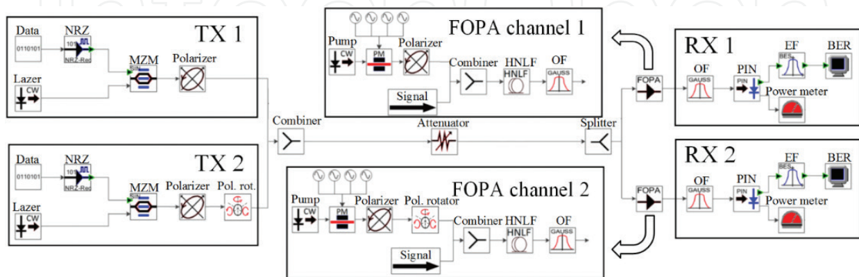
Figure 21. Simulation model of the two-channel optical transmission system with FOPA for division and amplification of polarization-multiplexed signals.
