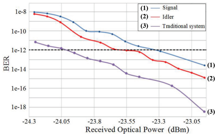
Figure 23. BER value dependence on the power of the detected signal in the standard single-channel system (3) and in the first channel of the system with the chosen FOFA configuration of the signal at its initial frequency (1) and of the idler (2).
