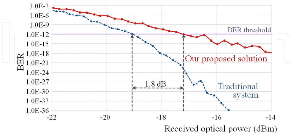
Figure 14. BER value dependence on the power of the detected signal for the 12th channel ( f=192.55 THz; \lambda = 1557 nm) in the system with the proposed multicarrier source solution (solid line) and in the system with traditional architecture (dashed line).
