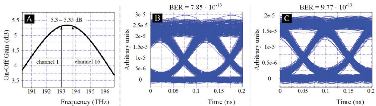
Figure 8. DRA produced gain spectrum (A) and eye diagrams of the ninth channel in the system with the SOA in-line amplifier (B) and the tenth channel in the system with the Raman-SOA hybrid amplifier (c).
