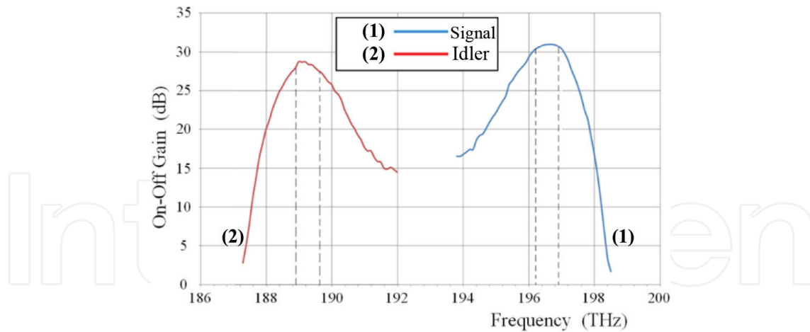
Figure 19. Gain spectrum ensured by the FOPA with 790 mW 1554.15 nm linearly polarized pumping radiation at initial signal frequencies (1) and idler frequencies (2).
