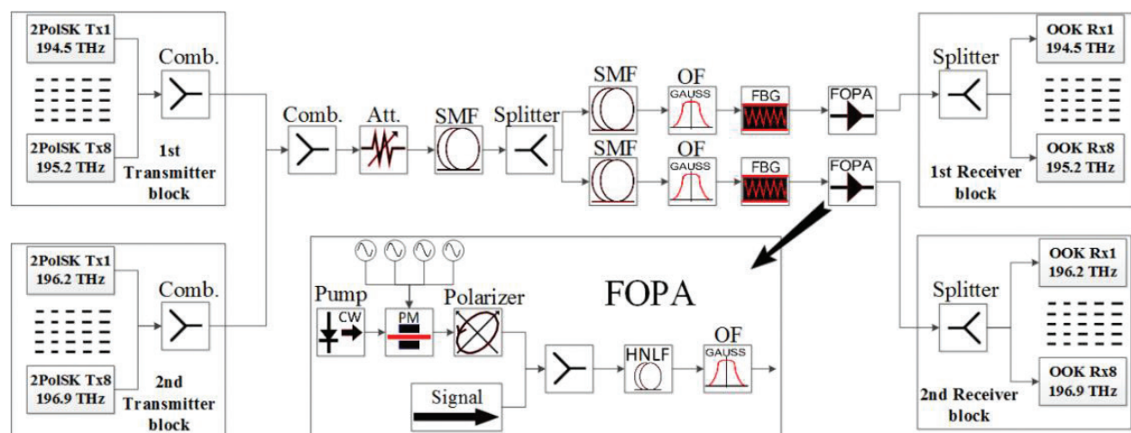
Figure 18. Simulation model of the 16-channel WDM transmission system with two access network branches, where in each branch the FOPA preamplifier is used for 2PolSK to NRZ-OOK (on-off keying) modulation format conversion.
