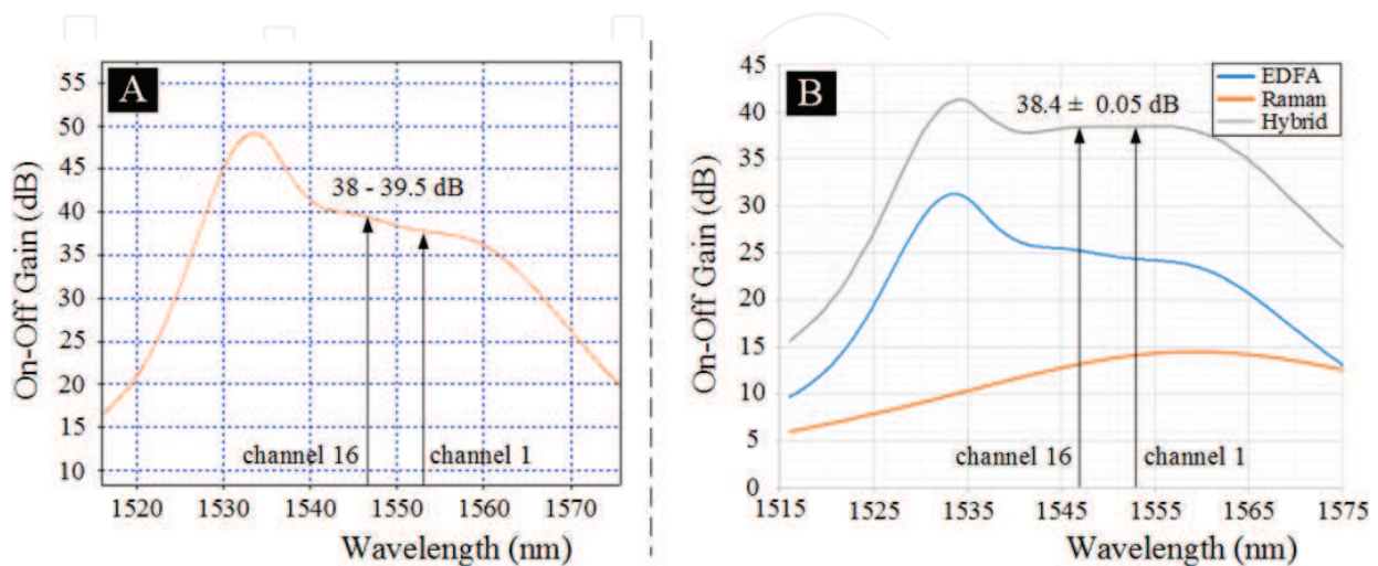
Figure 5. Gain spectra of the EDFA in-line amplifier (A) and of the hybrid Raman-EDFA amplifier (B).
