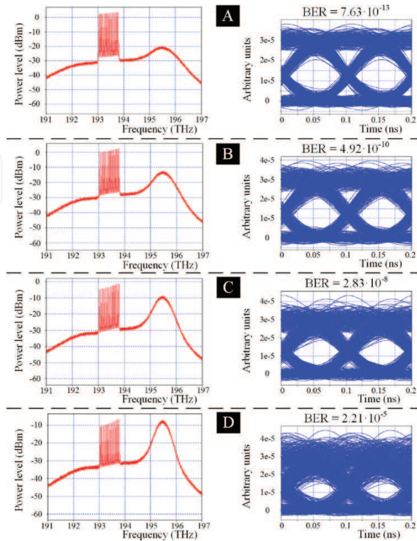
Figure 3. Optical spectra (the power level depending on frequency) at the output of the EDFAs (to the left) and eye diagrams of the signal detected in the ninth channel (to the right) after first (A), second (B), third (C), and fourth (D) stages of amplification.
