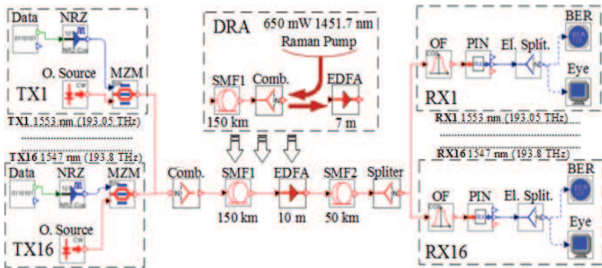
Figure 4. Simulation model of the 16-channel 10 Gbps DWDM transmission system with an EDFA in-line amplifier or with a hybrid Raman-EDFA amplifier.
