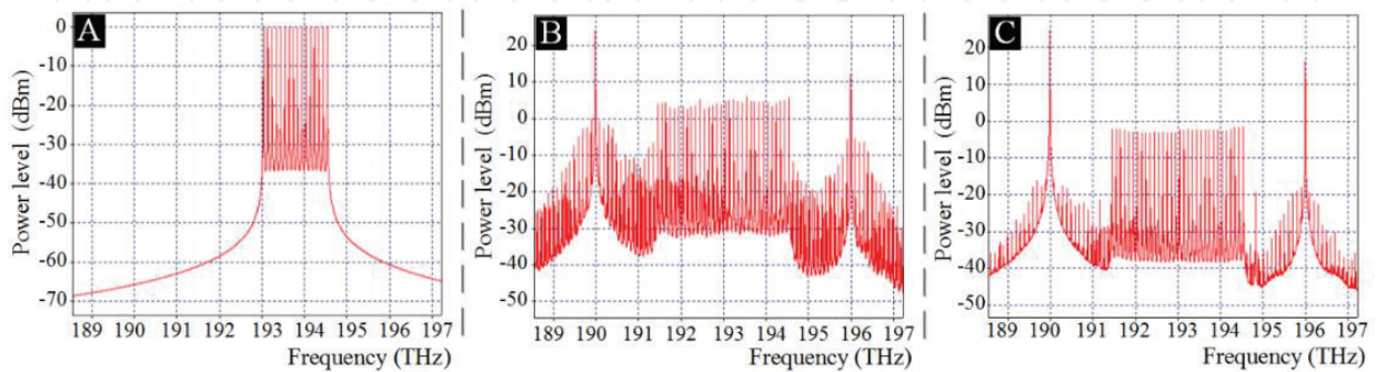
Figure 13. Optical spectrum at the input of the FOPA when initial carrier power is set to 0 dBm (A) and optical spectra at the output of the HNLF when the power of the initial carriers is set to 0 dBm (B) and to -10 dBm (C).
