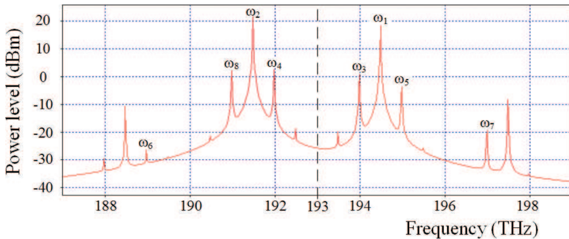
Figure 11. Optical spectrum at the output of a dual-pump FOPA with 200 mW 191.5 THz pumps and 500 meter long HNLF.
