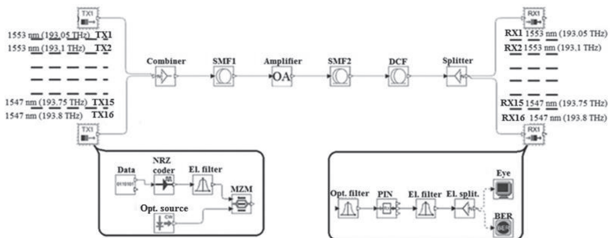
Figure 2. Simulation model of the 16-channel 10 Gbps DWDM transmission system used for comparison of optical amplifier performance.
