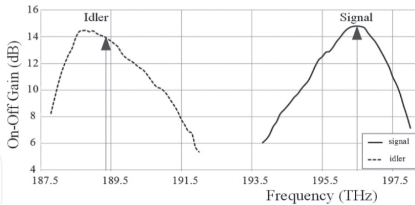
Figure 16. Gain spectrum produced by the single-pump FOPA with linearly polarized pumping radiation at signal frequencies (solid line) and at idler frequencies (dotted line).
