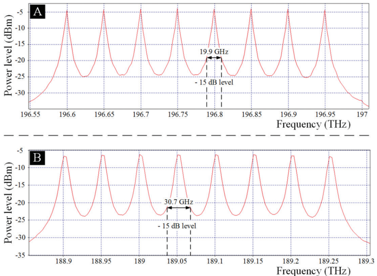
Figure 10. Spectra of the amplified signal (A) and the generated idlers (B) at the output of the single-pump FOPA.
