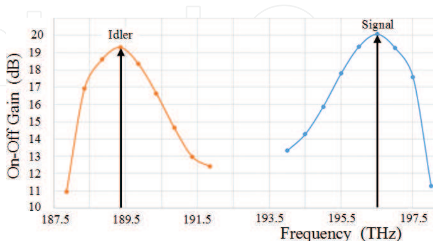
Figure 22. FOPA produced on-off gain for the first channel at idler frequencies (left side) and at the initial signal frequencies (right side).
