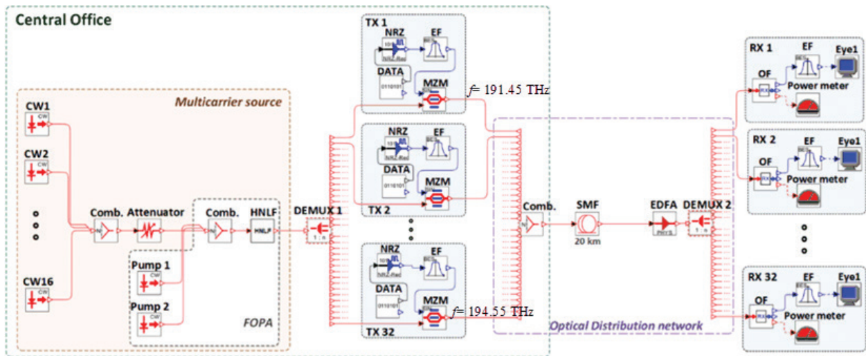
Figure 12. Simulation model of the 32 channel 10 Gbps WDM transmission system with the provided multicarrier source solution, which is based on wavelength conversion using a dual-pump FOPA.
