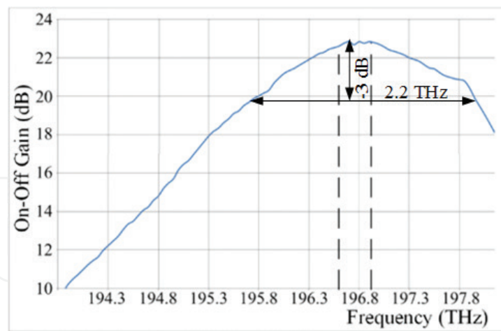
Figure 9. Gain spectrum of the single-pump FOPA with 660 mW 1553.9 nm pumping radiation.
