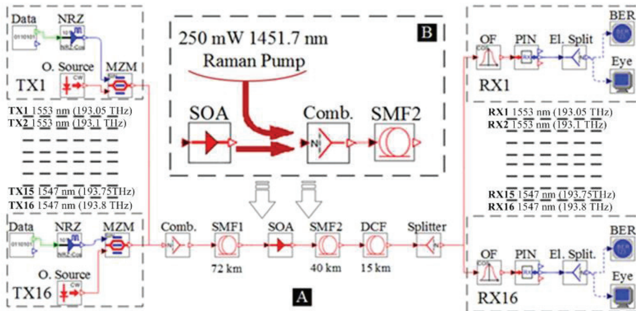
Figure 7. Simulation model of the 16-channel 10 Gbps DWDM transmission system with the SOA in-line amplifier (A) or with a hybrid Raman-SOA amplifier (B).
