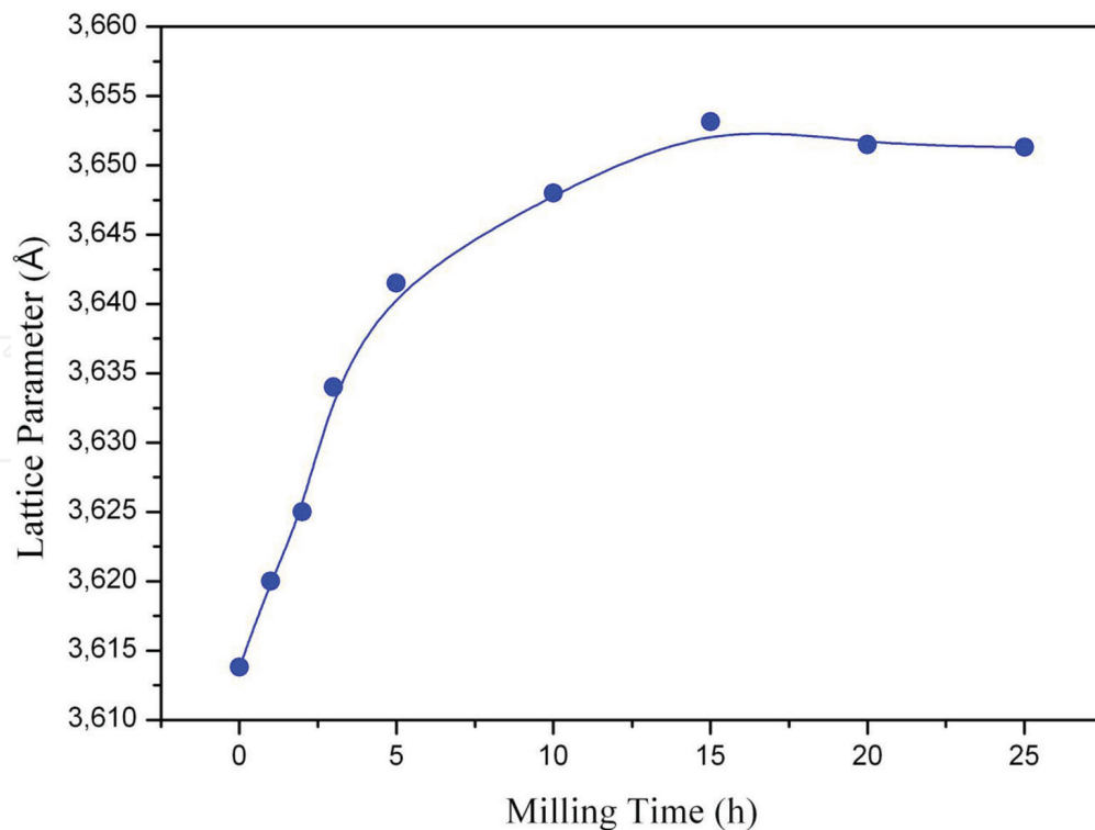
Figure 5. Lattice parameters of Cu-based FCC solid solution phase as a function of milling time. The line through the data points is a visual guide.
