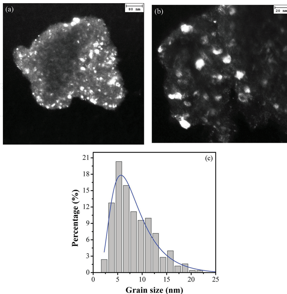
Figure 4. Dark field TEM micrographs of \text{Cu}_{50}\text{Mg}_{25}\text{Ni}_{25} powders milled for (a), (b) 25 hours, and (c) the corresponding grain size distribution with the solid line as the fit to the log-normal distribution.
