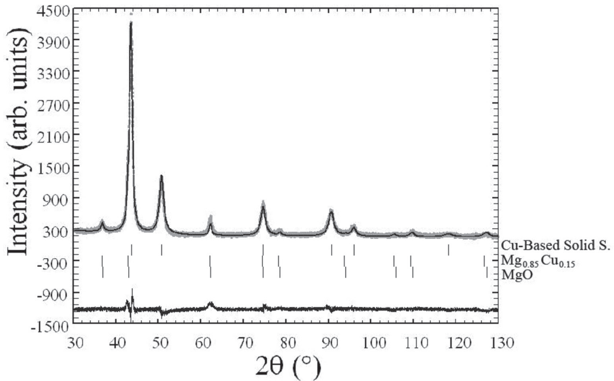
Figure 2. Rietveld refinement for XRD patterns of \text{Cu}_{50}\text{Mg}_{25}\text{Ni}_{25} powders after 25 hours of milling time.
