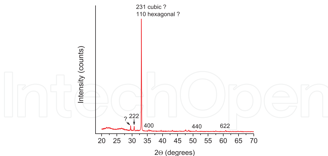
Figure 10. XRD spectra of the ITO film deposited on a Kapton substrate and annealed for 1 hour in oxygen at 300°C.
