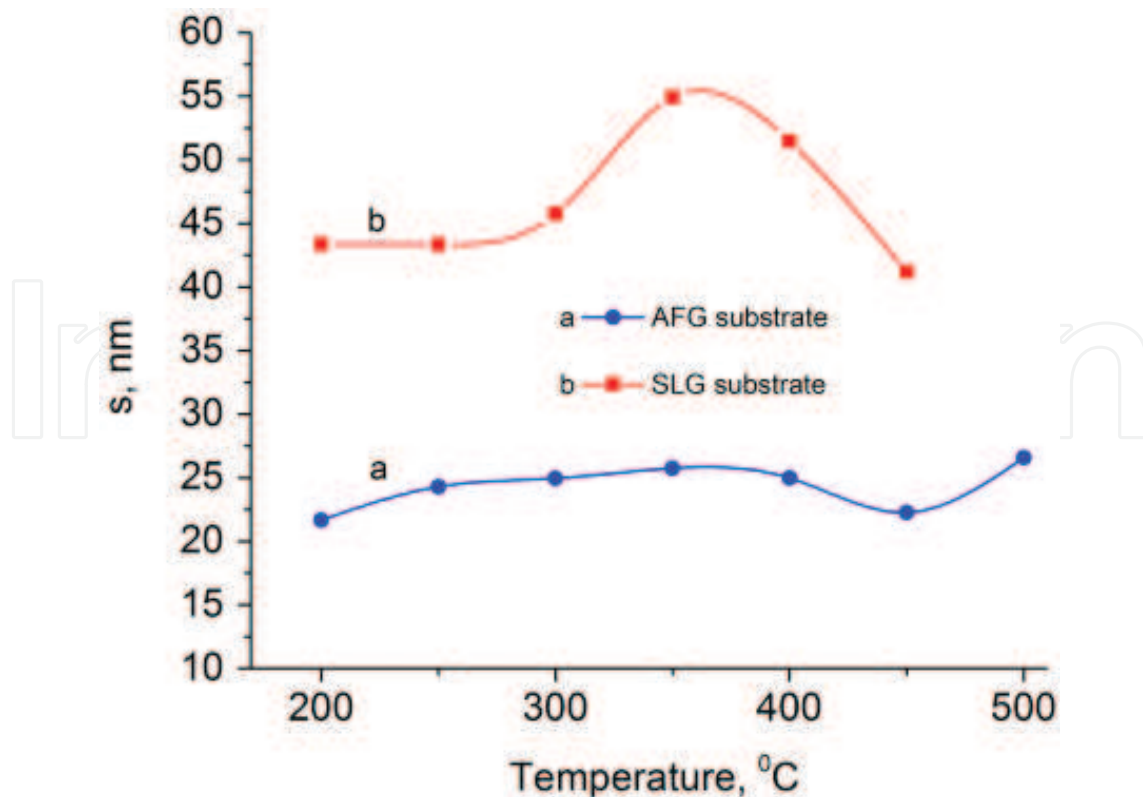
Figure 3. The average crystallite size calculated from the (222) peak.
