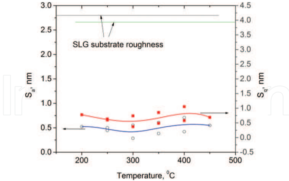
Figure 5. Average ( S_a ) and root mean square ( S_q ) roughness for the ITO film deposited on the SLG substrate and annealed in oxygen at different temperatures.
